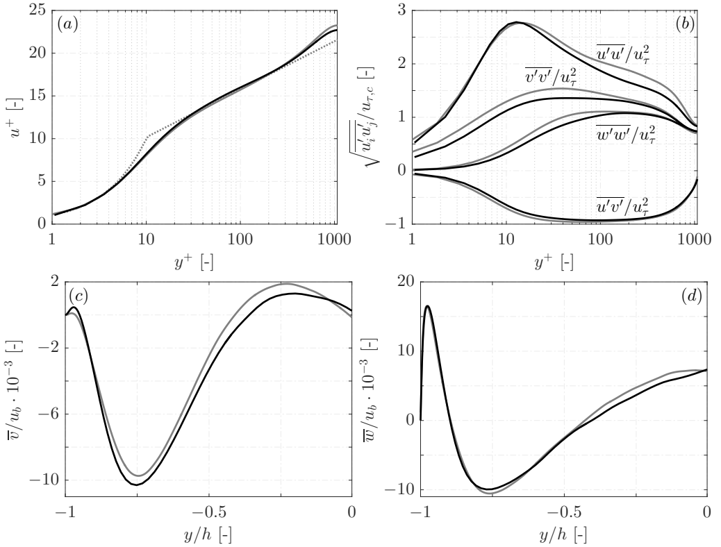
Figure 27: Profiles of (a) mean streamwise velocity and (b) Reynolds stresses along the duct midplane at z = 0 , and (c)/(d) secondary flow velocities at z = 0.75 for the LES ( — ) and DNS ( - - ) results of the adiabatic square duct. In (a) the analytical law of the wall ( u^+ = 1/0.41 \cdot \ln y^+ + 4.55 ) is represented by ( ······ ).
