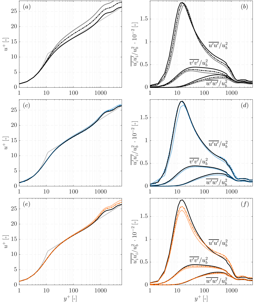
Figure 4: Grid sensitivity study with respect to (a)/(c)/(e) boundary layer velocity profile and (b)/(d)/(f) Reynolds stress distribution in the vicinity of the lower wall along the duct centre plane z = 0 . The quantities are time- and streamwise-averaged for the adiabatic domain D_{per} . Figures (a)/(b) show the influence of the maximum wall-tangential cell size using G_1 ( — ), G_2 ( - - - ) and G_3 ( ····· ), (c)/(d) the influence of the minimum cell size in wall-normal direction using G_1 ( — ), G_4 ( - - - ) and G_5 ( ····· ) and (e)/(f) the influence of the streamwise cell size using G_1 ( — ), G_6 ( - - - ) and G_7 ( ····· ). See table 2 for reference. The classical law of the wall ( u^+ = 1/0.41 \cdot \ln y^+ + 5.2 ) is represented by ( ····· ).
