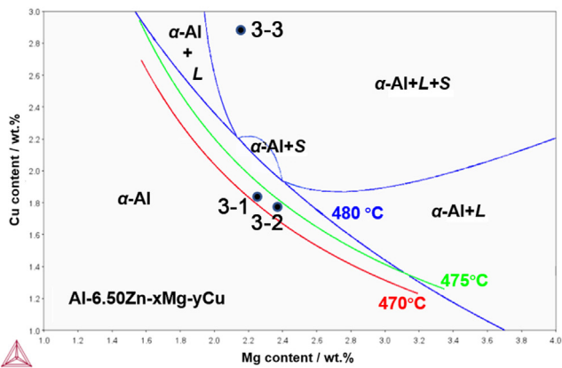
Fig. 11. Calculated isothermal sections of Al-(7.2 wt%, 6.87 wt%, 6.5 wt%)Zn-Mg-Cu system at 470 °C, 475 °C and 480 °C.
