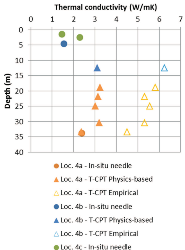
Figure 10. Thermal conductivity results at location 4.
