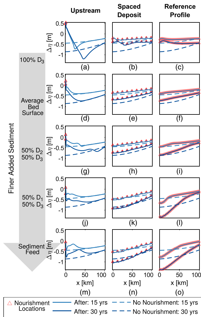
Fig. 6. Mitigation effectiveness for nourishments with sediment characterized by five grainsize distributions; nourishments (solid lines) against the base case in which no nourishments are added (dashed lines), after 15 and 30 years of model runs. Each row represents a grain-size distribution of nourished sediment (from coarsest to finest): (1) the coarse gravel (16 mm) (same as Fig. 5) (subplots a–c); (2) the bed surface prior to nourishment (d–f); (3) equal portions of fine gravel (6 mm) and coarse gravel (16 mm) (g–i); (4) equal portions of sand (1.5 mm) and coarse gravel (16 mm) (j–l); and (5) the same grainsize distribution as the sediment feed (m–o). Results are compared across three nourishment schemes: the upstream scheme, the spaced deposit scheme, and the reference profile scheme in Fig. 4.
