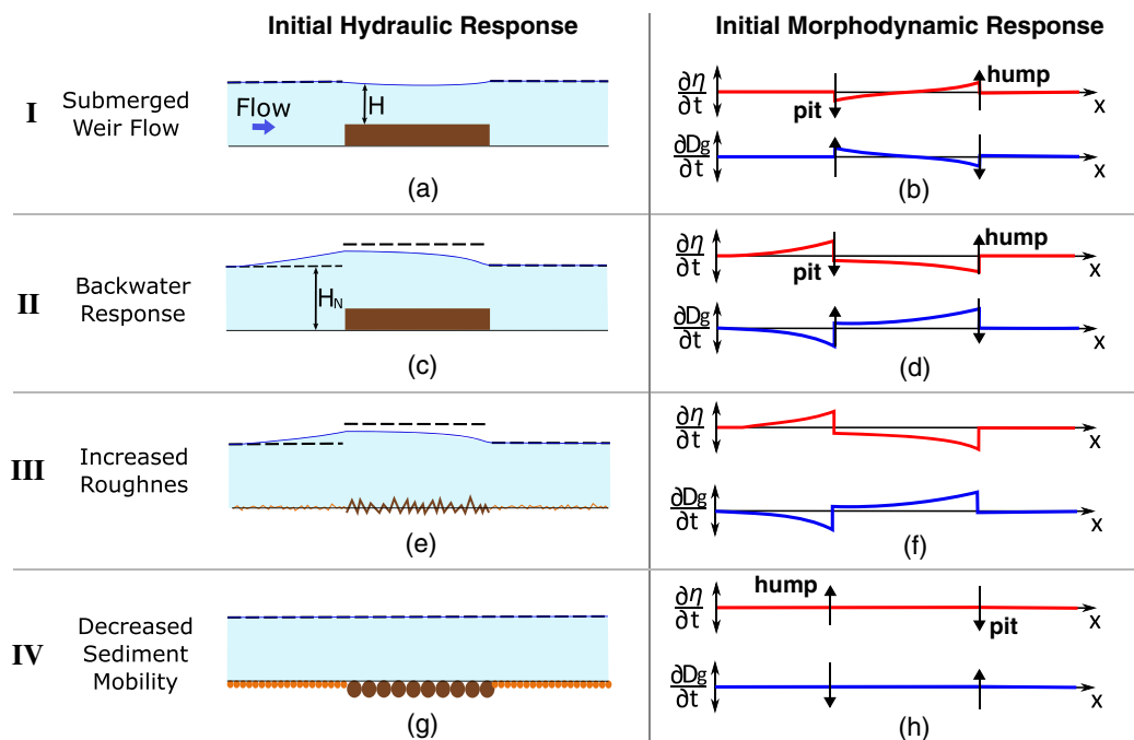
Fig. 2. (a, c, e, g) Short-term channel response regarding hydraulic change; (b, d, f, h) rate of bed level change, and rate of change of the geometric mean grain size of the bed surface sediment to a sediment nourishment. The channel response is subdivided into four relevant factors: (I) local increase in bed elevation resulting in subcritical flow over a sill (a and b); (II) local increase in bed elevation resulting in M1 backwater and M2 drawdown effects (c and d); (III) locally increased hydraulic roughness and normal flow depth due to increased bed surface grain size, and associated M1 backwater and M2 drawdown effects (e and f); and (IV) locally decreased mobility of the bed surface sediment due to increased bed surface grain size (g and h). Dashed lines in the first column indicate the water level that corresponds to the normal flow depth, while solid lines denote the actual water level.
