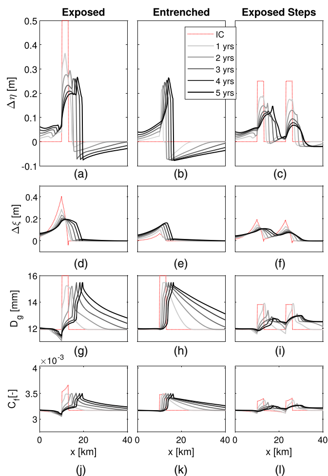
Fig. 3. Channel response to a single exposed nourishment (Column 1; subplots a, d, g, and j), entrenched nourishment (Column 2; subplots b, e, h, and k), or spaced exposed nourishments (Column 3; subplots c, f, i, and l). Nourished sediment is coarser than the bed surface sediment. Row 1 (subplots a–c) shows change in bed elevation relative to the initial state, \Delta\eta ; Row 2 (d–f) the change in water level relative to the initial condition, \Delta\xi ; Row 3 (g–i) the change in geometric mean grain size of the bed surface sediment, D_g ; and Row 4 (j–l) the dimensionless friction coefficient C_f .
