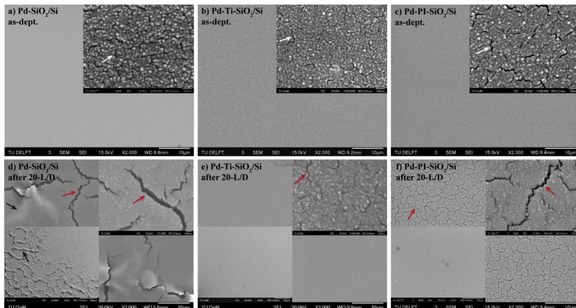
Fig. 2 – SEM images illustrating surface morphology of as-deposited and hydrogen cycled Pd thin films. From left to right: a&d) Pd-SiO 2 /Si, b&e) Pd-Ti-SiO 2 /Si and c&f) Pd-PI-SiO 2 /Si. The top layer contains as-deposited films with large images at a 10 μm scale and the inset images at a 100 nm scale. The bottom layer includes films after 20 hydrogen loading/deloading cycles (20-L/D) with large images of 10 μm scale and the inset images at 100 nm and 100 μm scales. The white arrows indicate as-deposited networks of primary microcracks associated with intercolumnar voids. The red arrows indicate hydrogen-induced microcracks, and the black arrows indicate delamination buckles or blisters in Pd-SiO 2 /Si film after 20-L/D cycles. Note that the micrographs of as-deposited films and films after 20-L/D are from two different samples. (For interpretation of the references to colour in this figure legend, the reader is referred to the Web version of this article.)
