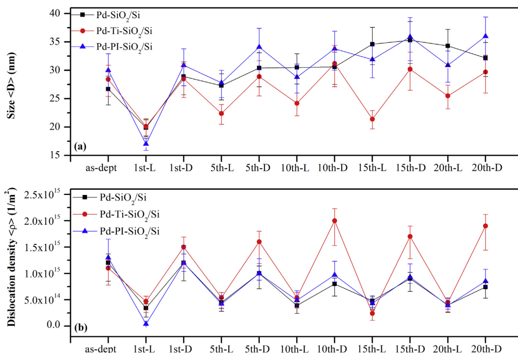
Fig. 9 – The crystallite size <D> (a) and the dislocation density \rho (b) plots to show its cyclic behavior during 20 hydrogen loading/deloading cycling (20-L/D). During loading, films are in the hydrogen-rich phase ( \beta -PdH 0.66 ) and during deloading films return to the metallic phase (Pd), as in the as-deposited state.
