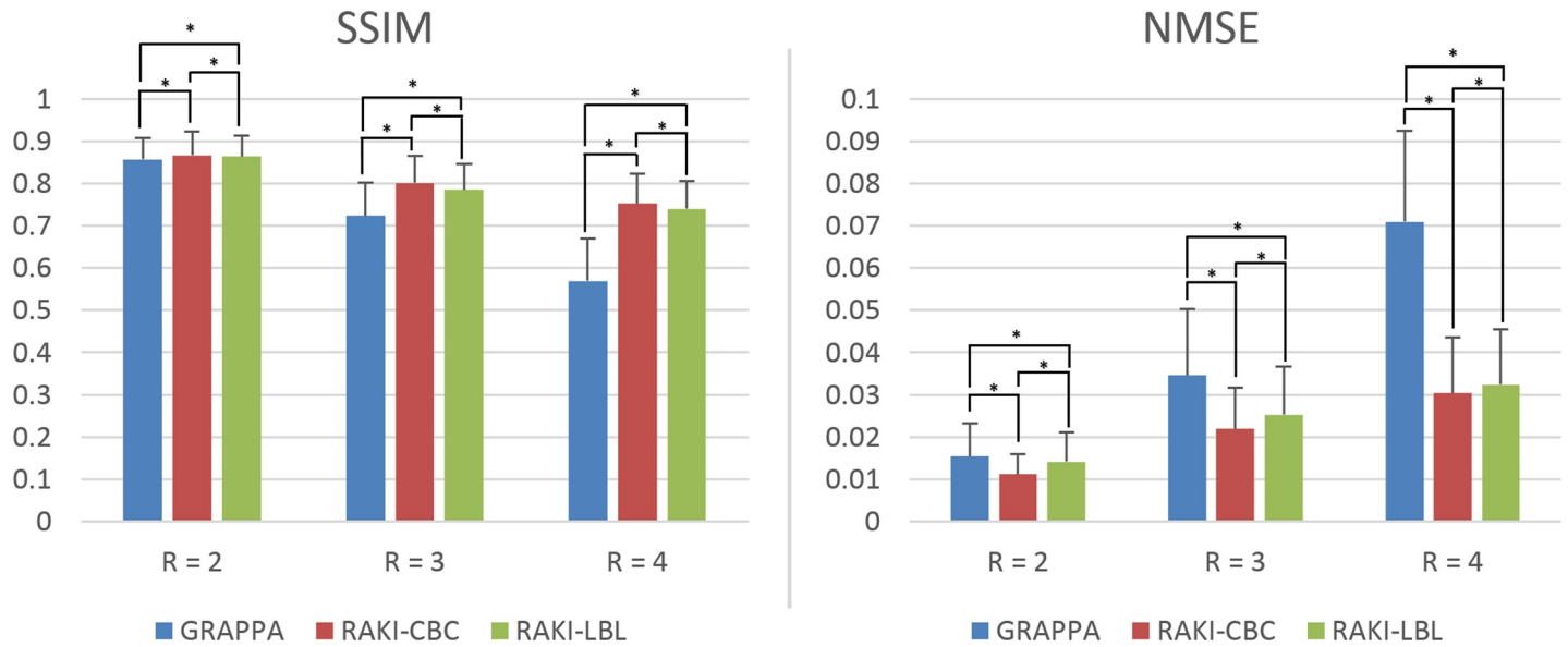
Fig 5. Mean structural similarity index (SSIM) and normalized mean squared error (NMSE) for different methods. SSIM and NMSE of GRAPPA, RAKI-CBC and RAKI-LBL for 190 proton density weighted knee data with fat suppression from the fastMRI dataset [23]. Error bars represent standard deviation across datasets. SSIM results showing both RAKI-CBC and RAKI-LBL offers better image quality than GRAPPA, with 24.0% improvement at R = 4 . Similar observations apply to NMSE. All differences between methods and across rates were statistically significant ( P < 0.05 ), which are marked with *.
