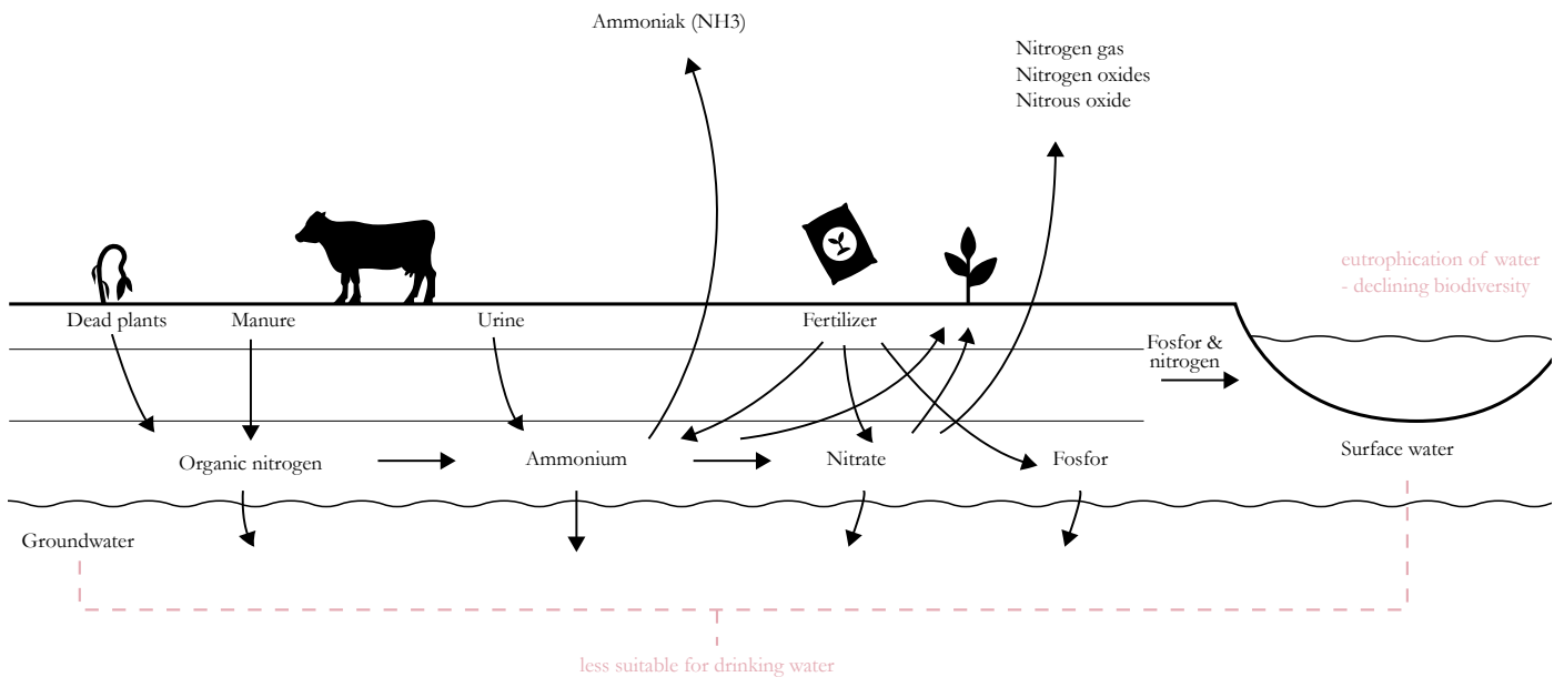
Processes in the ground resulting from manure and fertilizers. Source: RIVM, 2020. Image: Hanneke Wander, 2022.
