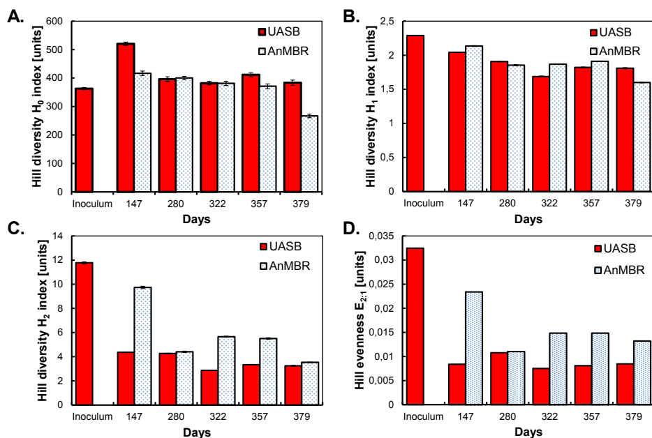
Figure 5.8 Alpha diversity of UASB and AnMBR. A. H_0 (richness, number of OTUs). B. H_1 (exponential value of the Shannon index). C. H_2 (inverse Simpson index). D. E_{2:1} (species evenness) were calculated both for bacteria and archaea.
