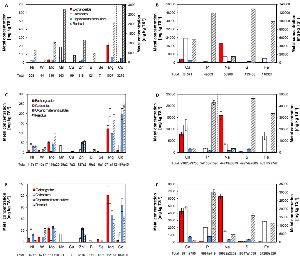
Figure 2.6 Trace and macro elements concentration [mg·kgTS -1 ], and partitioning in the operationally defined fractions after one month of operation. A, B. Inoculum biomass. C, D. AnMBR1. E, F. AnMBR2. After the dashed line the concentration must be read from the secondary y-axis.
