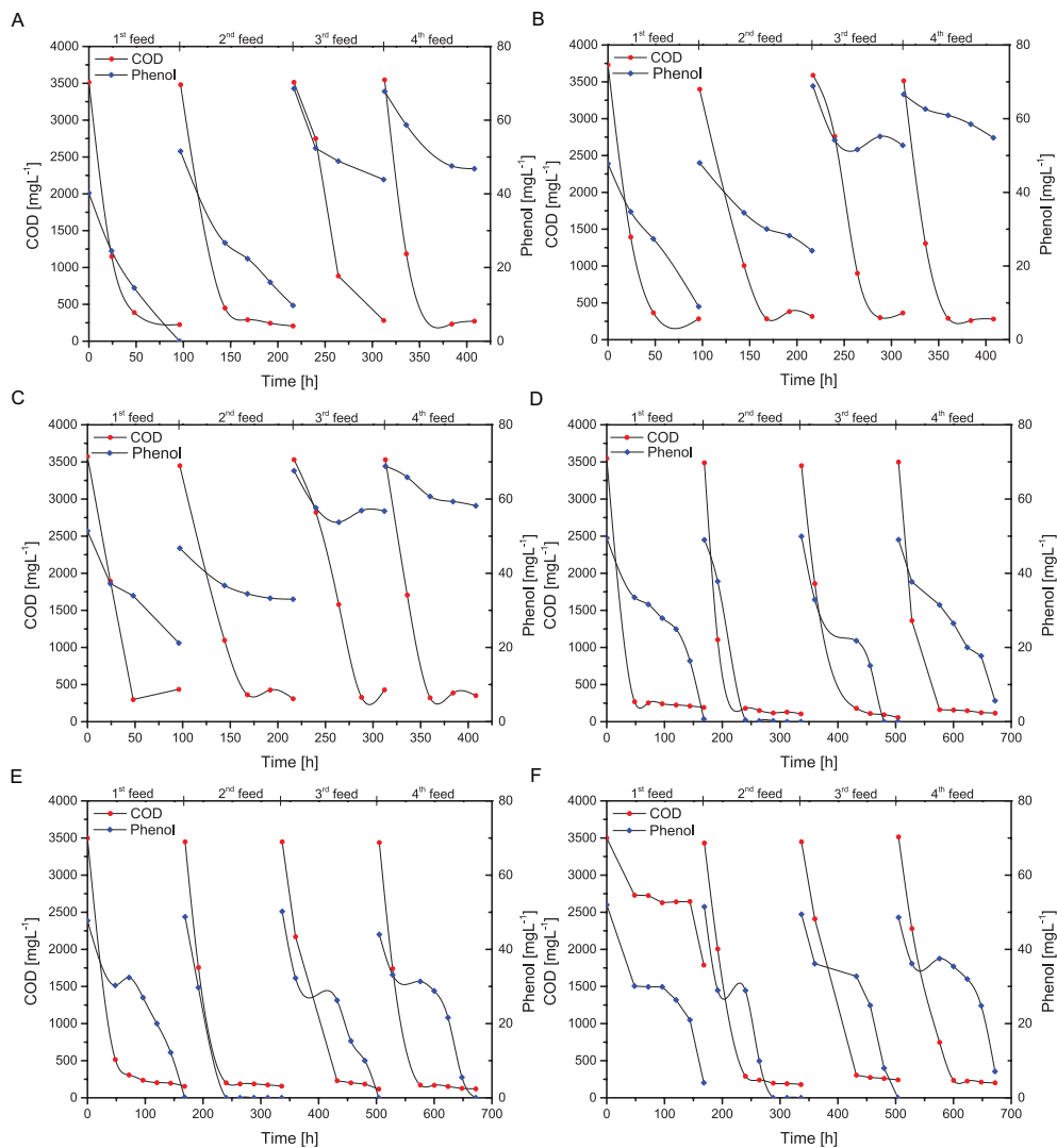
Figure 3.4 Batch test assessment of impact of K^+:Na^+ ratio on COD and Phenol degradation. Constant K^+:Na^+ ratio of 0.05 A. 16 gNa^+L^{-1} (0.05) B. 20 gNa^+L^{-1} (0.05) and C. 24 gNa^+L^{-1} (0.05). Varying K^+:Na^+ ratio D. 16 gNa^+L^{-1} (0.03). E. 20 gNa^+L^{-1} (0.025) and F. 24 gNa^+L^{-1} (0.02).
