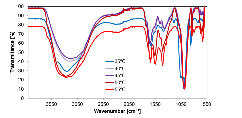
Figure S6.2. FT-IR spectra of the EPS extracted from the AnMBR.
