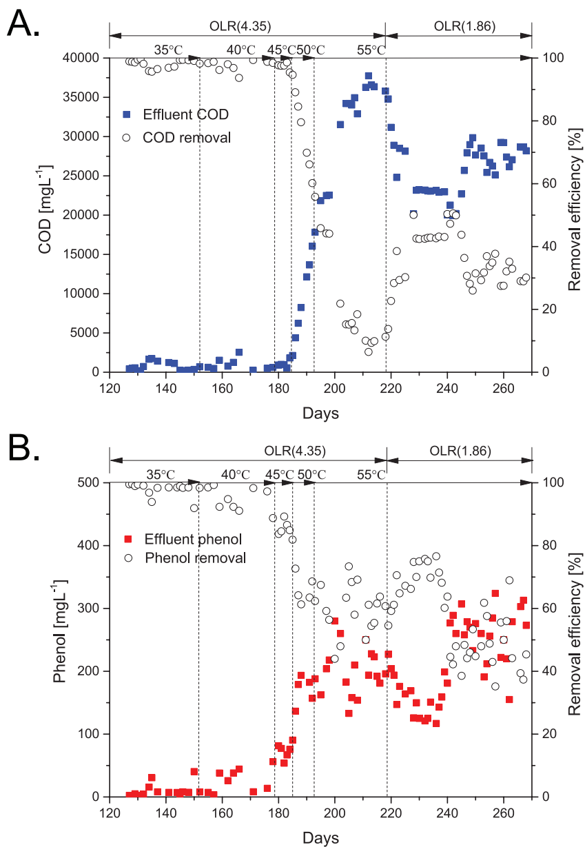
Figure 6.1 AnMBR performance under mesophilic, hyper-mesophilic and thermophilic conditions at 16 \text{ gNa}^+ \cdot \text{L}^{-1} . A. COD removal efficiency. B. Phenol removal efficiency.
