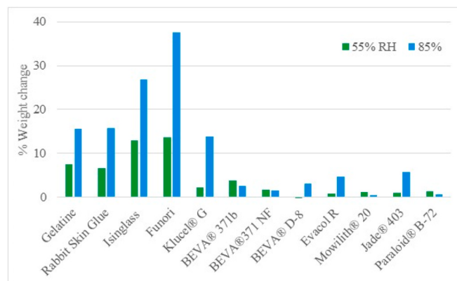
Fig. 2. The percentage of weight change due to moisture uptake, referenced to 6% RH, 25^\circ\text{C} .
