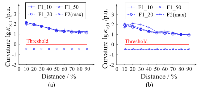
Fig. 15. Results of different sampling frequencies. (a) P-PTG; (b) PTP.
