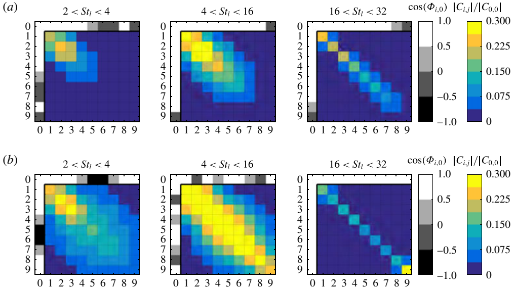
FIGURE 11. (Colour online) Phase information with respect to the overall segment (grey scale) and normalized cross-spectral-density matrix (colour scale) for the various strips (figure 10a) for the (a) sawtooth and (b) combed-sawtooth serrations.
