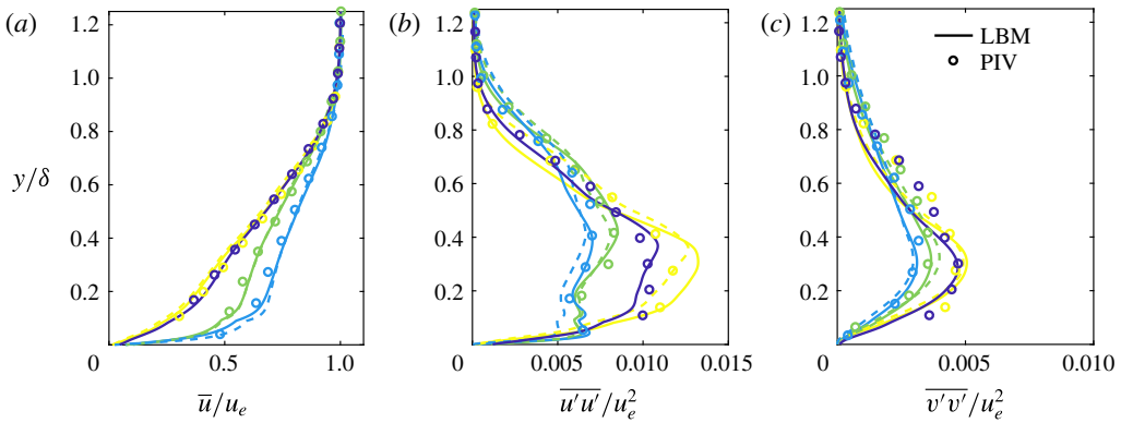
FIGURE 3. (Colour online) (a) Time-averaged, root-mean-square of the (b) streamwise and of (c) the wall-normal velocity components. Profiles at different locations along the edge for the straight and sawtooth configurations. Experimental PIV data for the serrated case (circles) are extracted from Arce-León et al. (2016b). The locations along the serration, indicated in the legend, are: (yellow) x/2h=0 , (green) x/2h=0.5 and (light blue) x/2h=1 ; the boundary layer for the straight trailing edge is reported in purple.
