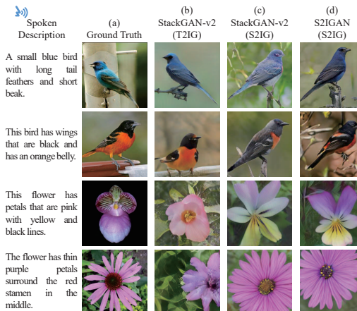
Figure 2: Examples of images generated by different methods.
