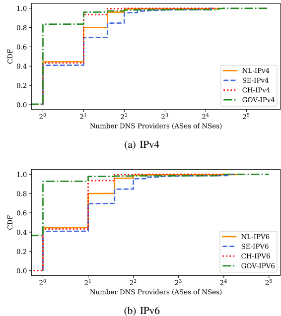
Fig. 5. Number of ASes (DNS providers) for e-gov domains
