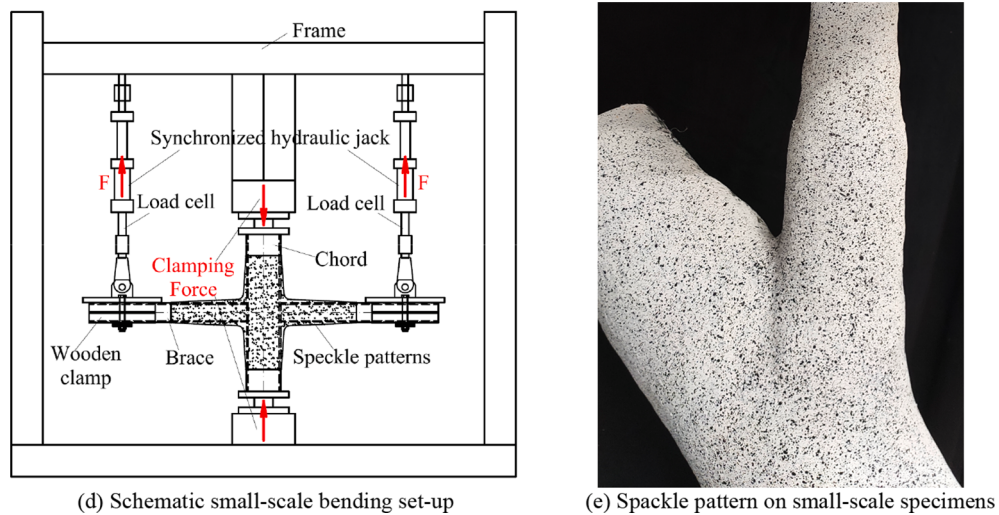
Fig. 6. The 3D DIC system with live measurement of displacements and strains on the surface of specimen at two scales.
