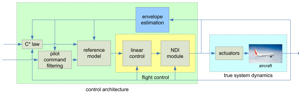
Figure 2. Global overview of manual control structure
