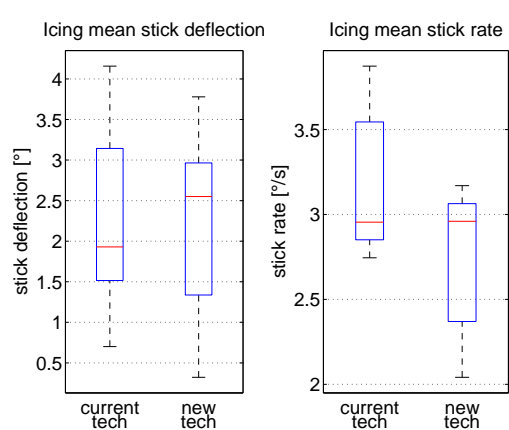
Figure 27. Statistical analysis of pilot activity for icing scenario, all crews
