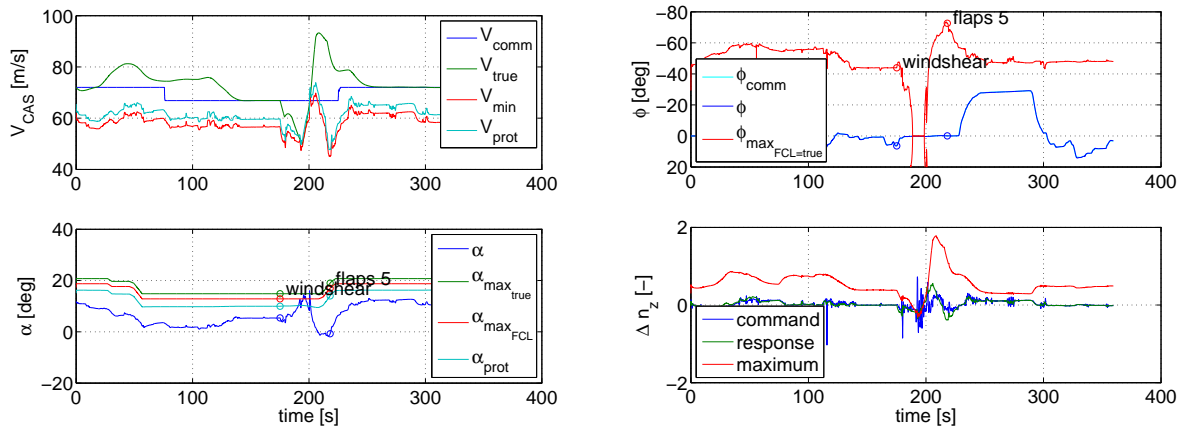
(a) time histories of calibrated airspeed V_{\text{CAS}} and angle of attack \alpha
