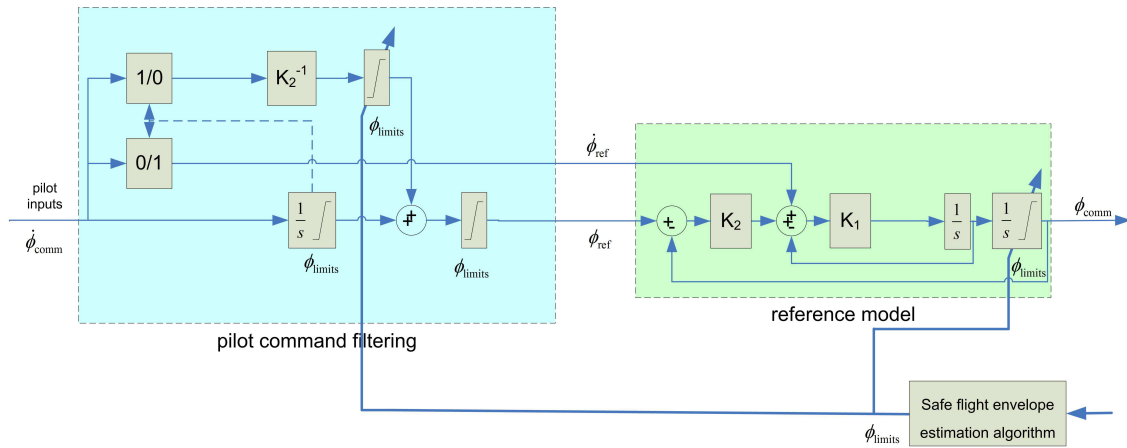
Figure 7. Directional control law setup (pilot command and reference model) with adaptive envelope limits
