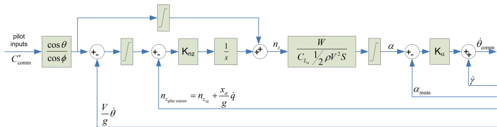
Figure 5. Control setup of the C^*/n_z control law, modified from Ref. [10]
