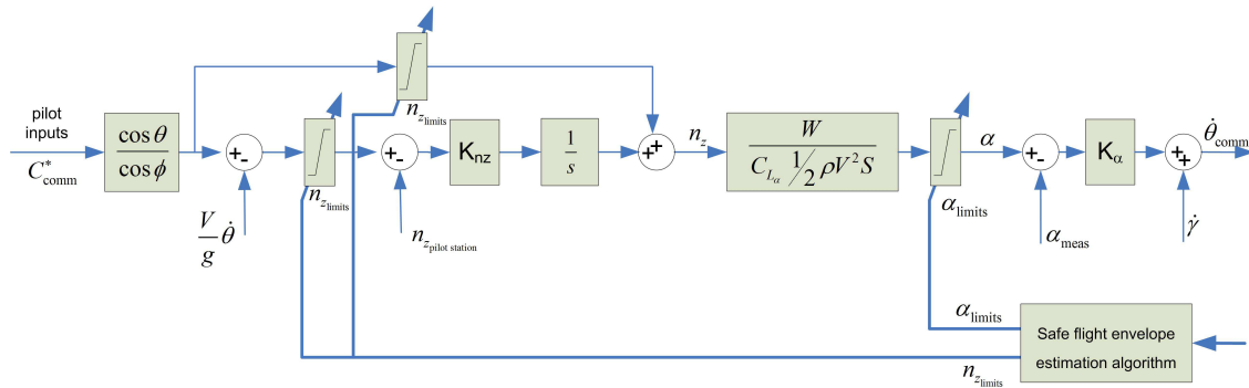
Figure 6. Longitudinal control law setup with adaptive envelope limits
