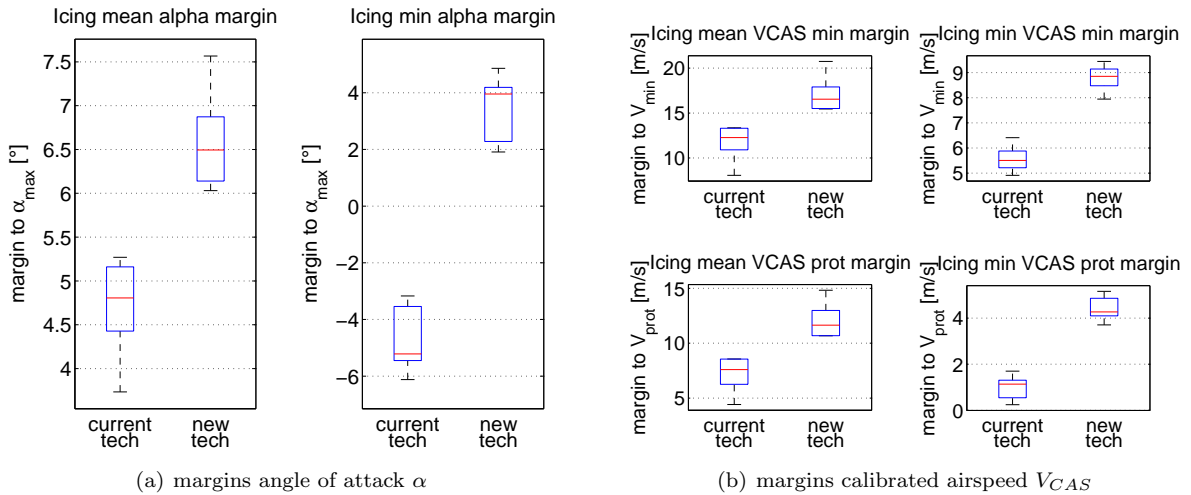
Figure 25. Statistical analysis of angle of attack and speed margins to envelope boundaries for icing scenario, all pilots
