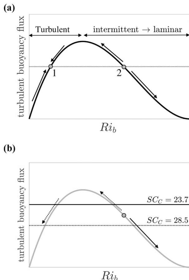
FIG. 5. Sketches of the steady-state relation between the turbulent buoyancy flux and the bulk Richardson number. Similar sketches were presented by van Hooijdonk et al. (2015) and Ansgore (2017). The shape of the curve to the right of the maxima is highly uncertain, since the flow is not horizontally homogeneous in this regime. (a) Sketch of the flow character at different stages. The black-circled dots represent conceptual equilibrium states for a specific (absolute value of) imposed wall flux (dashed line). (b) Sketch of the hypothesized evolution for two different imposed wall fluxes (represented by black horizontal lines) when the flow is initialized from a strongly stratified state (black-circled dot). The arrows indicate the hypothesized evolution for the two cases described in the main text: i.e., collapsing (solid) and recovering (dotted).
