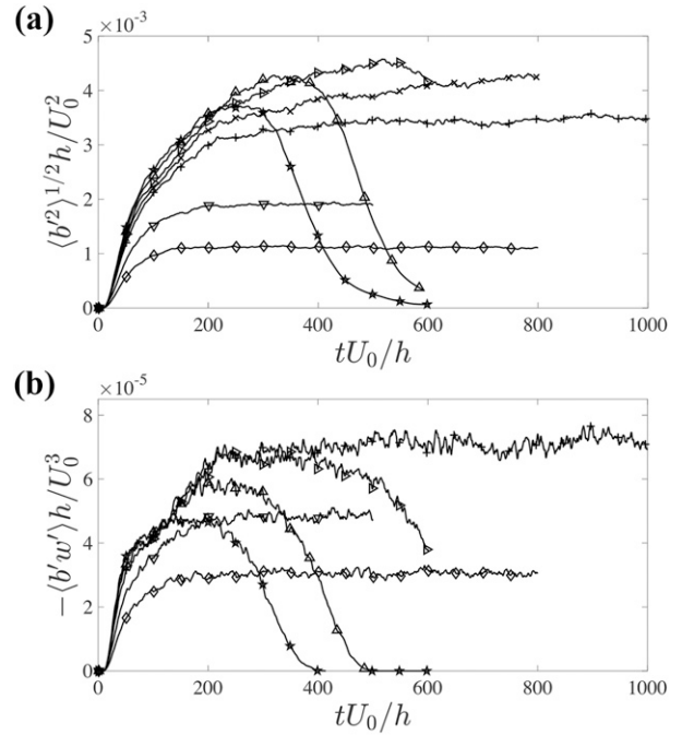
FIG. 3. Time series of (a) the buoyancy fluctuations and (b) the turbulent buoyancy flux at z = h for all SC_C at Re = 3500 . Symbols are as in Fig. 1.
