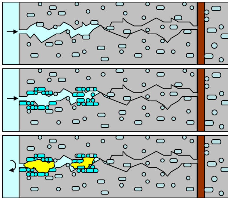
Figure 1: Scenario of crack-healing by concrete-immobilized bacteria (after [1]). Ingress water activates bacteria on fresh crack surfaces, bacteria multiply and precipitate calcium carbonate, eventually sealing and plugging the crack, protecting embedded steel reinforcement from further external attack.
