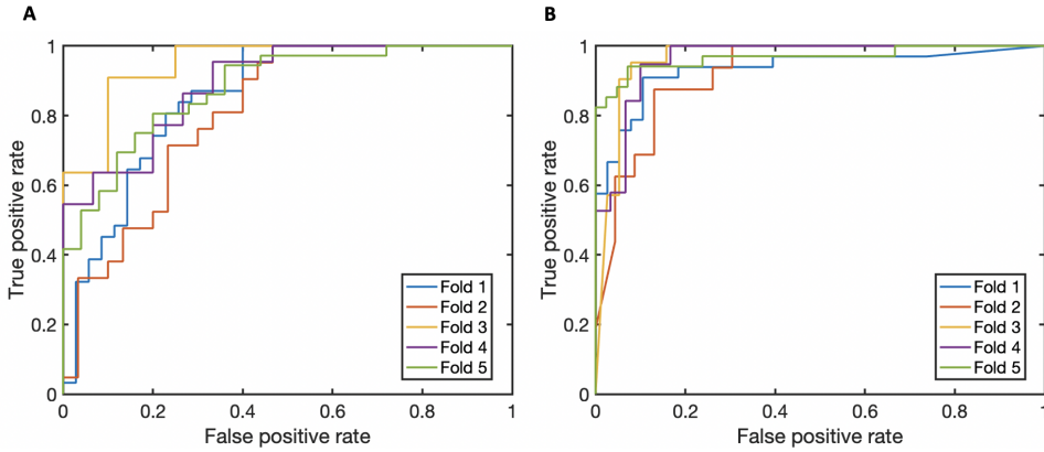
Figure 4.13: Receiver operating characteristic (ROC) curve on the testing dataset, A) SVM, B) RF.
