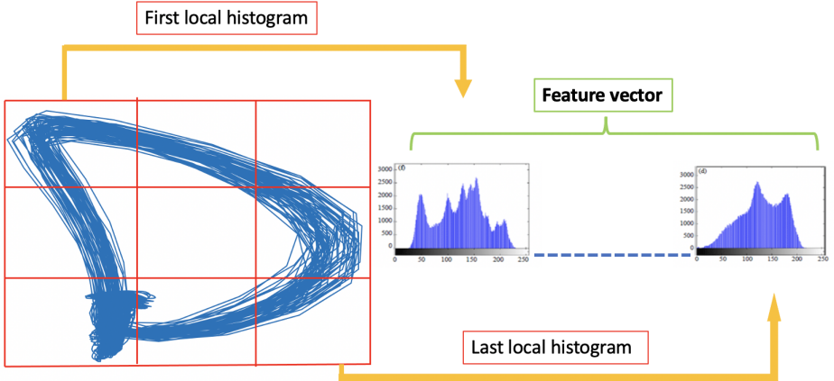
Figure 4.8: The URILBP feature vector of an image consists of a concatenation of the histogram of URILBP scores of each sub-image
