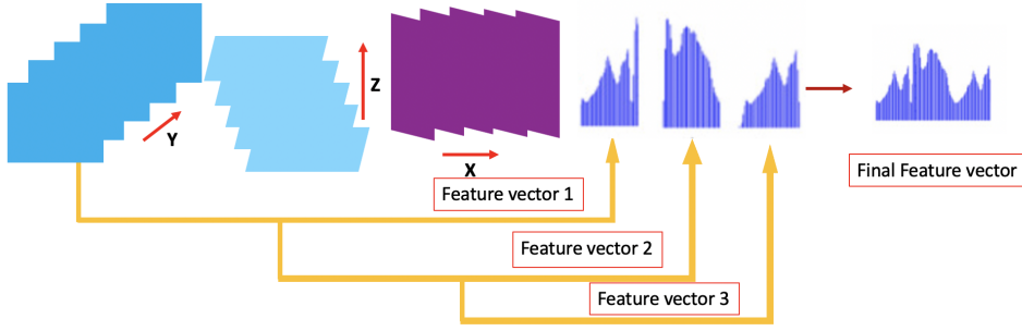
Figure 4.9: 3DLBP feature vector .
