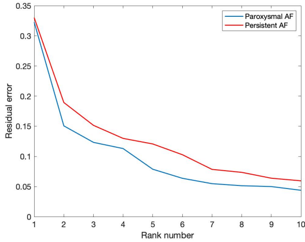
Figure 3.3: Relative error of tensor decomposition by reconstructing the tensor by varying r between 1 and 10
