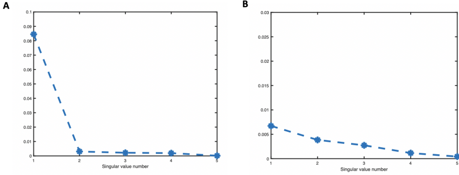
Figure 4.4: Singular values of matrix H : A) de novo POAF, B) persistent AF
