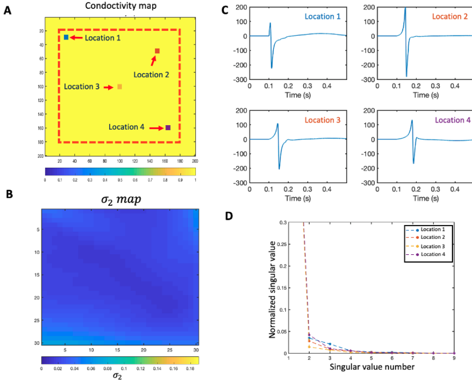
Figure 5.3: \sigma_2 map analysis of a homogeneous tissue
