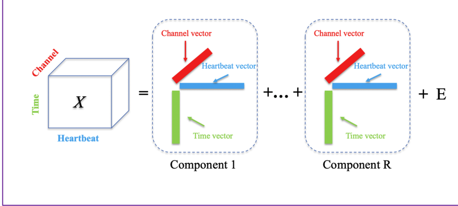
Figure 3.2: Tensor construction and CPD decomposition
