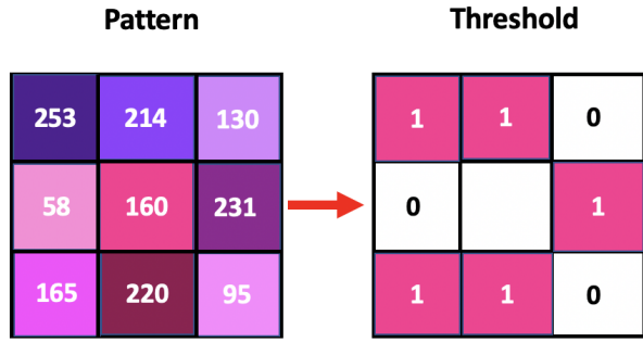
Figure 4.6: LBP operator
