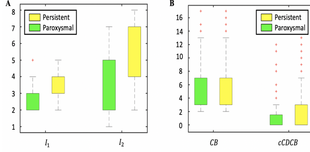
Figure 7.2: Box plots of the features, A) proposed features, B) state-of-the-art features.
