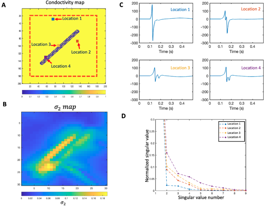
Figure 5.4: \sigma_2 map analysis of a tissue with a diagonal line of block.
