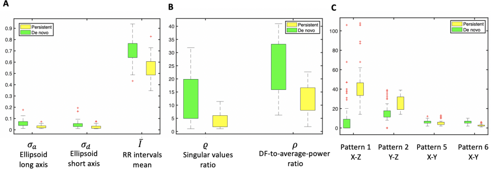
Figure 4.12: Box plots of the selected features, A) Rhythm-based features ( \sigma_a : ellipsoid long axis, \sigma_d : ellipsoid short axis and \tilde{I} : RR intervals mean), B) Ratios ( \rho : singular values ratio Eq. (4.6), \rho : DF-to-average-power ratio Eq. (4.8)), C) VCG-based features .
