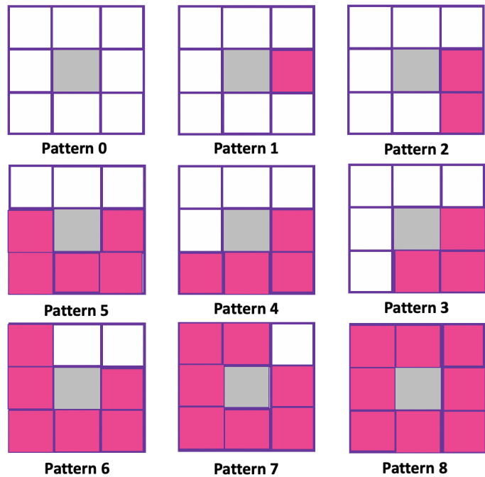
Figure 4.7: URILBP: There are in total 9 possible uniform rotationally invariant local binary patterns.
