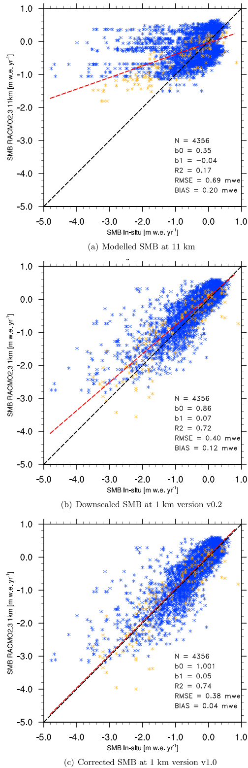
Figure 3. Comparison of SMB observations collected at 237 sites with (a) modeled SMB from RACMO2.3 at 11 km, (b) downscaled SMB at 1 km (v0.2), and (c) corrected downscaled SMB at 1 km (v1.0). The orange symbols correspond to in situ measurements from Penny ice cap (39 sites, SCAA). The red dashed lines represent the regression including all measurements (NCAA and SCAA) using a perpendicular fit. SMB = surface mass balance; RACMO2.3 = Regional Atmospheric Climate Model version 2.3; SCAA = Southern Canadian Arctic Archipelago; NCAA = Northern Canadian Arctic Archipelago.
