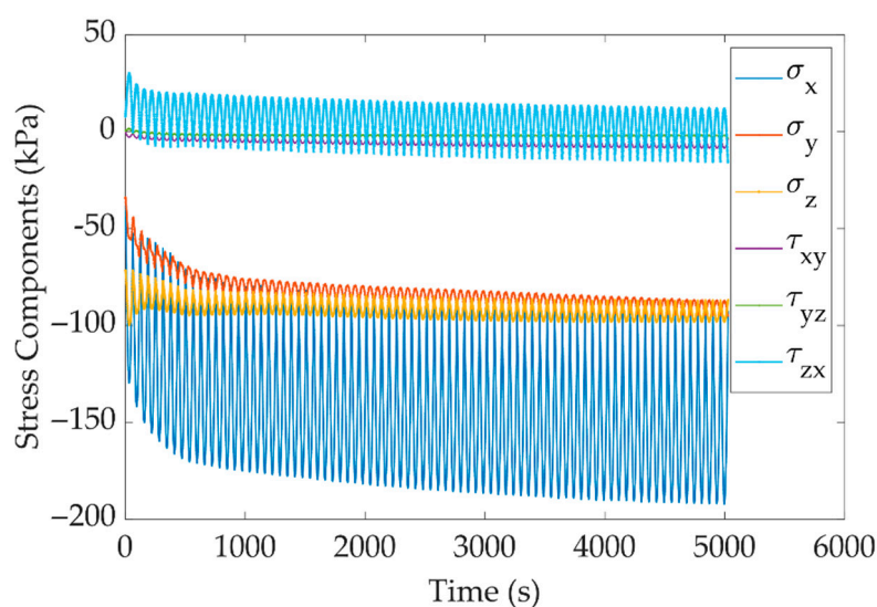
Figure 3. Variation of stress components during applied cyclic loading for element E1.
