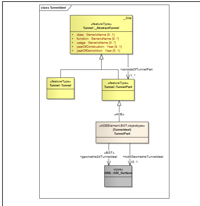
Figure 1: TunnelPart AD Element with 2D geometry
