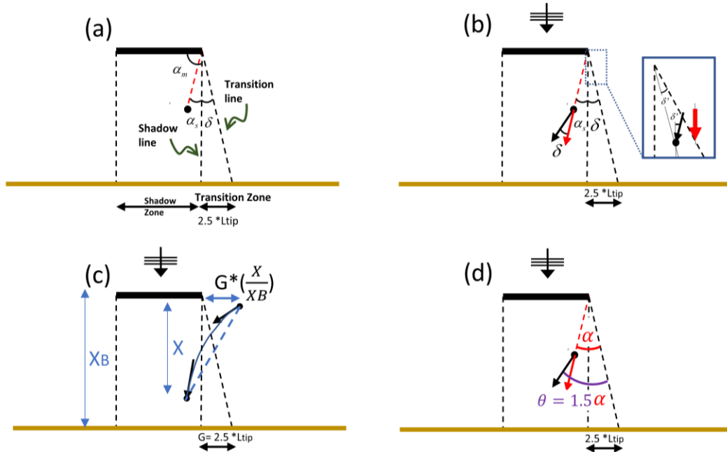
Figure 1. Definition sketch of (a) the parameters used in this study, (b) the new approach for the angle treatment behind the breakwater, (c) Dabees approach, and (d) modified Hurst approach.
