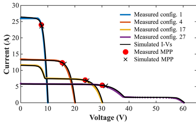
Fig. 10. Measured and simulated I–V curves of configurations 1, 4, 17, and 27 in shading experiment A.
