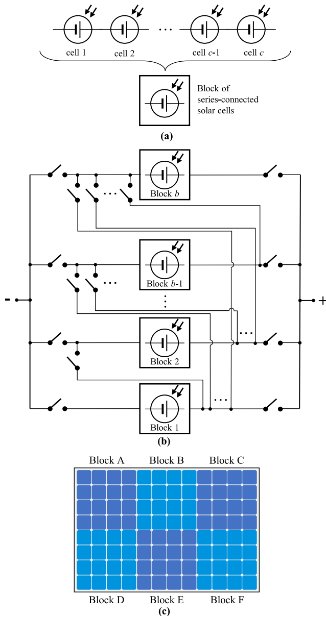
Fig. 1. Reconfigurable series-parallel PV module. (a) One block of c solar cells connected in series. (b) Generic diagram of a fully reconfigurable series-parallel PV module with b blocks. (c) Layout of the studied reconfigurable module. The module is organised in 6 blocks ( b = 6 ), indicated in different shades of blue) of 4 by 4 solar cells connected in series. The positive and negative terminals of each block are connected to the inputs of the switching matrix.
