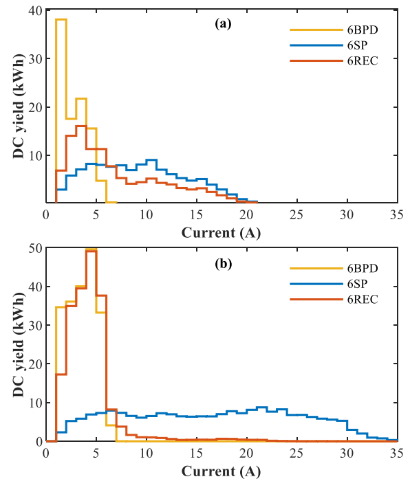
Fig. 6. DC current distribution of the analysed module topologies in Utrecht. (a) Histogram of the DC energy generated by the analysed module topologies as a function of the module's output current for the most shaded position (1) on the rooftop. (b) Histogram of the DC energy generated by the analysed module topologies as a function of the module's output current for the least shaded position (3) on the rooftop. It is assumed that the 6BPD module is always operated at the true MPP and that the switching matrix of the 6REC module is controlled by the proposed algorithm.
