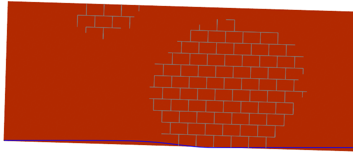
Figure 15: Deformed mesh and active joints (in grey) at end-settlement of 6 mm. 20\times displacement magnification.
