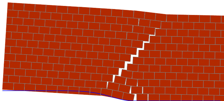
Figure 17: Deformed mesh at end-settlement of 12 mm for a model with all joints a priori active. 20\times displacement magnification.
