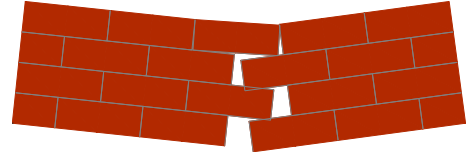
Figure 6: Deformed mesh at a CMOD value of 2 mm for a model with all joints a priori active. 40× displacement magnification.
