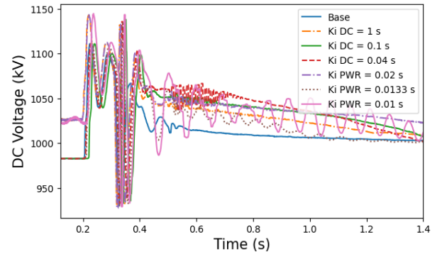
Fig. 11. DC voltage response for different integral gains
