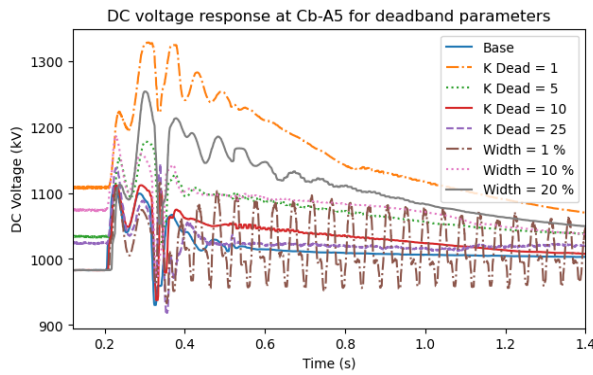
Fig. 12. DC voltage response for different dead-band parameters
