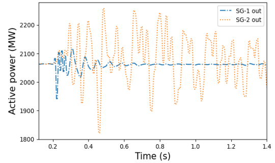
Fig. 4. Active power flow in line 1-5 for different outages
