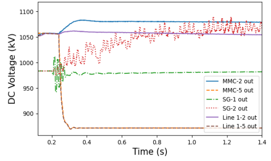
Fig. 2. DC voltage response at bus 5 for different outages
