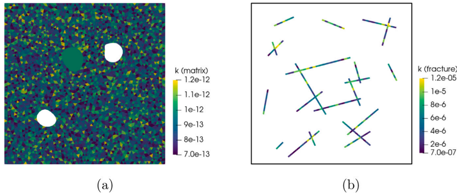
Fig. 16. Permeability distribution (unit: [m²]) of the rock matrix (a) and fractures (b) with high-conductivity.
