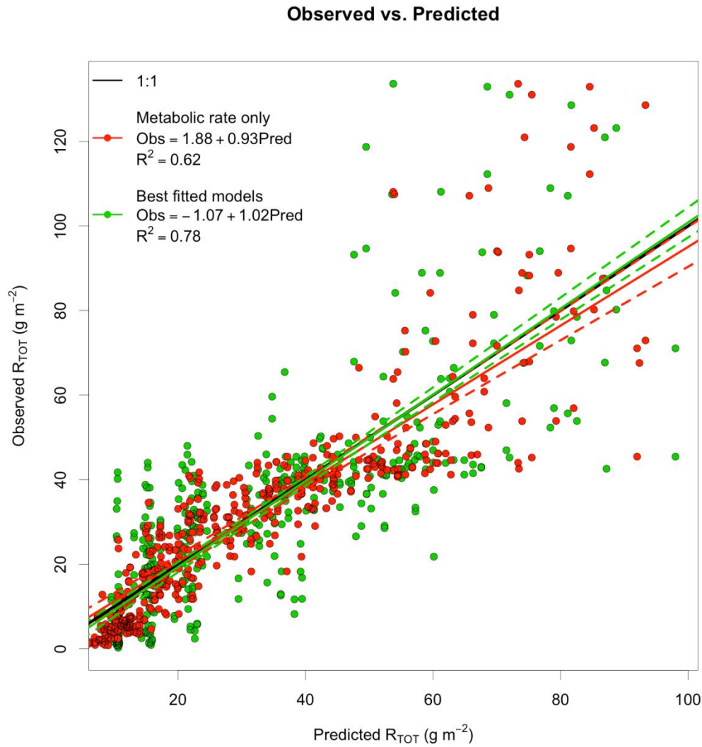
Figure 3. Relationship between observed sediment resuspension in our experiments ( R_{TOT} g m -2 ) and predictions from Equation 5: R_{TOT} \sim a_{BIO}/1 + e^{[(b_{BIO} - BSS)/c]} . The black full line show the 1:1 ratio. Full coloured lines show the average trend; dashed lines show the 95% Confidence Interval around the average trend. The red points and lines show the prediction of Equation 5 using the metabolic rate of the bioturbations population as only descriptor for variations in a_{BIO} and b_{BIO} . The green points and lines show the prediction of Equation 5 including also the negative dependence of a_{BIO} from the individual size and allowing interspecific variations in b_{BIO} (Table 5).
