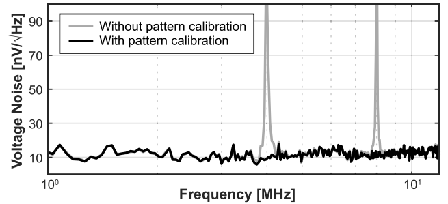
Fig. 20. Input-referred spectral voltage noise density with and without calibration of the static mismatch pattern of the subarray beamformer.
