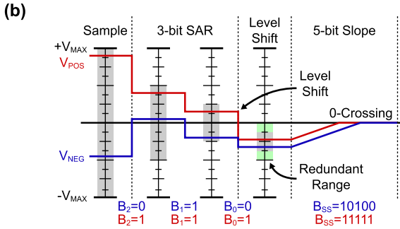
Fig. 10. (a) Overview of SAR DAC with unit cell details. (b) Exemplary conversion diagram showing the residual on sampling capacitors.
