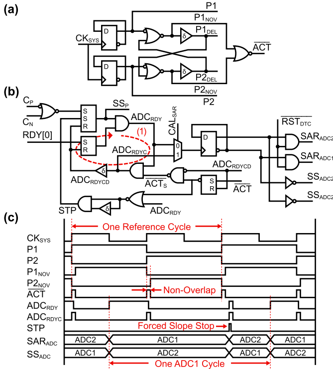
Fig. 6. (a) Synchronous timing generator of the shared converter. (b) Loop determining asynchronous ADC timing. (c) Conceptual timing diagram.
