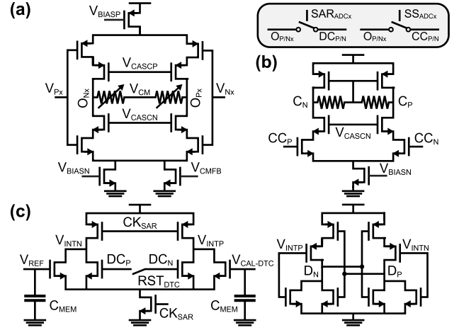
Fig. 8. (a) Schematic of the preamplifier with switches to second stages. (b) Schematic of the continuous-time comparator. (c) Schematic of the DTC.
