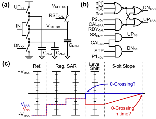
Fig. 12. Conceptual diagram of (a) calibration charge pumps, (b) related SAR and SS controls, and (c) calibration switching overview.
