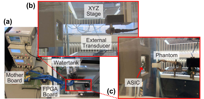
Fig. 19. (a) Overview of the acoustic measurement setup. (b) Inset showing watertank with external transducer. (c) Imaging experiment details.
