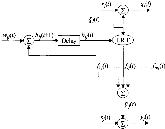
Figure 2.3: Causal dependencies in the motorway model. According to the model, the idealized entry flows \tilde{q}_i(t) are distributed over the EE flows f_{ij}(t) in a series of Independent Random Trials (IRT), using the split probabilities b_{ij}(t) .
