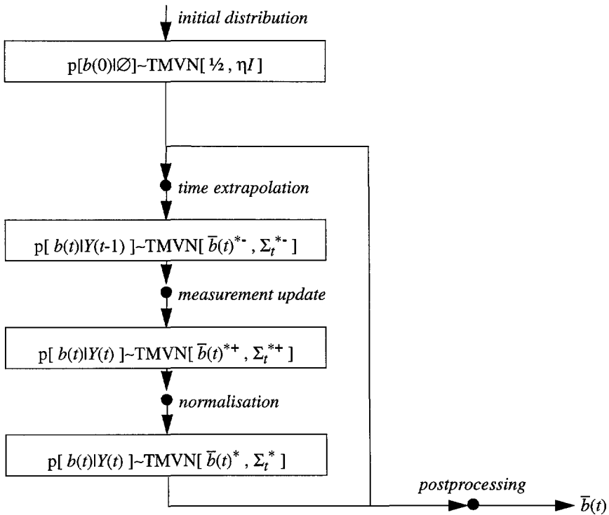
Figure 4.4: Structure of bayesian estimator for split probabilities, including initialization, time extrapolation, measurement update, normalization and postprocessing.
