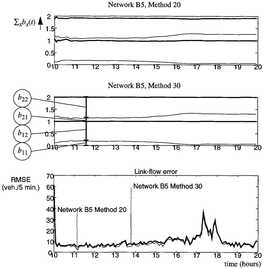
Figure 9.6: (Above) Stacked plot of the estimated split probabilities as a function of time of day for network B5 and methods 20 and 30. The lines in these plots represent (from below to above): b_{11} , b_{11}+b_{12} , b_{11}+b_{12}+b_{21} , b_{11}+b_{12}+b_{21}+b_{22} (Below) RMSE link-flow error, plotted for network B5 and methods 20 and 30. Method 20 systematically underestimates the split probabilities, but despite these bias, results in lower link flow errors
