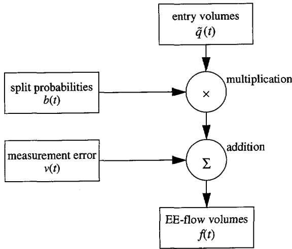
Figure 5.1: Destination choice modelled by deterministic selection, followed by addition of a measurement error.
