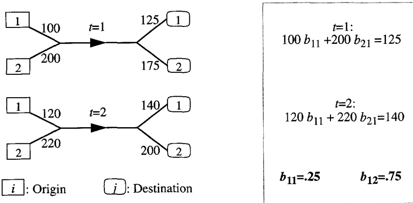
Figure 1.3: Application of the split ratio principle: assuming the split proportions are constant during two periods, results in two independent linear equations with two unknowns; from these equations the split proportions can be solved.
