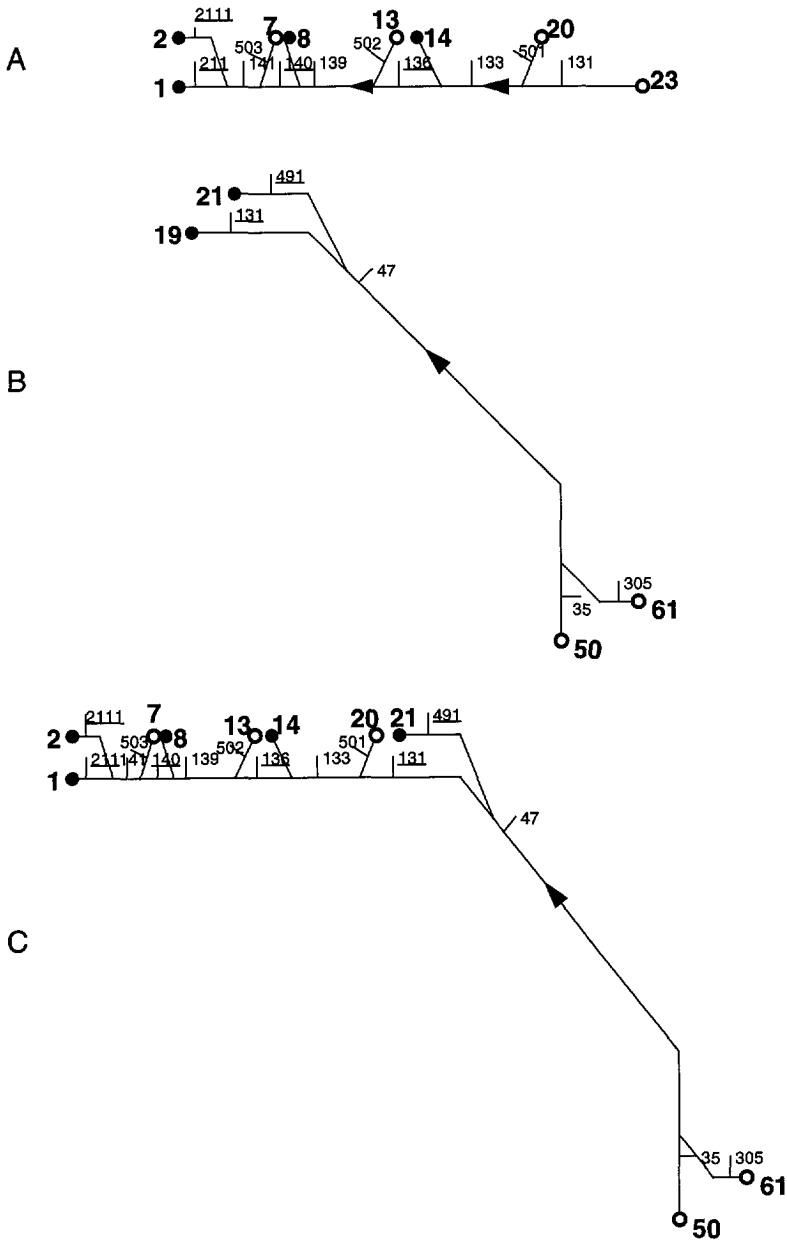
Figure 9.4: Network variants A, B and C. The bold numbers are node numbers. Closed circles are origins. Open circles are destinations. The small numbers indicate the locations of the induction loops. The underlined numbers indicate the induction loops that were used as a reference location.
