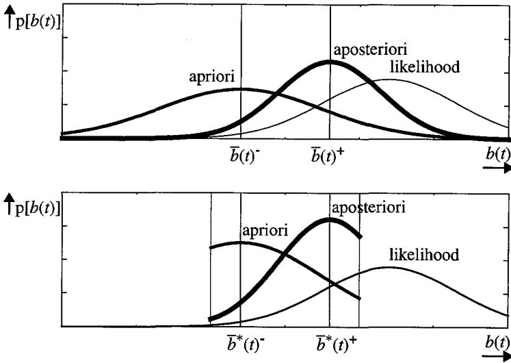
Figure 4.2: Bayesian update: \text{aposteriori} = \text{likelihood} \cdot \text{apriori} / \text{normalising constant} . Top graph: prior distribution is MVN. Bottom graph: prior distribution is TMVN.
