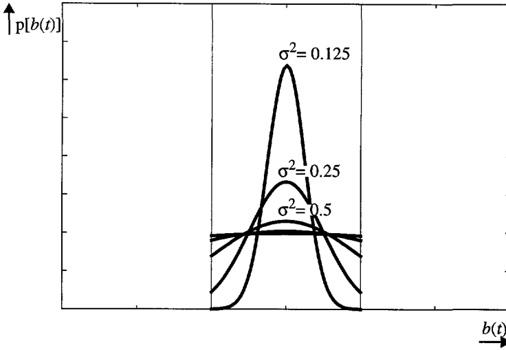
Figure 4.3: Truncated normal distributions approach the uniform distribution if variance increases
