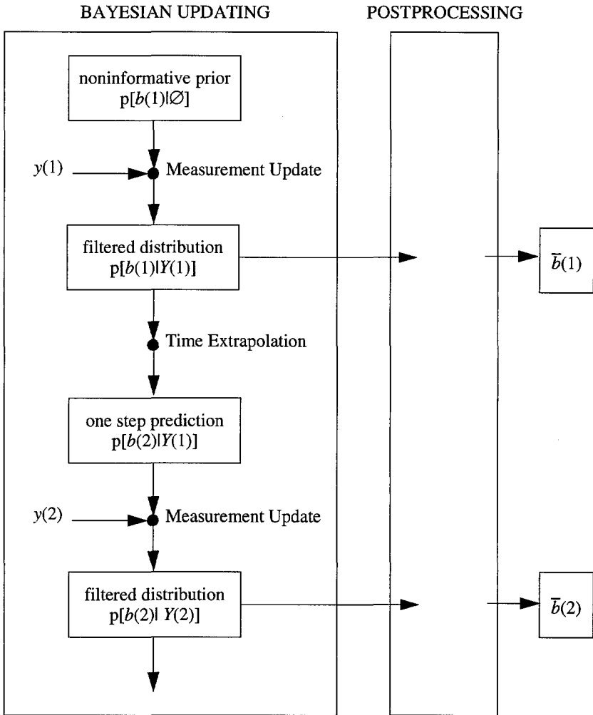
Figure 4.1: Bayesian updating scheme. The procedure is initiated with a noninformative prior. Via a sequence of measurement updates and time extrapolations the probability distribution of the state is traced. Postprocessing is needed to make practical use of this distribution.
