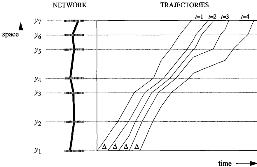
Figure 1.2: Moving time coordinate system. The time space trajectories divide the consecutive periods.
