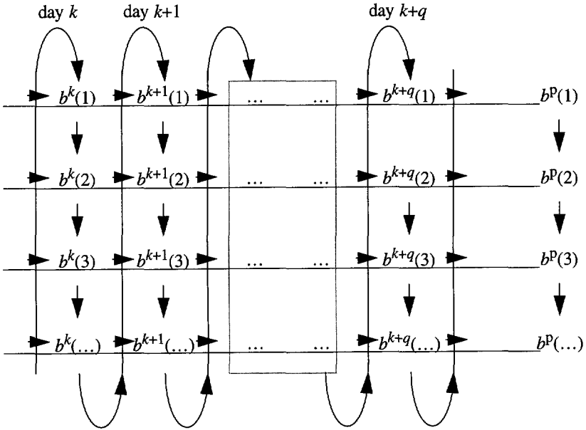
Figure 6.3: Vertical and horizontal random walk model
