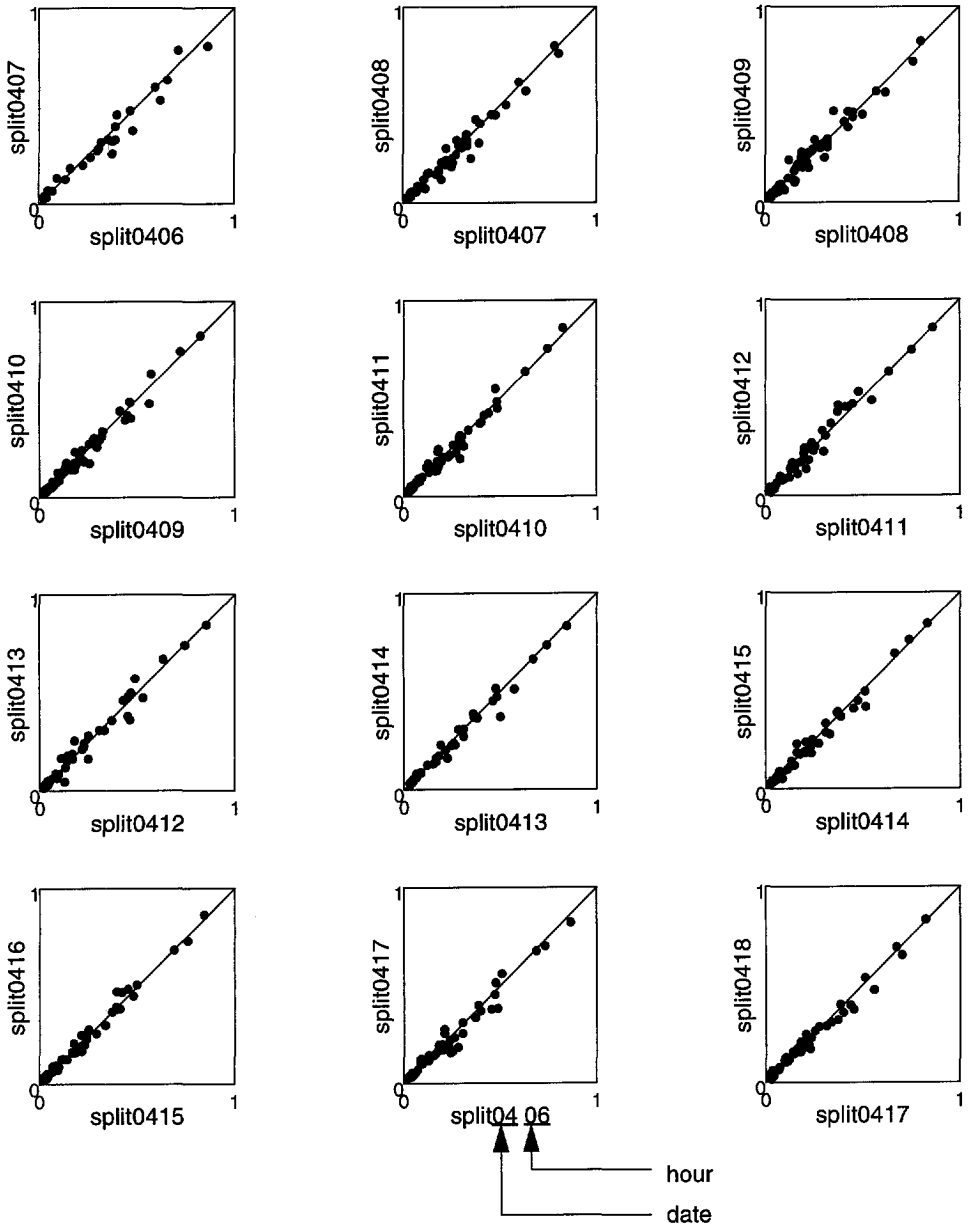
Figure 6.1: One hour-averaged split-ratios on the tollroad 'route du soleil' in France, plotted against the split-ratios during the previous hour of departure, measured from 6.00-18.00 on tuesday, August 4, 1992
