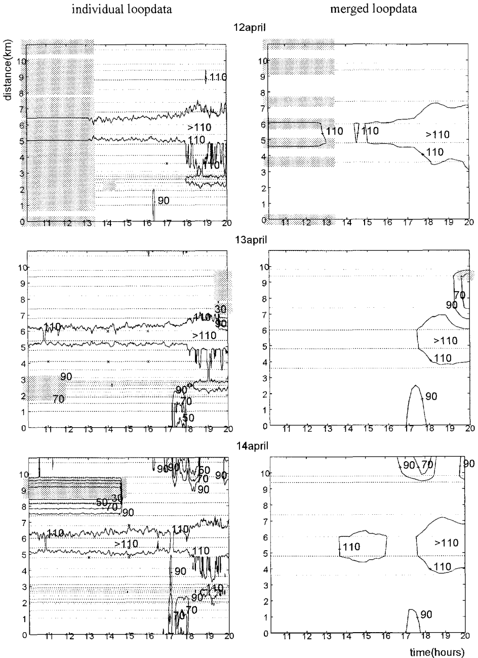
Figure 9.3: Contours of the observed velocities as a function of time and location. The dotted lines represent locations of induction loops. The gray bars represent missing data. Left: all induction loops are used. Right: induction loop data have been merged where appropriate, eliminating some of the missing data.
