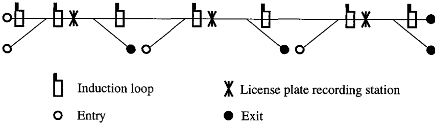
Figure 7.1: Sample network. Traffic data are collected with induction loops and license plate readers.
