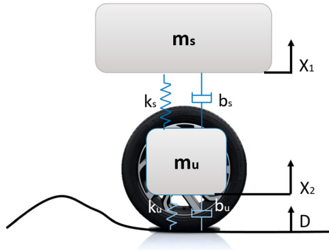
Figure 3. The quarter car linear oscillatory model used to model the suspension travel ( X1 - X2 ) for different road disturbance frequencies ( D ).
