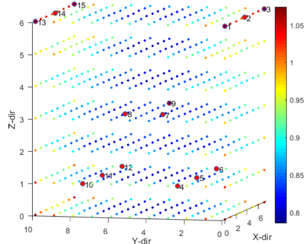
Figure 5. The total precision for possible user tag locations for the geometric configuration of 15 beacons.
