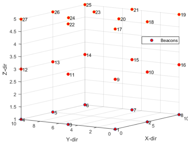
Figure 9. The 27 possible beacon locations for a 10x10x5 theoretical space.
