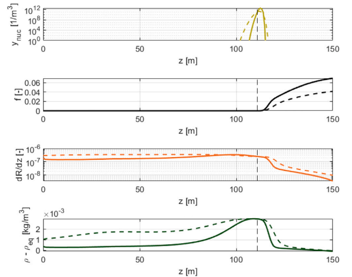
Fig. 10. \gamma_{nuc} , f , dR/dz and \rho - \rho_{eq} profiles of the channel with a smaller throat (solid lines) and the baseline channel (dashed lines). The vertical dashed line represents the location of the throat.
