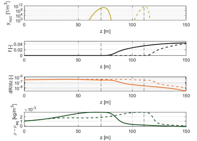
Fig. 7. \gamma_{nuc} , f , dR/dz and \rho - \rho_{eq} profiles. The solid lines are the results of the channel with the new throat location, the dashed lines are the results of the baseline channel, and the vertical dashed lines represent the locations of the throats.
