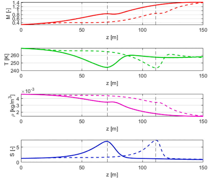
Fig. 6. M , T , \rho and S profiles of the baseline channel. The solid lines represent the results for the channel with the new throat location, the dashed lines are the results of the baseline channel, and the vertical dashed lines represent the locations of the throats.
