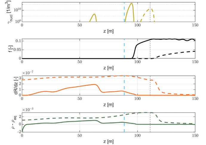
Fig. 13. \gamma_{nuc} , f , dR/dz and \rho - \rho_{eq} profiles of the baseline channel with accretion at the end of our 100-hour simulations (solid lines), compared to the initial baseline channel (dashed lines). The vertical dashed lines indicate the location of the throat at the end of our simulations (cyan) and at the beginning with the baseline channel (black).
