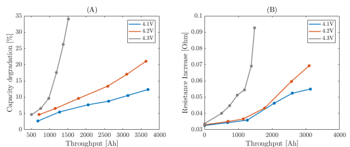
Fig. 16: Comparison of the capacity degradation (A) and resistance increase (B) of LCO cells tested at 1C, 25°C and various EOCV. significant increase in degradation is observed for the cells cycled up to 4.3V, and therefore too high EOCV should be avoided. Based on data obtained from [126]
