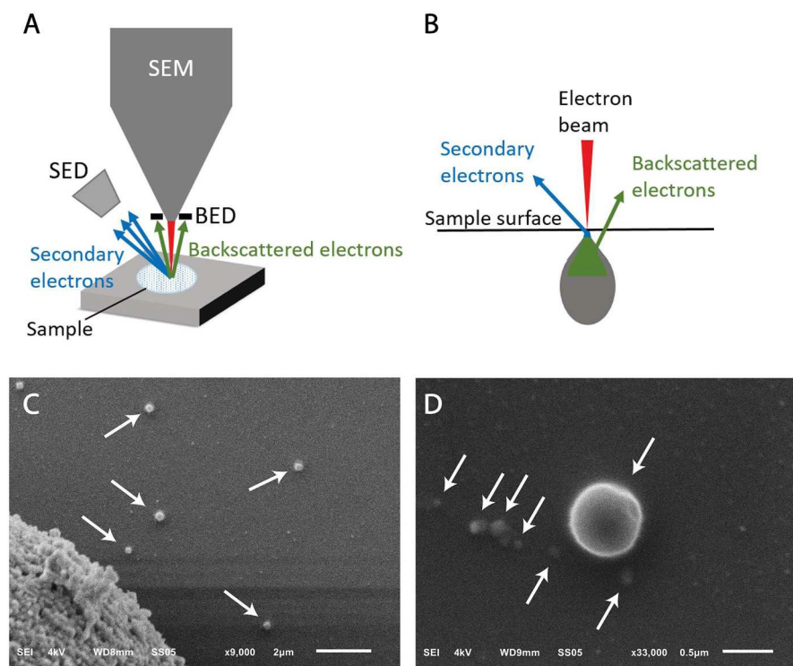
FIGURE 4 | Scanning electron microscopy (SEM) of extracellular vesicle (EV) samples. (A) Schematic representation of a SEM setup. SED, secondary electron detector; BED, backscatter electron detector. (B) The sample is illuminated by the electron beam. Electrons interact with the sample at different depths, resulting in emitted electrons from the surface (secondary electrons) and from deeper layers (backscattered electrons). (C) SEM image of LNCaP EVs indicated by arrows. The large object in the left lower corner is part of a LNCaP cell floating in the cell supernatant and was imaged to show that the contrast of EVs is similar to cells. The scale bar represents 2 \mu\text{m} . (D) Higher magnification allows imaging of smaller particles, possibly EVs, with lower contrast. The scale bar represents 500 nm.
