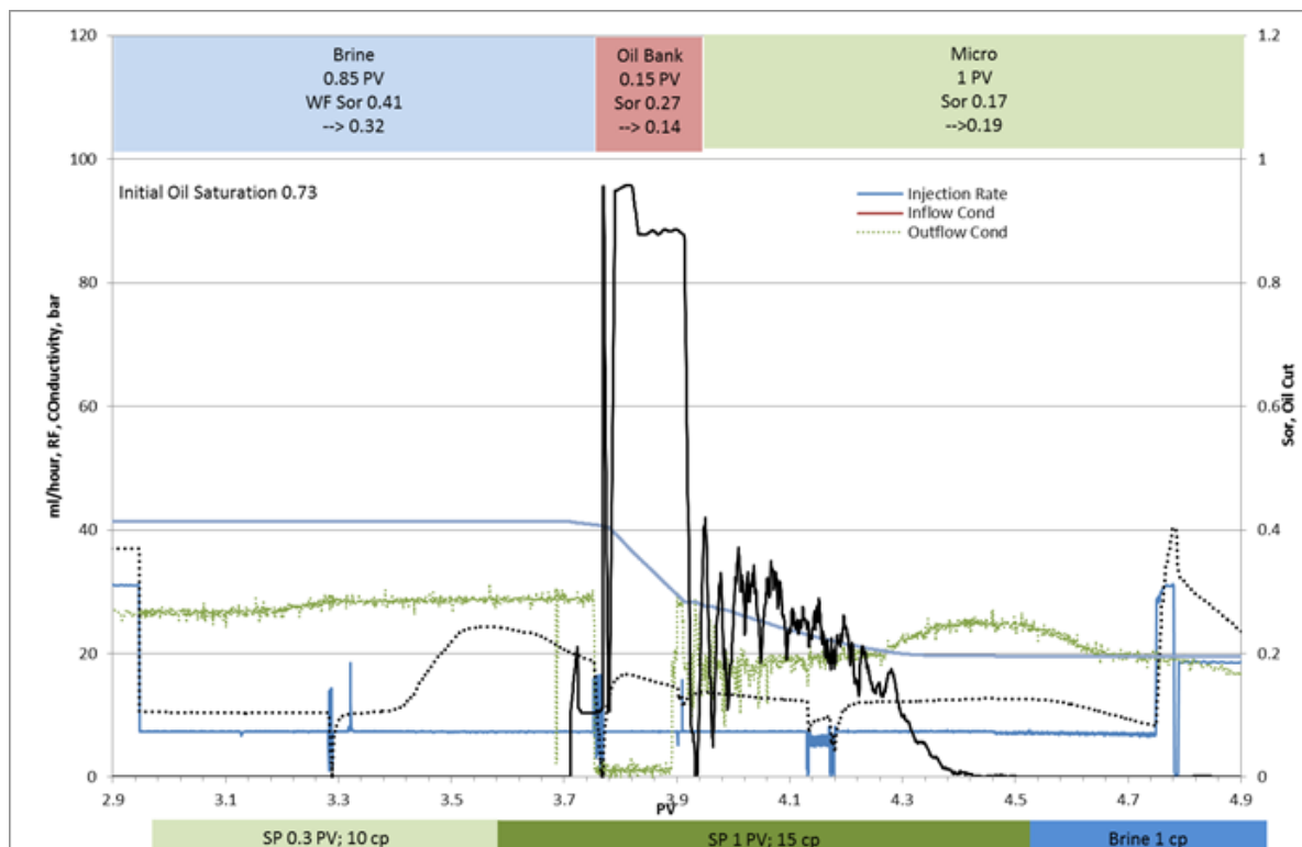
Figure 5.3: coreflow experiment in 10 mD sample; chemical slug is 0.3 PV
