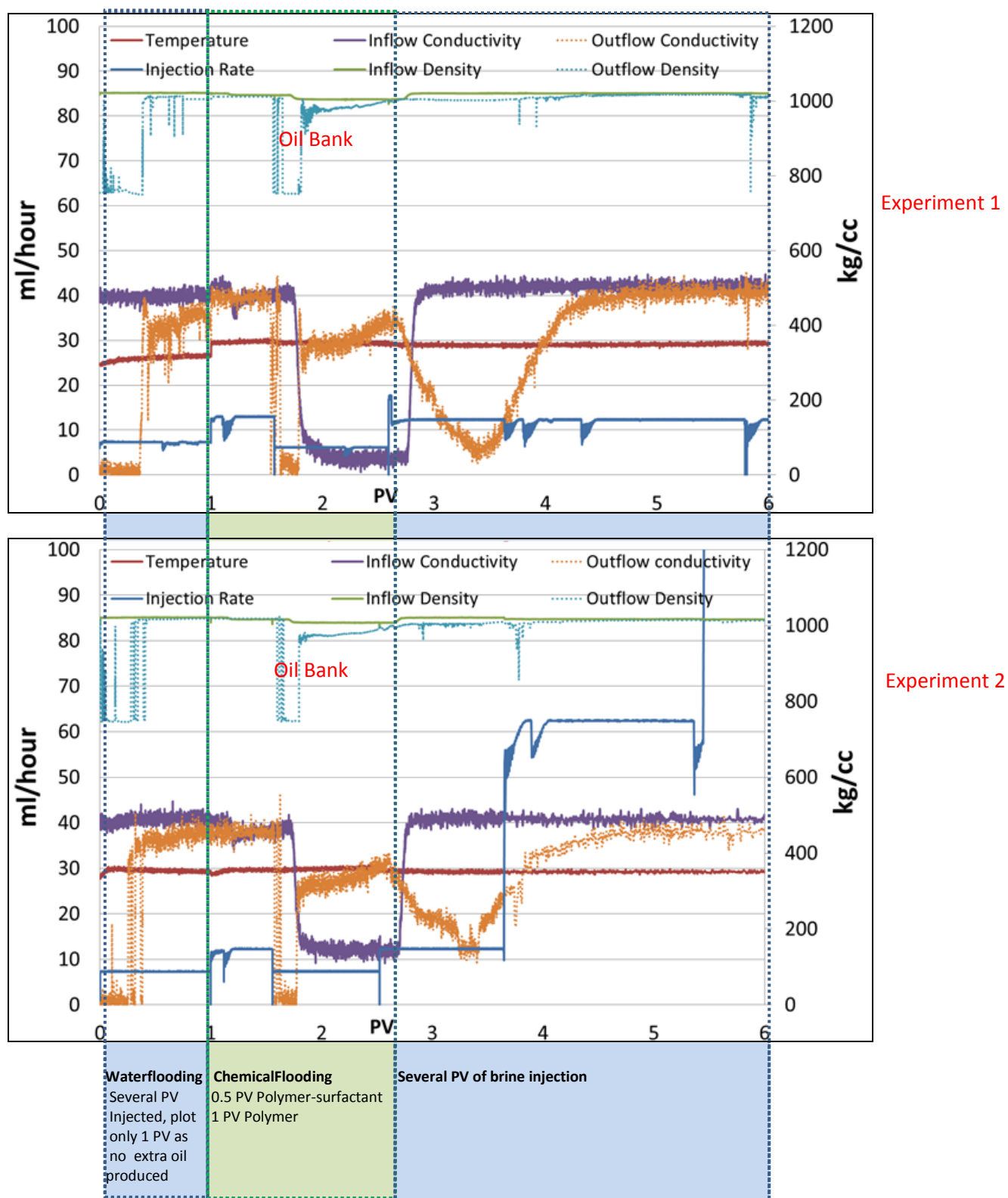
Figure 3.15: Two experiments repeated on the same core following the same experimental protocol to demonstrate the reproducibility of the experimental data. Oil Bank could be identified clearly at density of 750 kg/cc and conductivity of 0.
