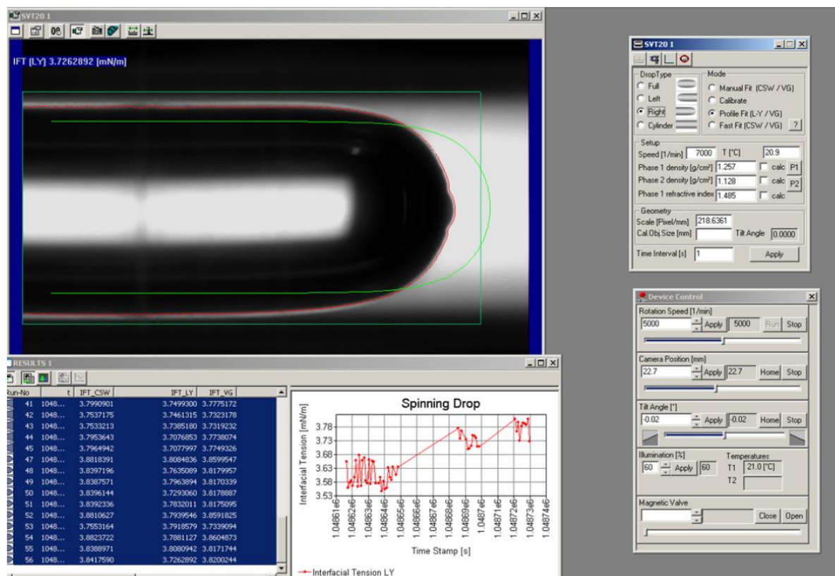
Figure 4.3: Screenshot showing the elongated oil droplet in the spinning drop tensiometer, as well the fitting software.
