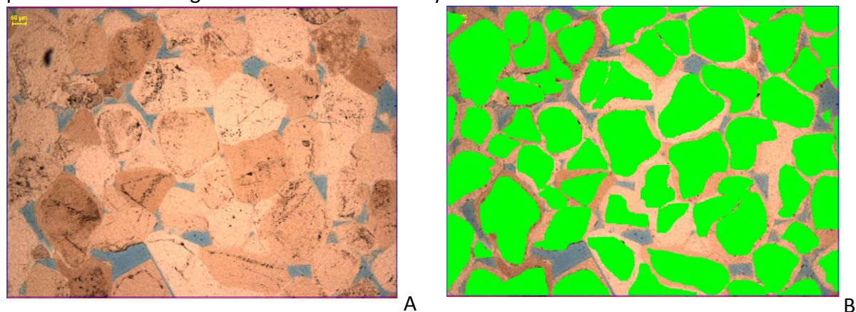
Figure 2.11: A. Quartz overgrowth around original “dirty” grains, In thin sections, the fines can be recognized as dark brown patches. These circular dust lines represent an earlier grain shape, which has overgrown at a later stage. The fines in the overgrowth part represent the rims of the grain shape before quartz overgrowth started. B. Definition of the original grain core (green) in the right image; the beige color shows the overgrowth, blue represents the pore space.
