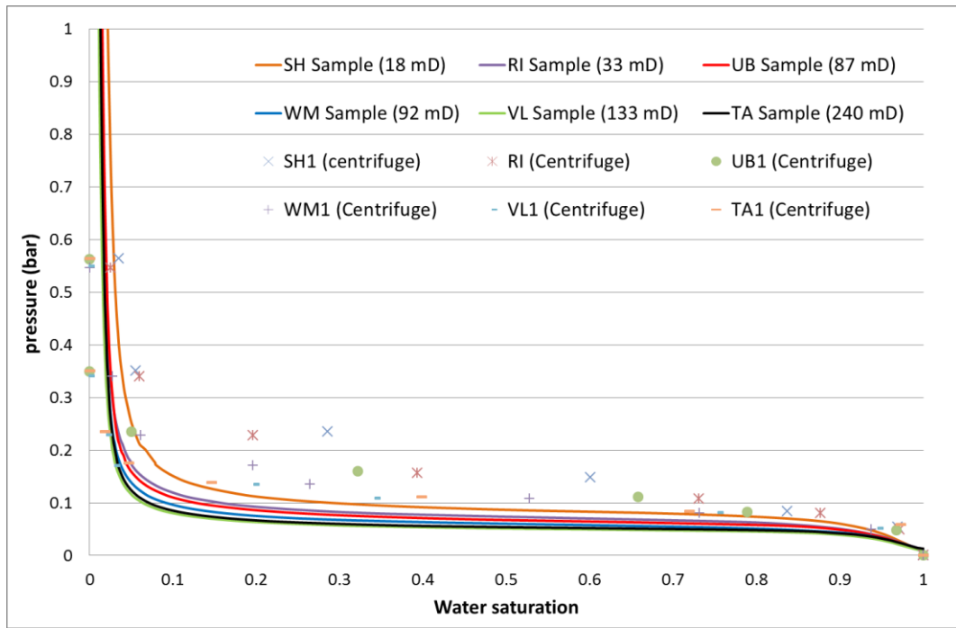
Figure 2.19: Fontainebleau centrifuge experiments (crosses, dots and lines) compared to the MICP data
