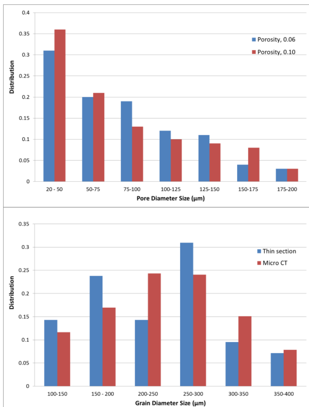
Figure 2.14: Pore and grain size distribution.
