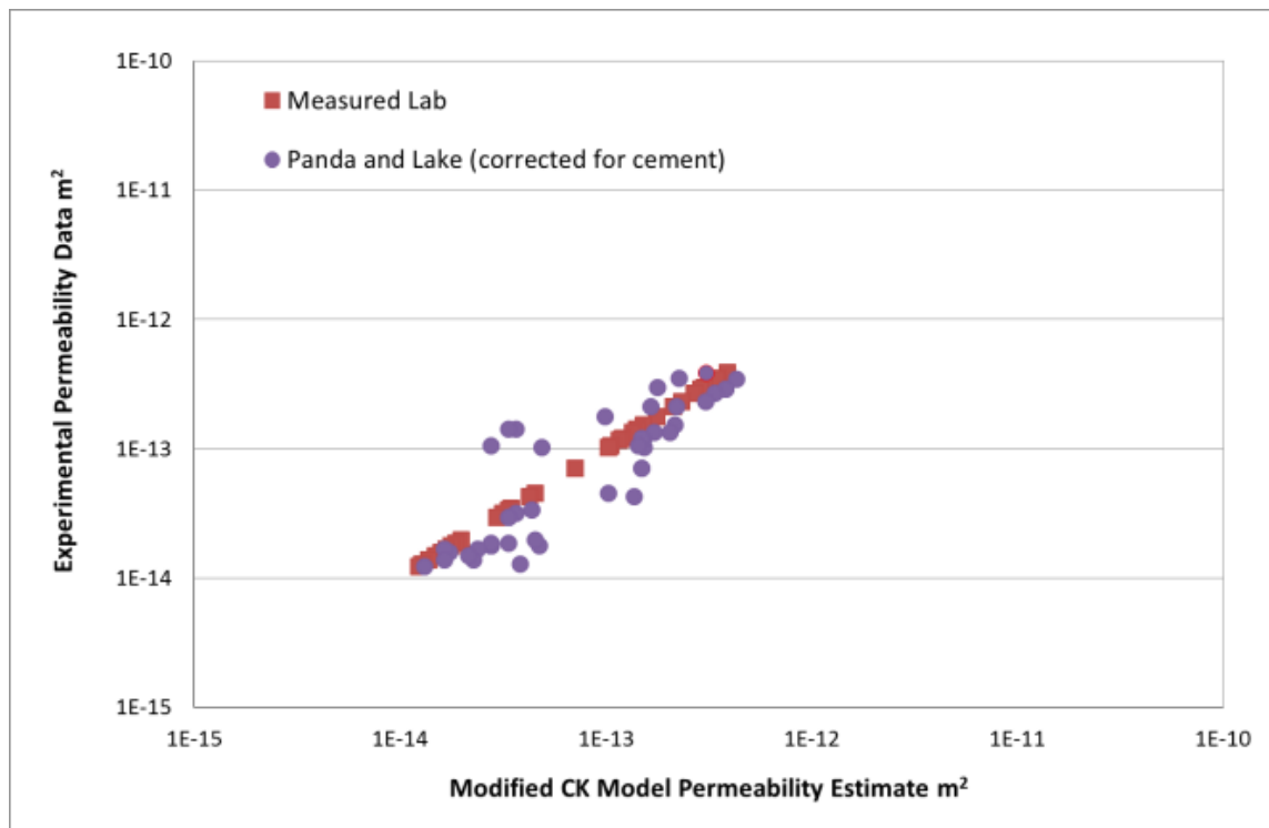
Figure 2.17. A. Variance between the permeability model estimation (not corrected for cement) versus the experimental data. B. Comparison but using the modified CK Model as proposed by Panda and Lake, which includes the effects of cements.
