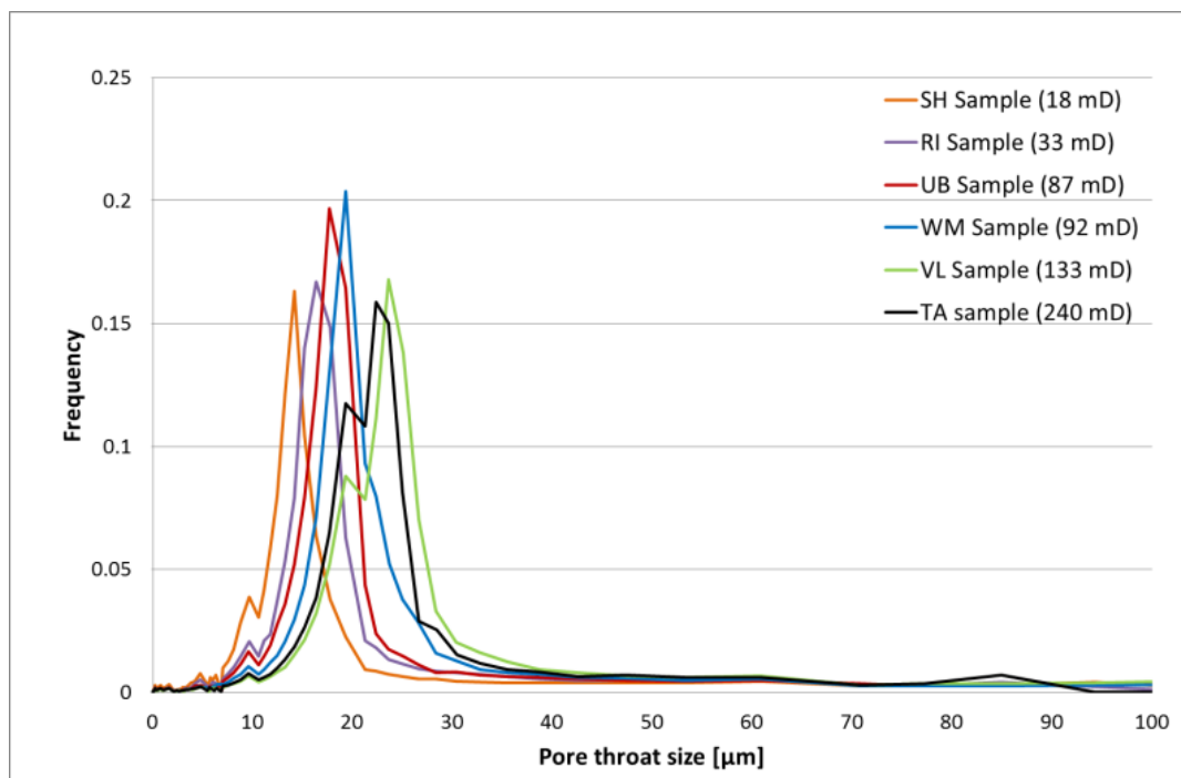
Figure 2.18: Fontainebleau Pore throat size distribution from MICP
