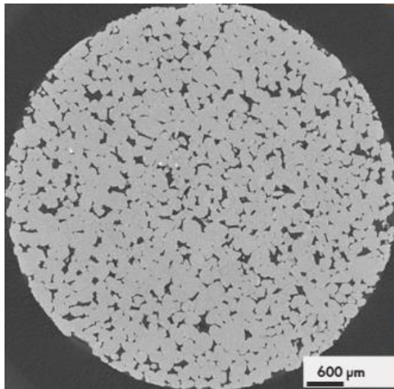
Figure 3.1A: Images of Fontainebleau sample, Micro-CT slice, representing the grain aggregate (light) and pore space (black).
