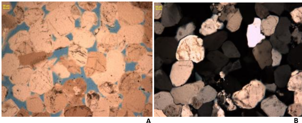
Figure 2.3: A: Fontainebleau thin section image. B: Image with polarized light
