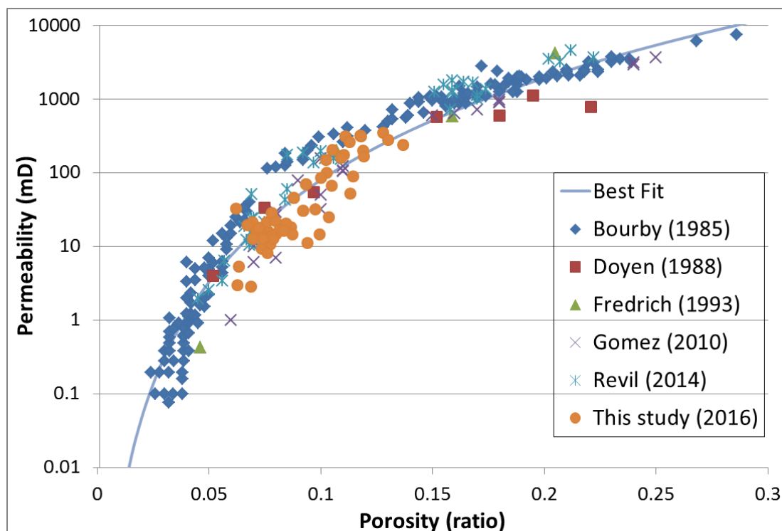
Figure 2.16: Porosity vs Permeability of Fontainebleau sandstone
