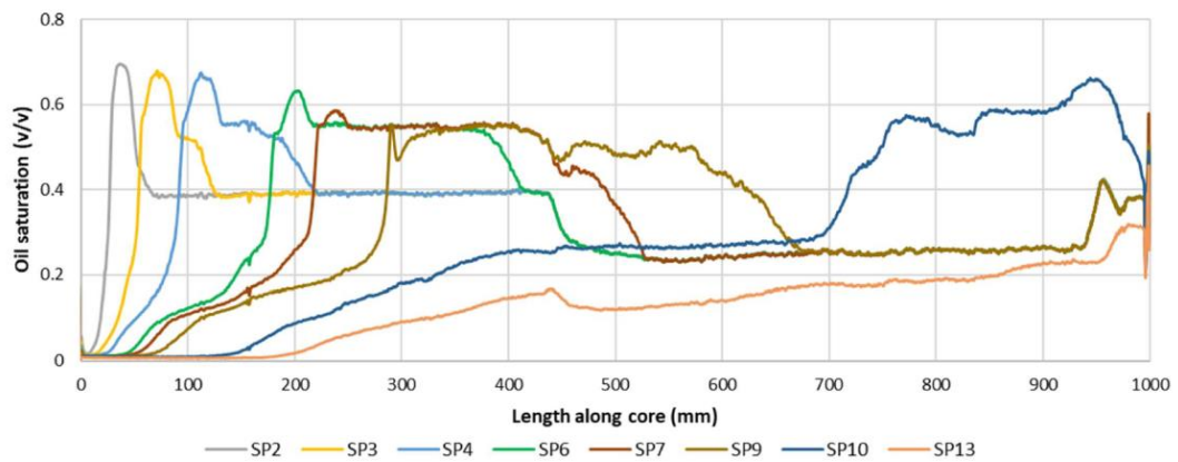
Figure 5.15: Oil Saturation across 1 m Bentheimer core. The saturation profiles composed from the CT-scans labelled as SP1-13. Scan SP1-13 show that the highest oil saturation is directly ahead of the SP-slug and the oil bank volume increases across the core.
