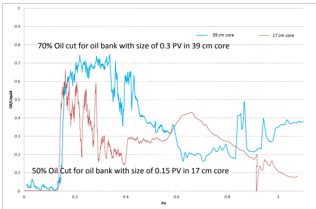
Figure 4.10: Oil cut profiles at the exit of the core for coreflow experiments with 17 and 39 cm core lengths.
