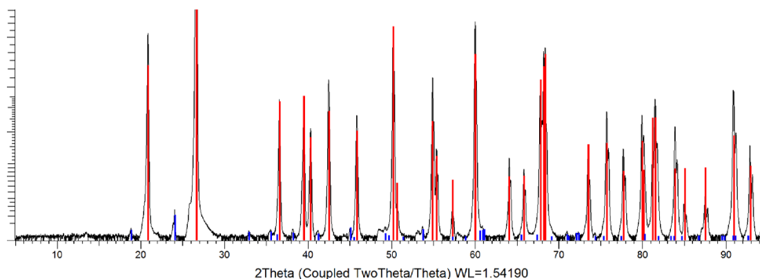
Figure 2.8: The measured XRD pattern in black, after background subtraction. The red lines are peak positions and intensities of known mineral phases. Only quartz was found; the extra peaks, indicated with the blue stick pattern, are due to the Kb contribution in the incident X-ray beam.
