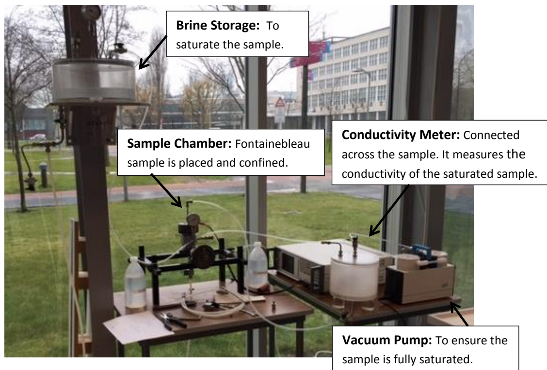
Figure 2.6: Set-up for measuring conductivity.
