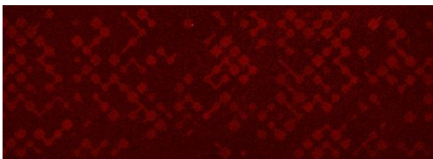
A: After Waterflooding, Oil is disconnected and at residual condition, the lighter red parts represent the accumulated oil phase, the dark parts are the brine phase and pore space.
