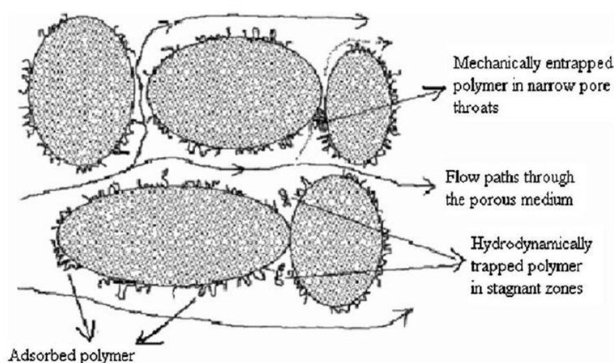
Figure 5.8: Polymer entrapment mechanisms in porous medium (Sorbie, 2014)
