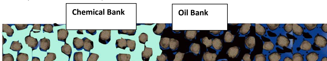
Figure 5.6: schematic of Oil Bank build up in 2D model
