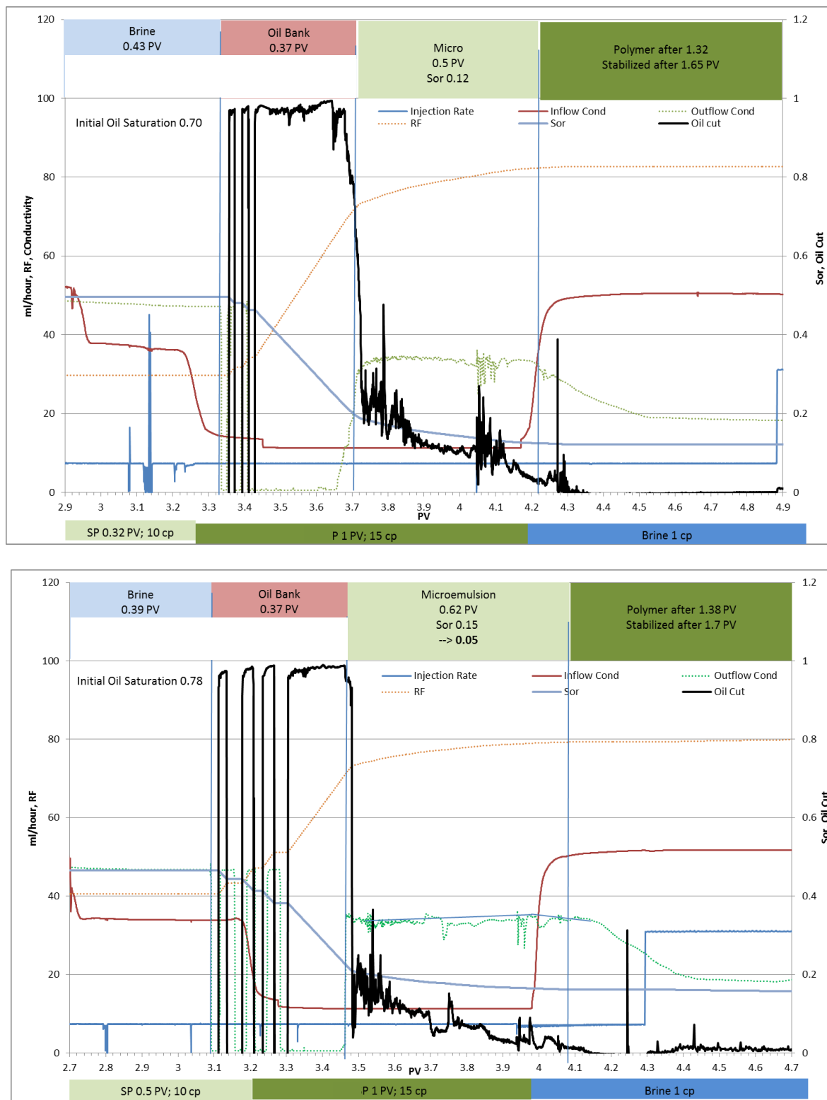
Figure 4.11: coreflow experiment in 80 mD sample; Top: chemical slug is 0.3 PV; bottom: chemical slug is 0.5 PV
