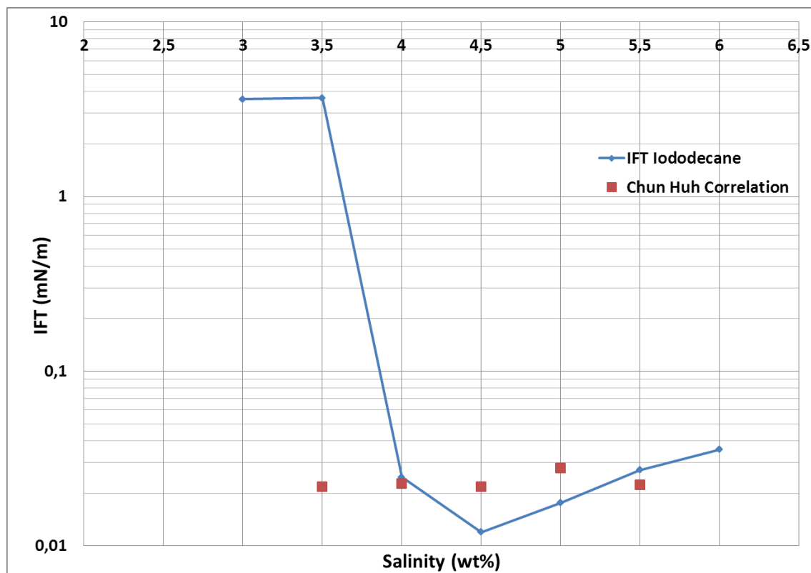
Figure 4.8: IFT measurements for iodododecane/surfactant/brine system at different salinities.
