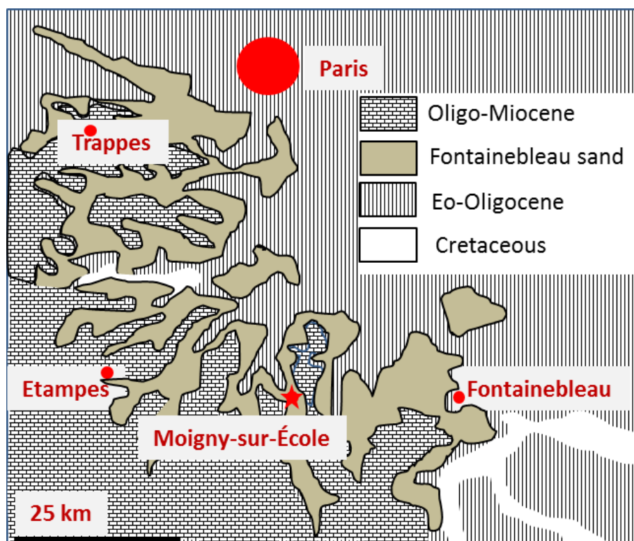
Figure 2.1: The layout of Fontainebleau sandstone. ★ The Grès de Fontainebleau & Cie quarry in Moigny-sur-École for rock sampling (Quarry coordinates: 48.434237,2.433944). Modified after: Thiry et al., 1988.
