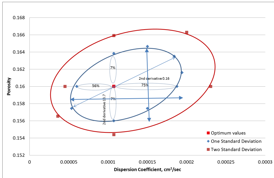
Figure 3.13: Statistics of the effective porosity against dispersion based on Gaussian LSQ analysis
