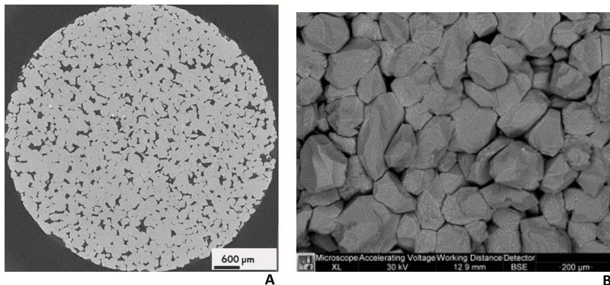
Figure 2.4: Fontainebleau images, A: Micro-CT, B: SEM
