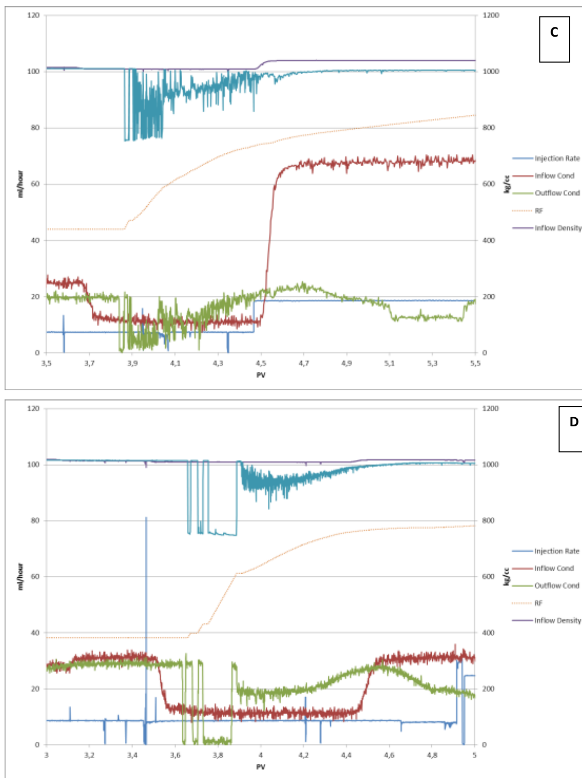
Figure 5.9: Core flow results on the same core. Figure 5.9 A shows the results of the 1 st coreflow experiment. Figure 5.9 B 5.9 C presents two repeated experiments where we could reproduce same results as in the 1 st experiment. After further investigation, we identified the reason as the change of chemical formulation over time. By preparing a new chemical formulation we managed to reproduce the results as seen in Figure 5.9 D.
