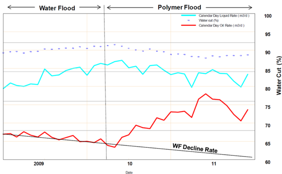
Figure 1.2: Oil gain due to polymer injection (Al-Saadi et al, 2012)
