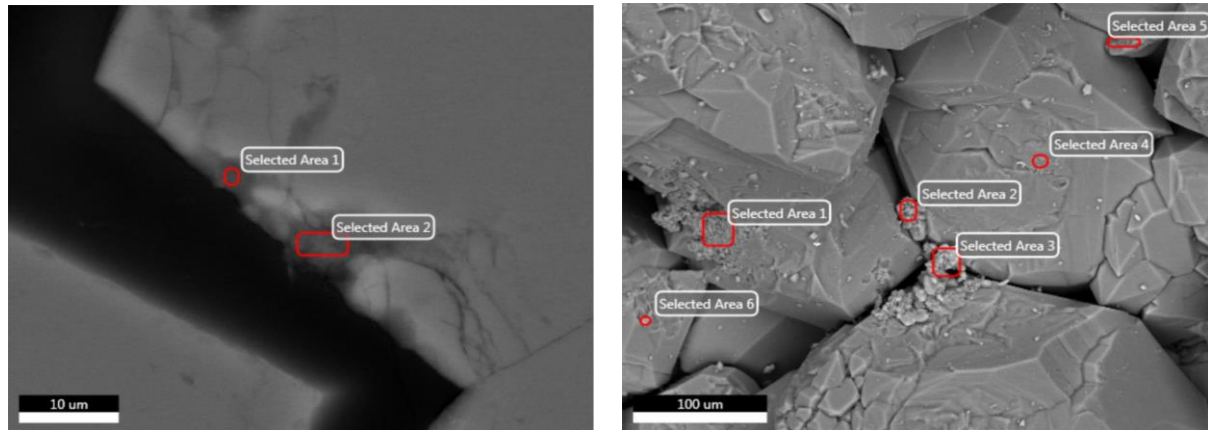
Figure 2.10: Selected Areas via SEM to examine the presence of clay.
