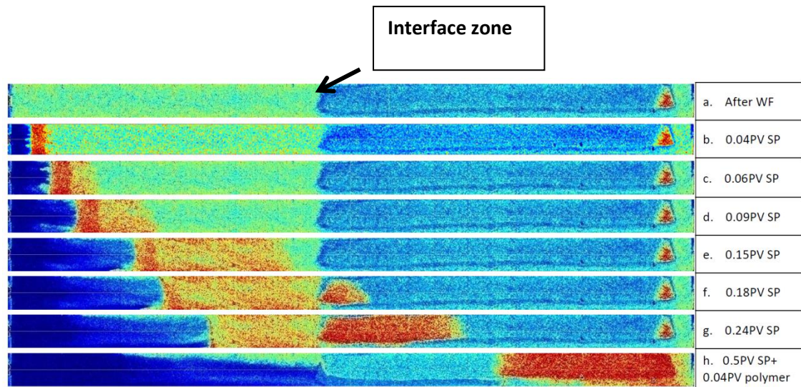
Figure 5.14: CT scans for 1 m Bentheimer core.
