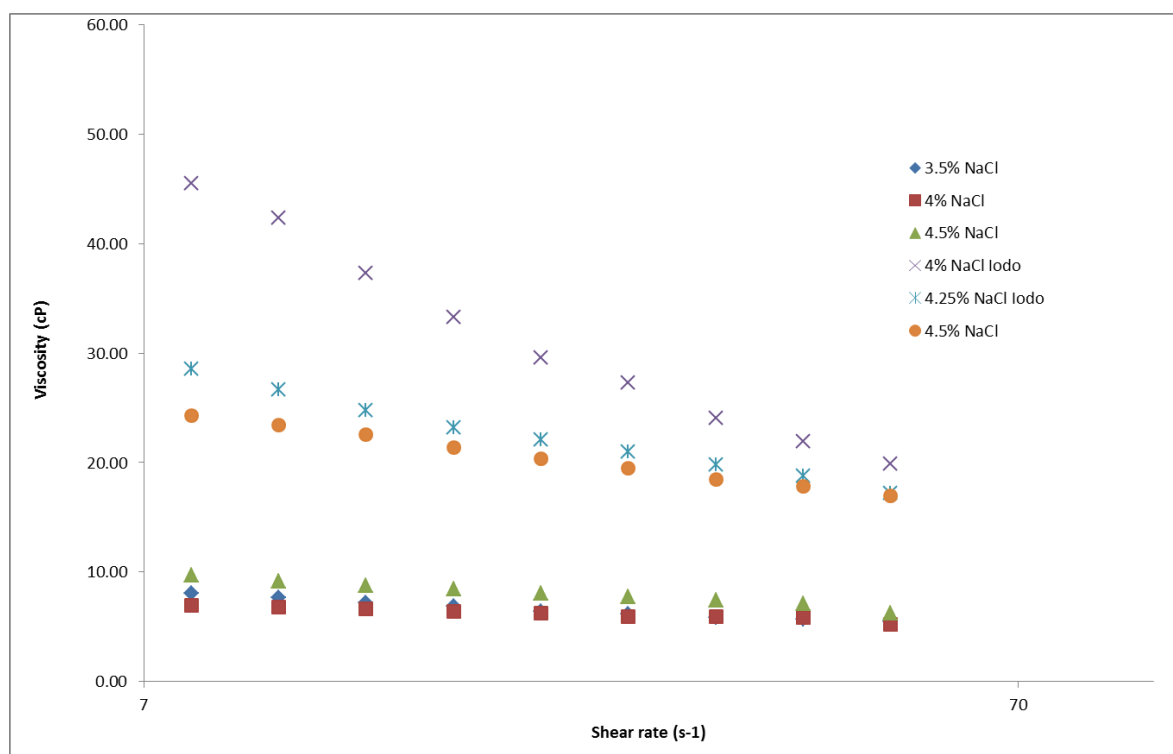
Figure 4.16: viscosity measurements for the dodecane/surfactant and iodododecane/surfactant systems.
