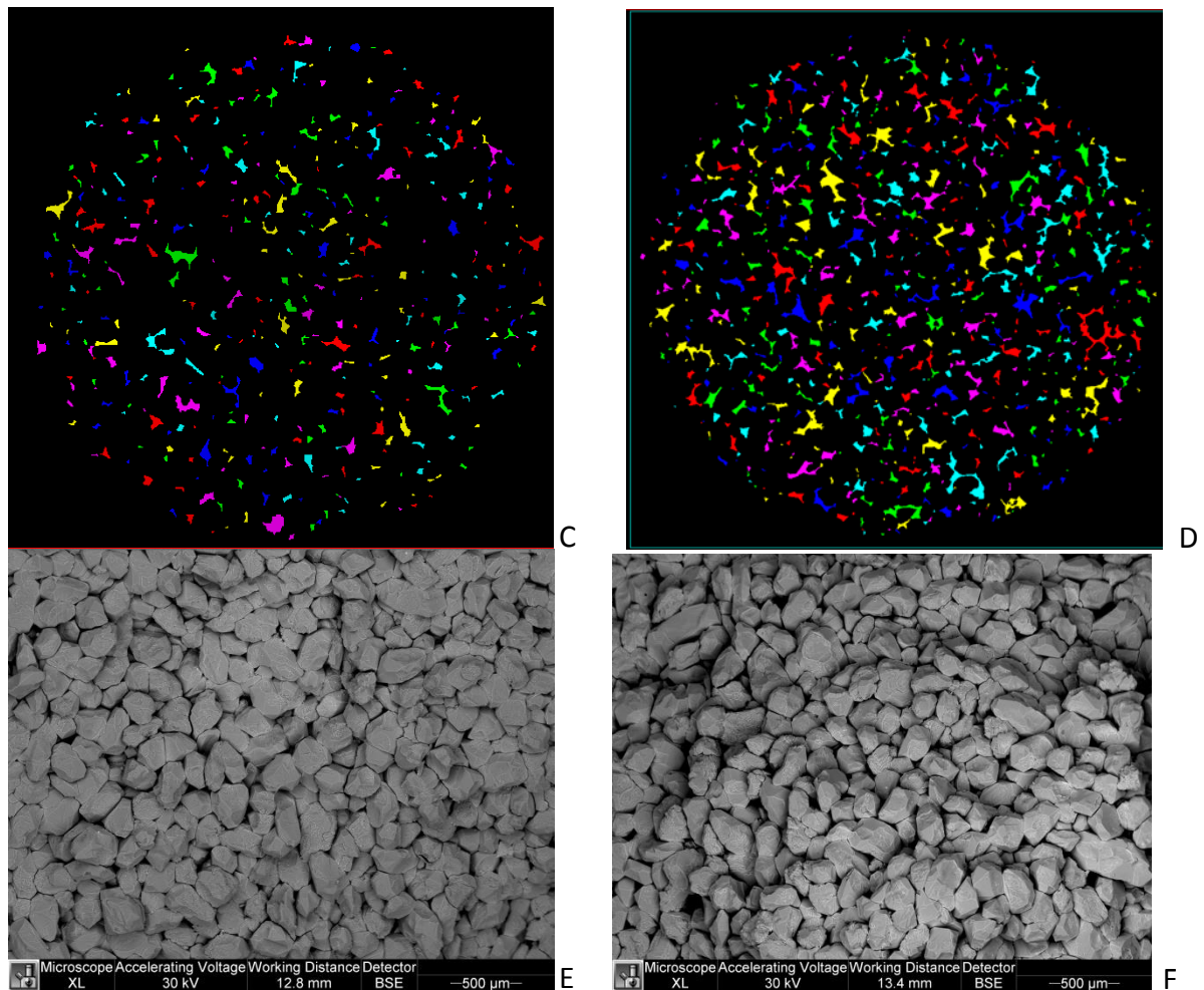
Figure 2.13: Thin sections (matrix grains and overgrowth and pores), Micro-CT images (pore space detection) and SEM (grain framework surface characterization)
