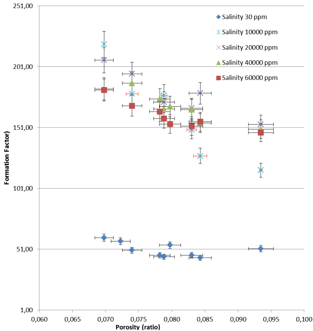
Figure 2.22: Formation Factor vs Porosity
