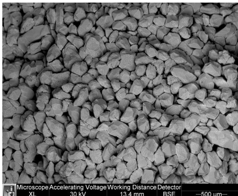
Figure 3.1B: Images of Fontainebleau sample, SEM where the grain aggregate representation shows the angular particles due to quartz overgrowth.
