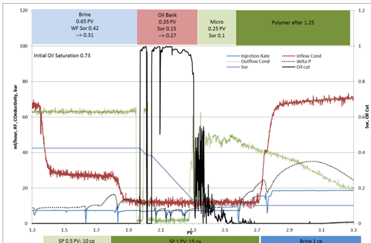
Figure 5.4: coreflow experiment in 10 mD sample; chemical slug is 0.5 PV
