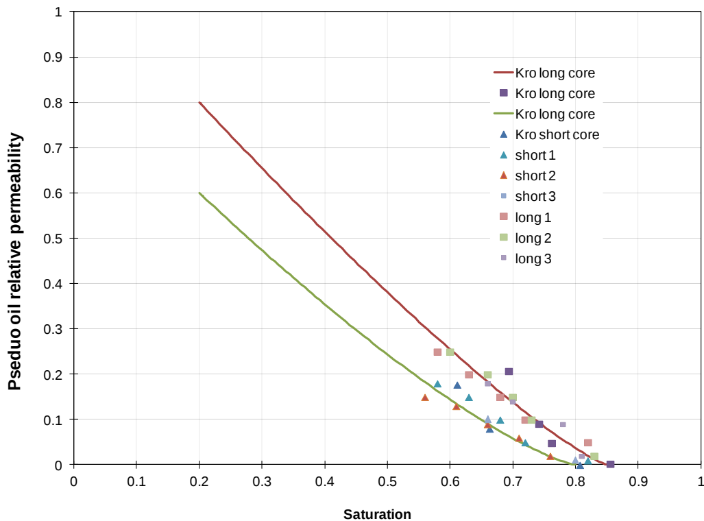
Figure 5.17: oil mobility for different core lengths. (Y-axis: Pseudo relative permeability)
