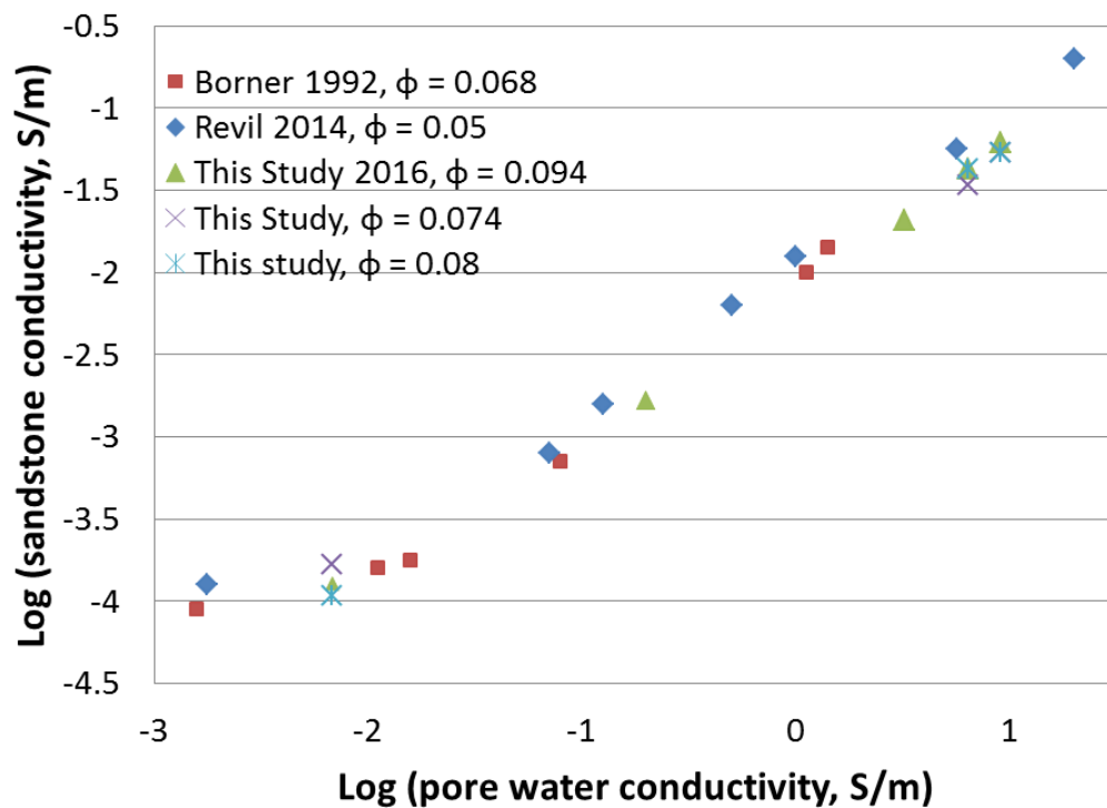
Figure 2.5: Saturated Fontainebleau sample conductivity vs brine conductivity
