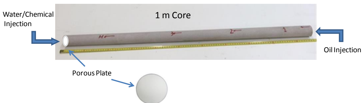
Figure 3.6: The flow configuration of the 1 m sample with the porous plate at the water/chemical injection side.
