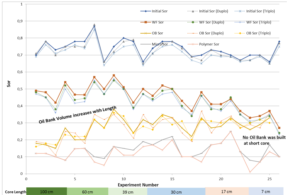
Figure 5.16: Demonstrations of Reproducible Coreflow experimental data for 78 coreflow experiments. X-axis represents the Number of experiments and the core length of the core used in each experiment. Y-Axis represents the remaining average oil saturation after each flooding step (Initial S_{or} is the initial oil saturation after oil filling, WF S_{or} is the oil saturation after waterflooding, OB S_{or} is the oil saturation after oil bank, Polymer S_{or} is the residual oil saturation after polymer flooding). The dotted lines represents the 1 st and 2 nd repetitions of the experiments on the same core.
