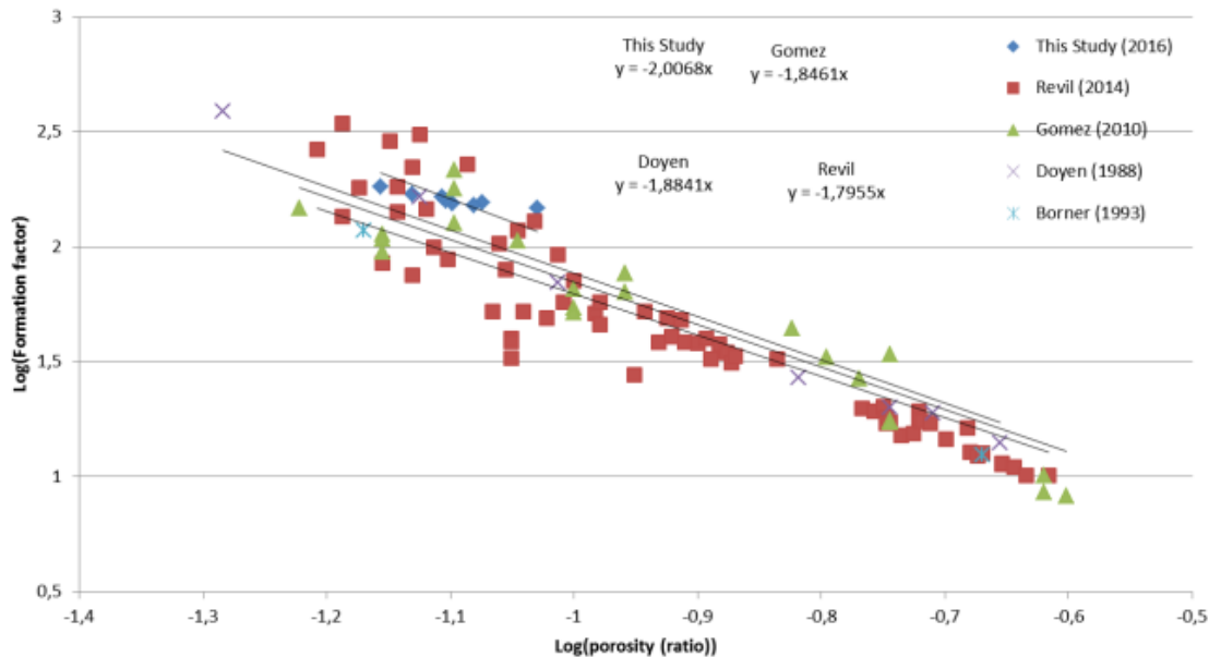
Figure 2.23: Log (formation factor) vs log (porosity).
