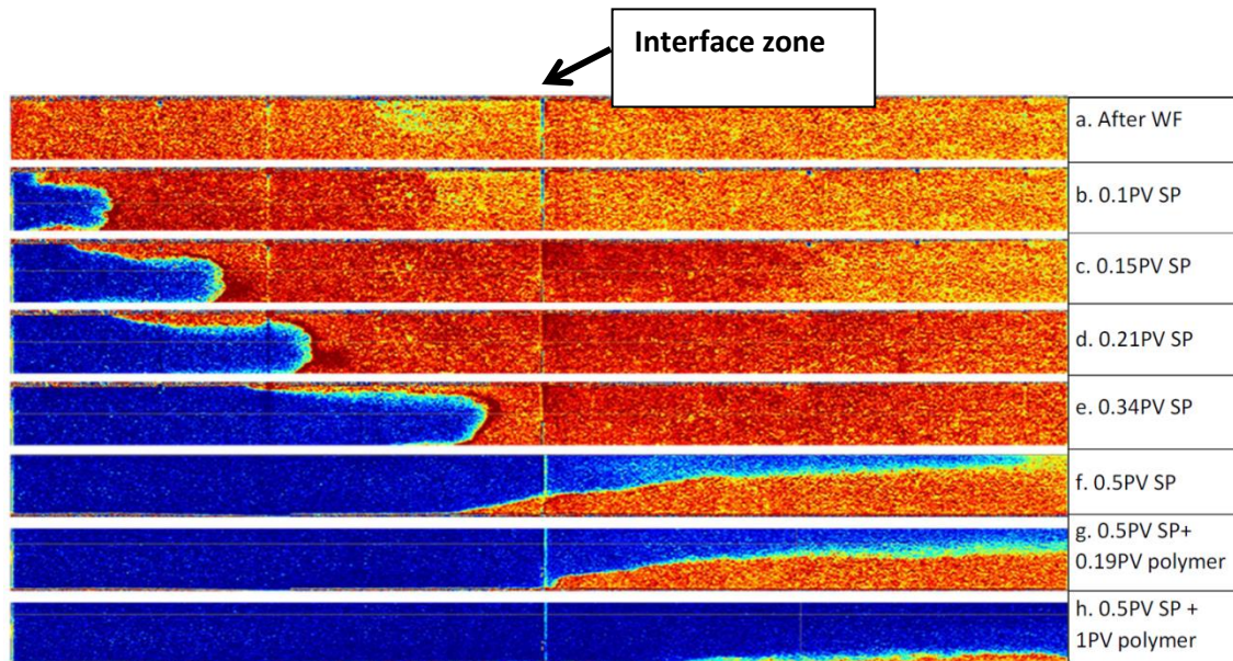
Figure 5.13: CT scans for 60 cm stacked core Fontainebleau. Same experimental protocol as explained in chapter 3 was used.
