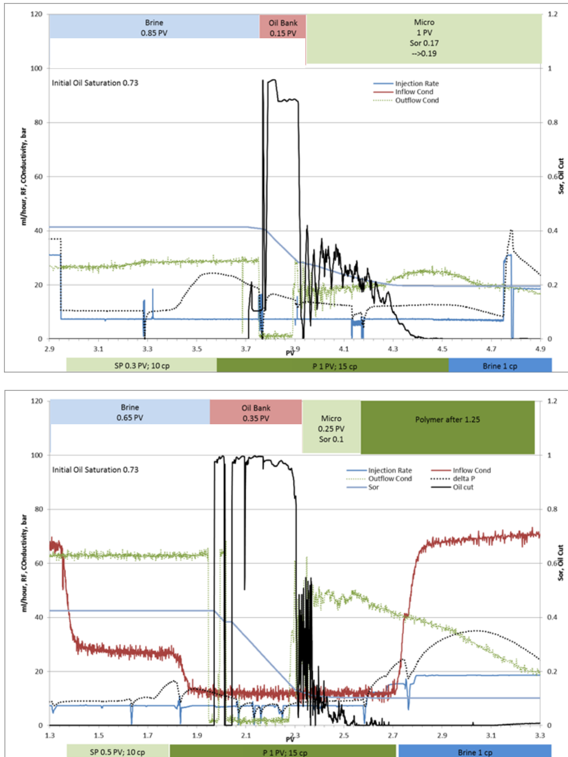
Figure 4.12: Coreflow experiment in 10 mD sample; Top: chemical slug is 0.3 PV; bottom: chemical slug is 0.5 PV
