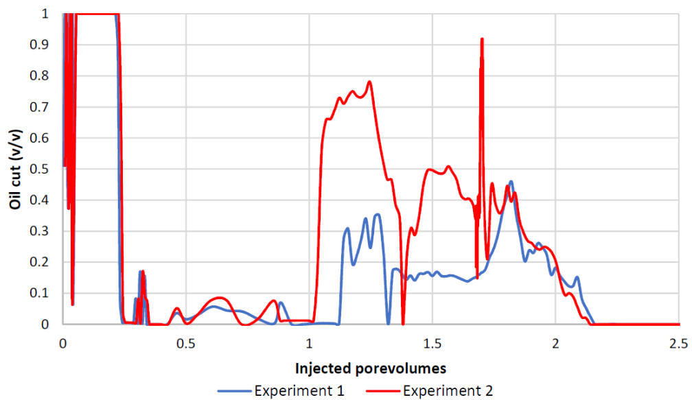
Figure 5.12: Oil cut for two different experiments at different IFT.
