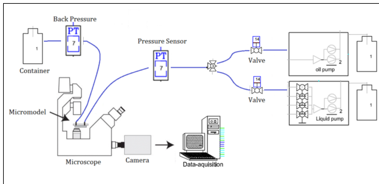
Figure 3.3: Schematic design of the Microfluidic setup
