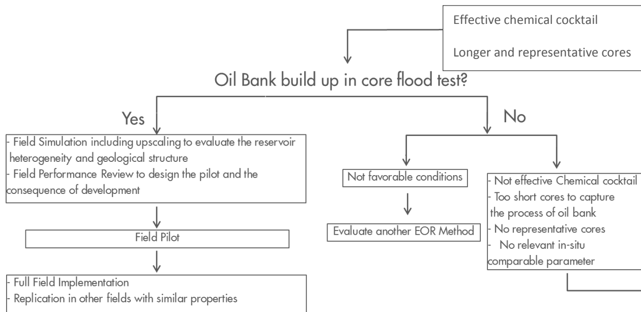
Figure 1.4: A decision tree on building an oil bank in core-flow tests.
