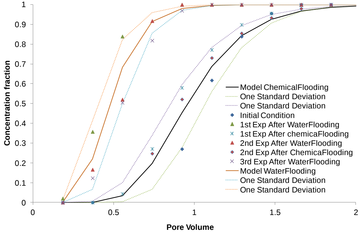
Figure 3.11: Tracer experimental data in effluent and model data.
