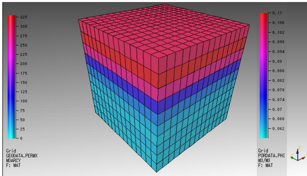
Figure 2.15: Permeability and Porosity variation within the block.
