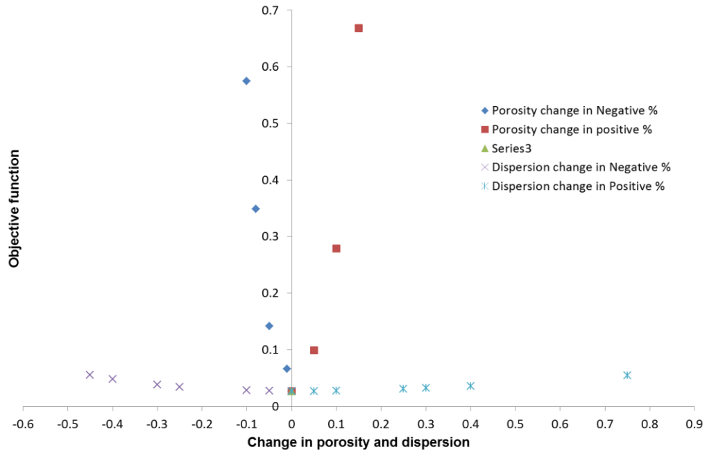
Figure 3.12: Change in porosity and dispersion.
