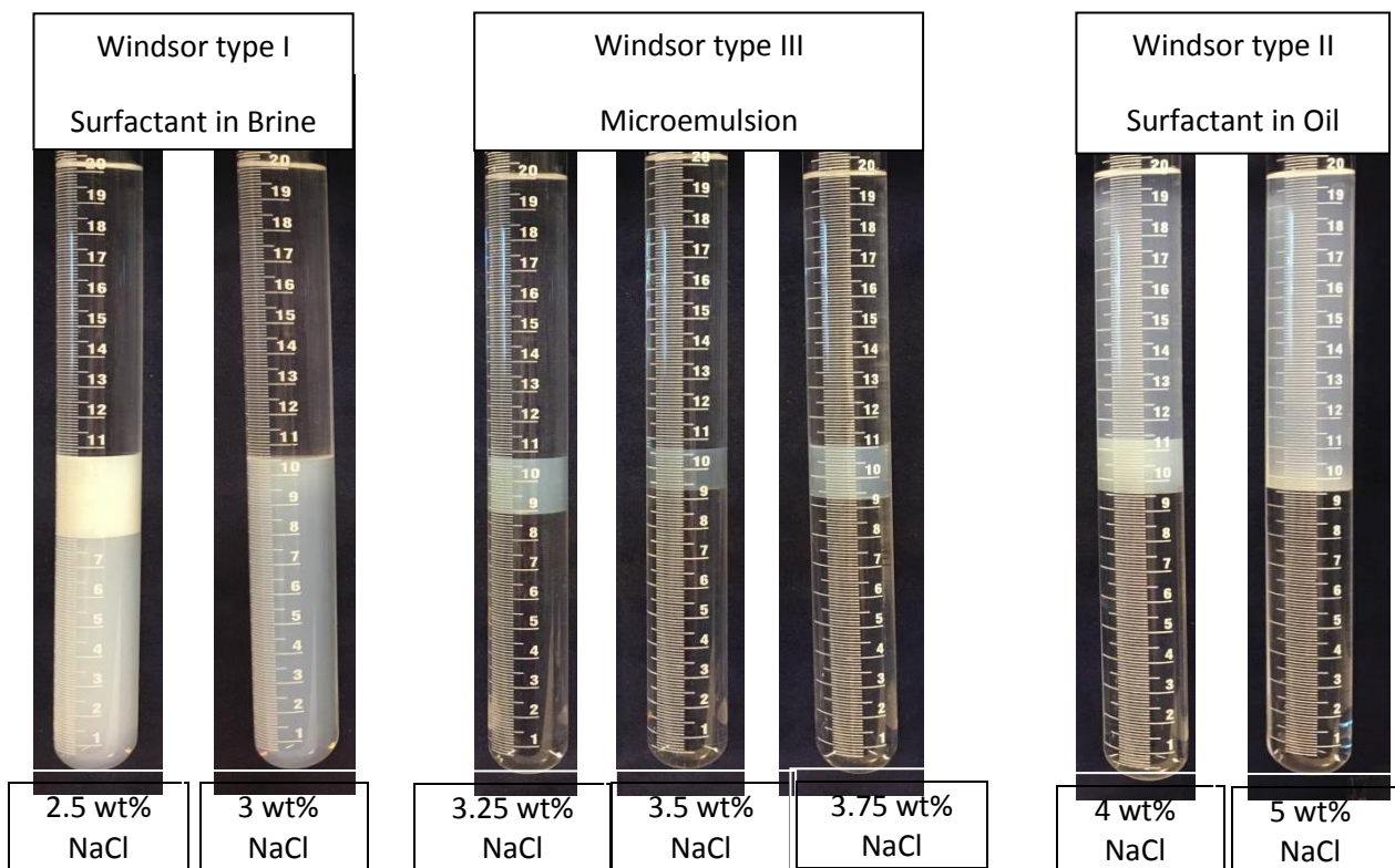
Figure 4.4: Visualisation of the phases during phase behaviour of a dodecane/surfactant/brine system at different salinities at ambient temperature.
