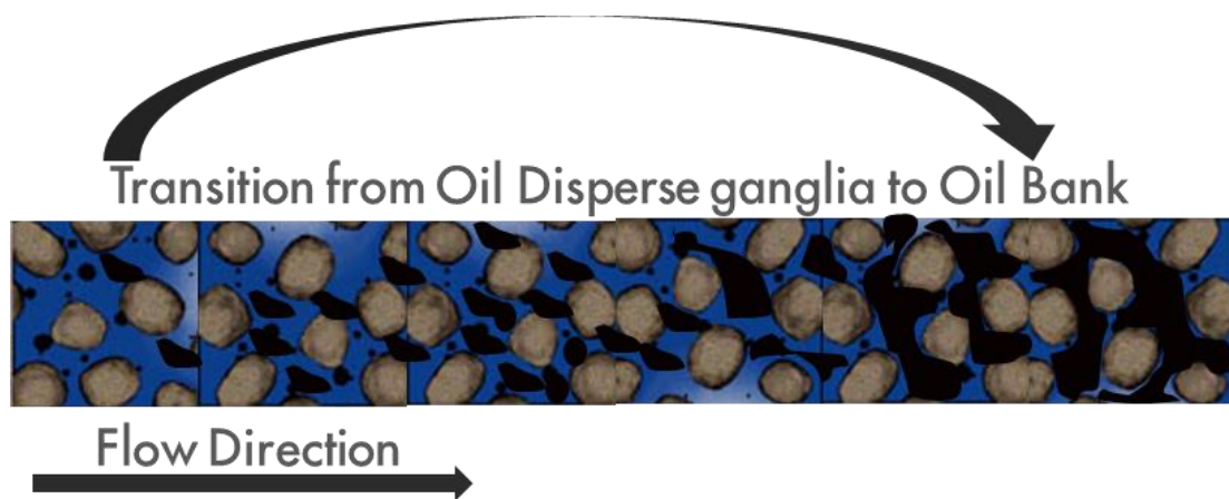
Figure 4.1: 2D Schematic of porous media; oil ganglia (black), brine (blue) and porous media grains (brown).
