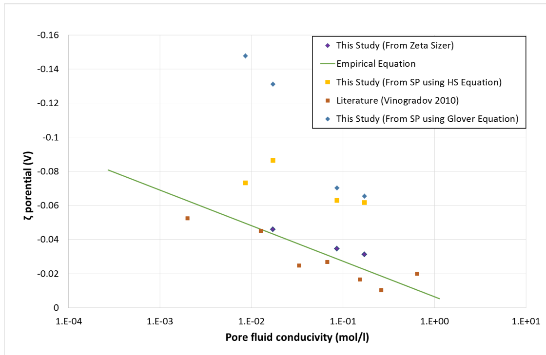
Figure 2.25: Fontainebleau Zeta potentials
