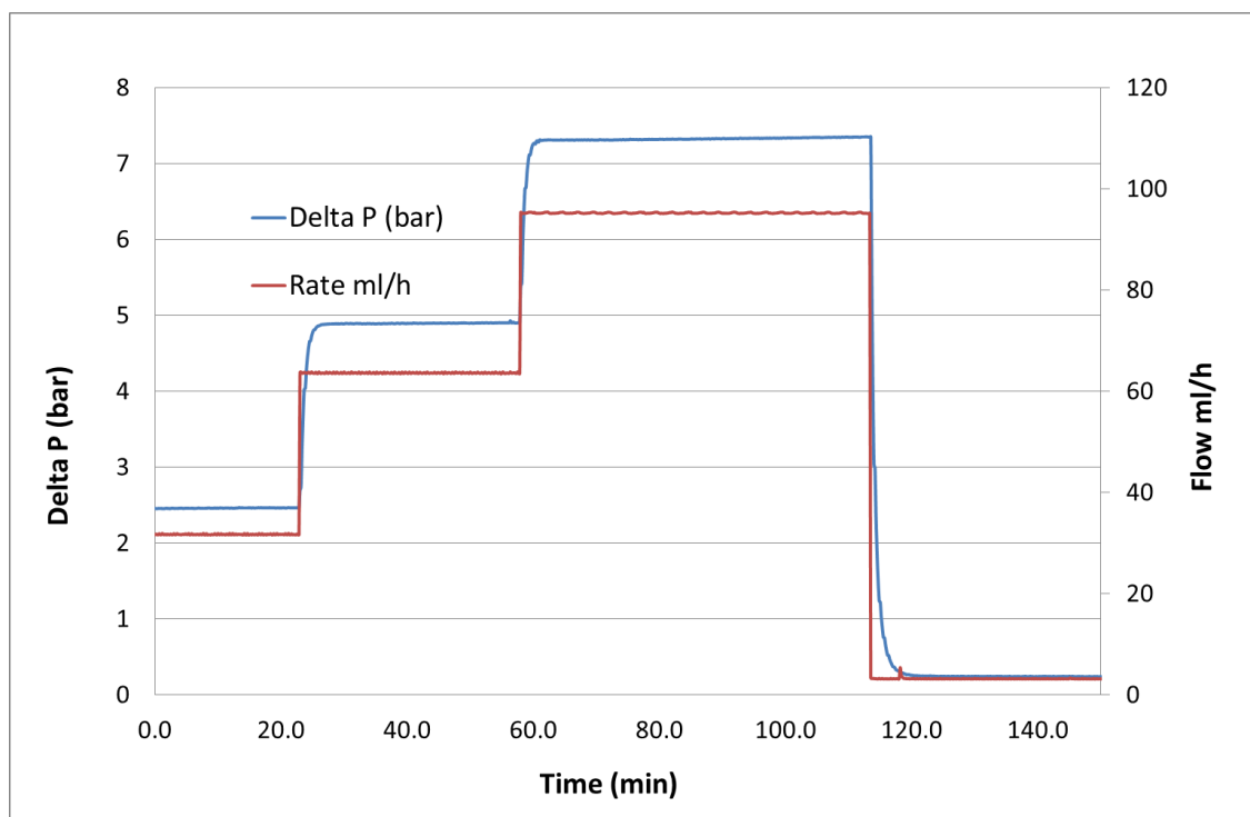
Figure 3.10: Differential pressure and flow rates vs time.
