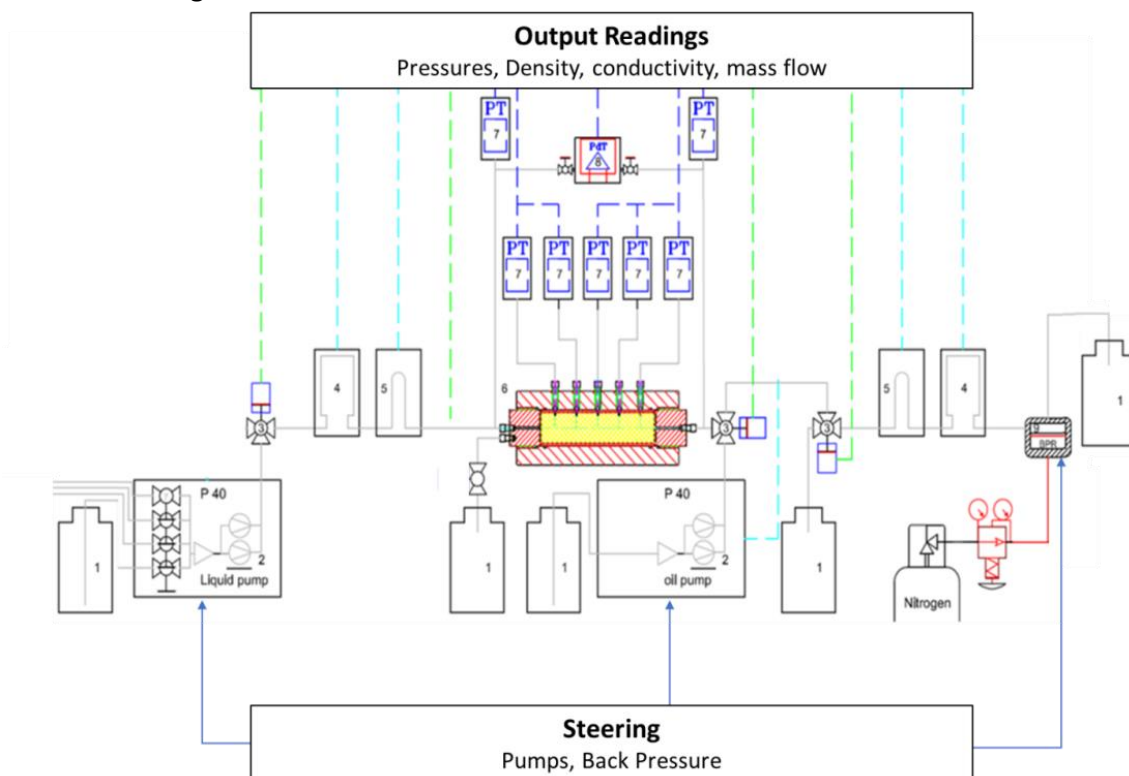
Figure3. 7: Schematic design of the core flow setup. The numbers correspond with the set-up description here below.
