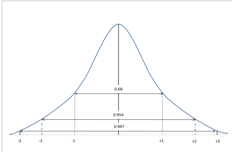
Figure 3.9: Areas enclosed by standard deviations of the standard normal distribution.
