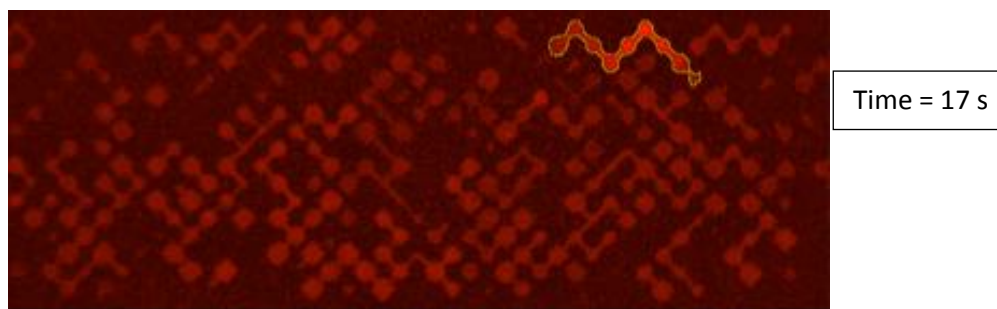
Figure 3.5: The propagation of an oil ganglion, size 0:187 mm 2 at different time steps.
