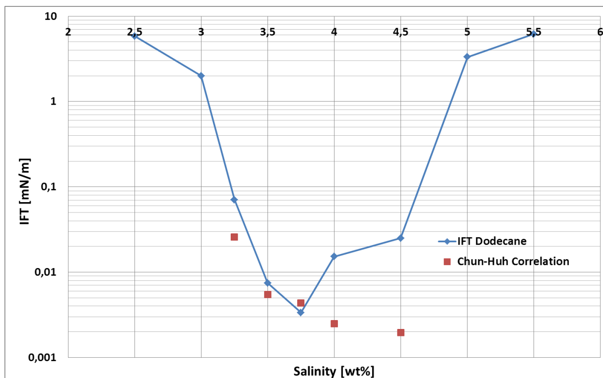
Figure 4.7: Spinning drop IFT measurements for dodecane/surfactant/brine system at different salinities and calculated IFTs based on solubilisation ratio and the Chun Huh correlation.
