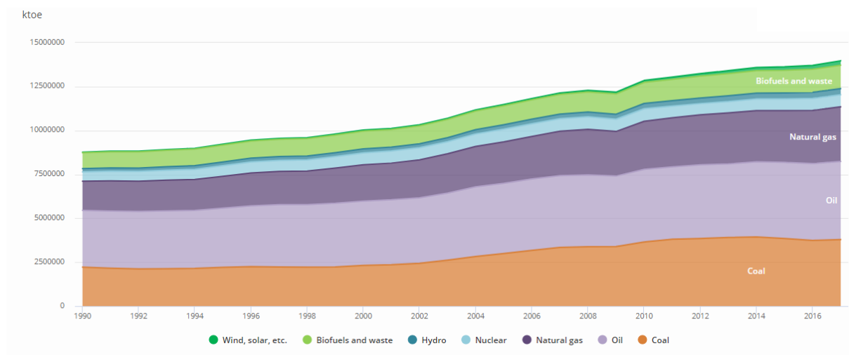
Figure 1.1: Total primary energy supply by source, World 1990 – 2017. Source: World Energy Balance 2019
