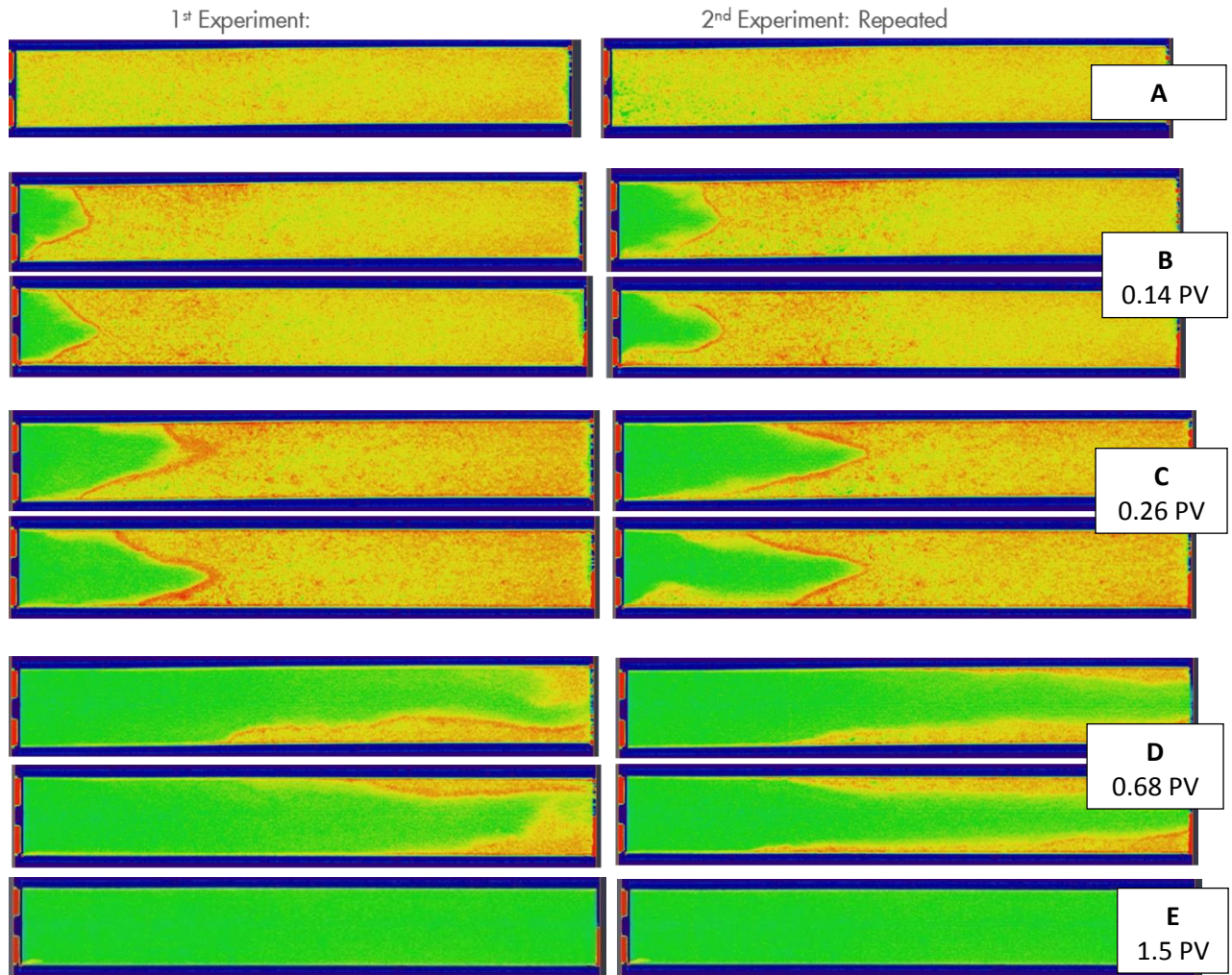
Figure 3.14: Synchronized CT scans at the same PV with chemical injection. The left-side images are the first experiments, the right side images represent the repeated experiments. Each PV is labelled from A to E. From each stage new phase injection stage we present a cross section in the horizontal and vertical cross-sections. Figure 3.14A present the residual oil status after waterflooding. Figure 14B, 14C show the surfactant movement and oil bank build up after 0.14 and 0.26 PV SP injected respectively. Figure 14D demonstrate the SP breakthrough after 0.68 PV. Figure 3.14E confirms that oil is swept after 1.5 PV.
