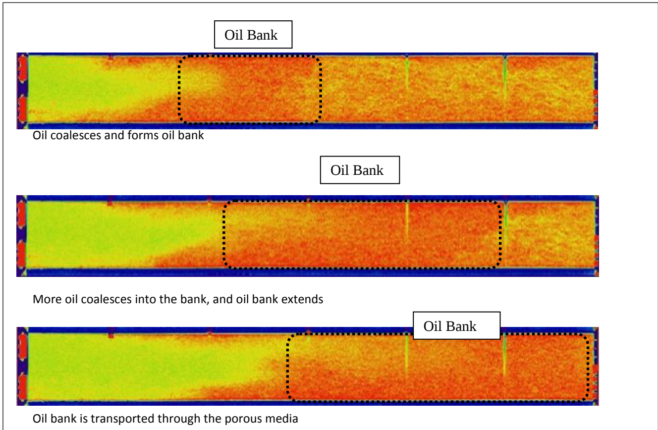
Figure 4.9: Oil Bank build up process in the core (Core Length is 38 cm, core diameter is 3.8 cm). Horizontal cross-sections from the X-ray CT data at the middle of the core. The injected volume increases from top to bottom. Red colour indicates larger oil volume fractions and green indicates the absence of oil.
