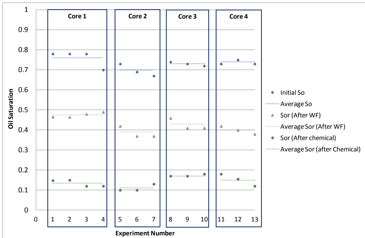
Figure 3.16: Oil Saturation profiles
