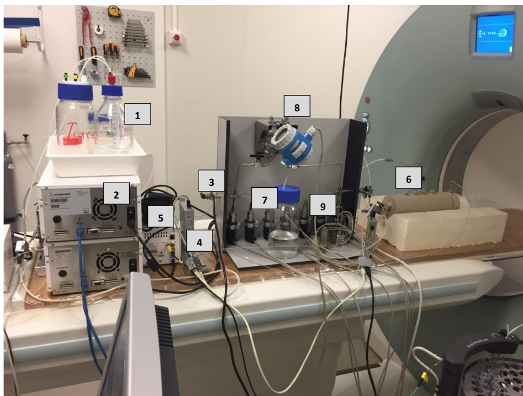
Figure 3.8: the coreflow setup under the CT scanner
