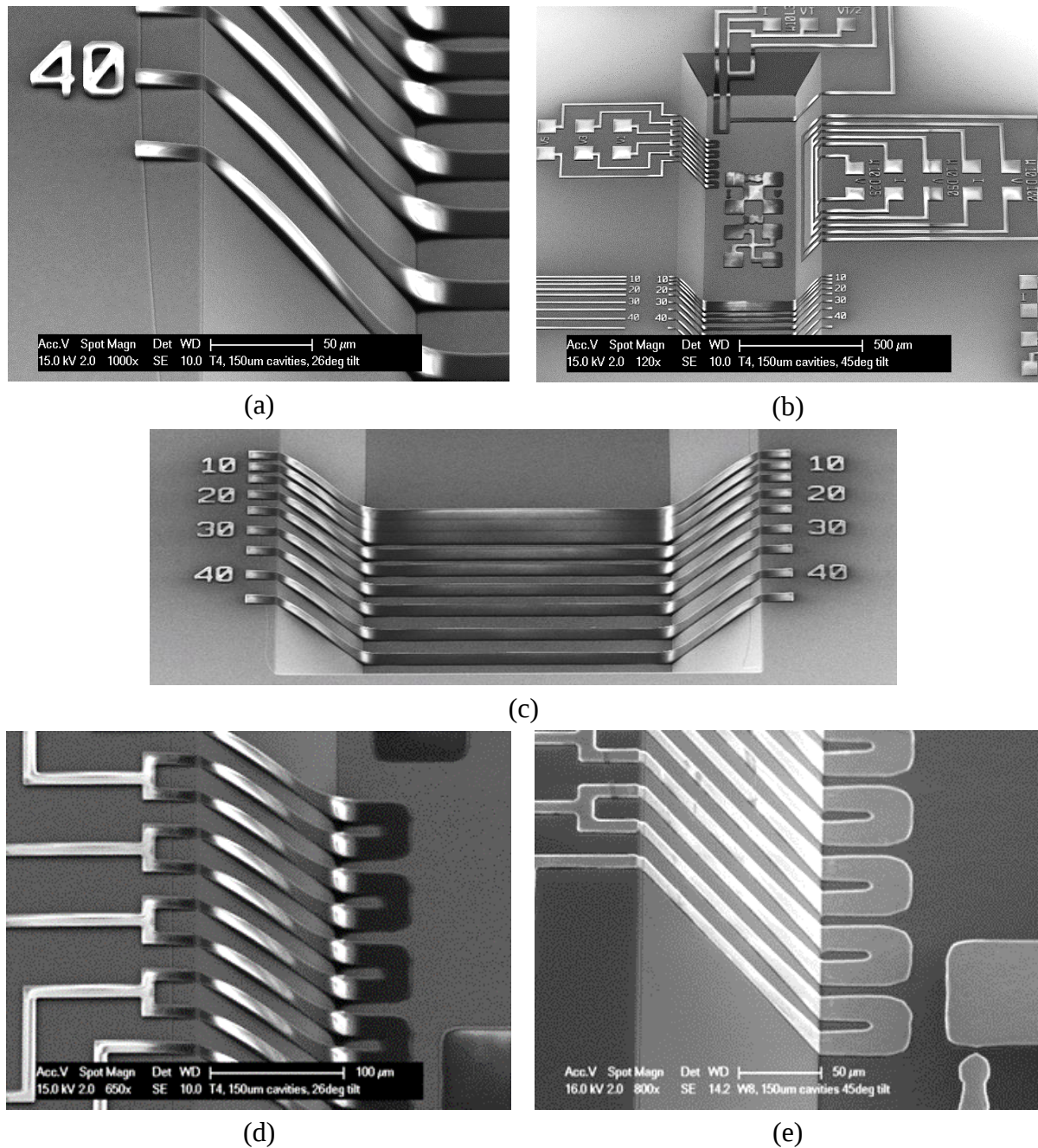
Figure 6-10: The SEM images showing (a) resist coverage over 150 \mu\text{m} cavity coated with spray coating, (b) different structures of 10 \mu\text{m} lines over 150 \mu\text{m} cavity, (c) lines with various gaps from 10 to 40 \mu\text{m} (it can be observed that the lines with 20 \mu\text{m} pitch are merged), (d) 10 \mu\text{m} width / 30 \mu\text{m} pitch wire traces on resist film, and (e) the same feature after etching in aluminum layer.
