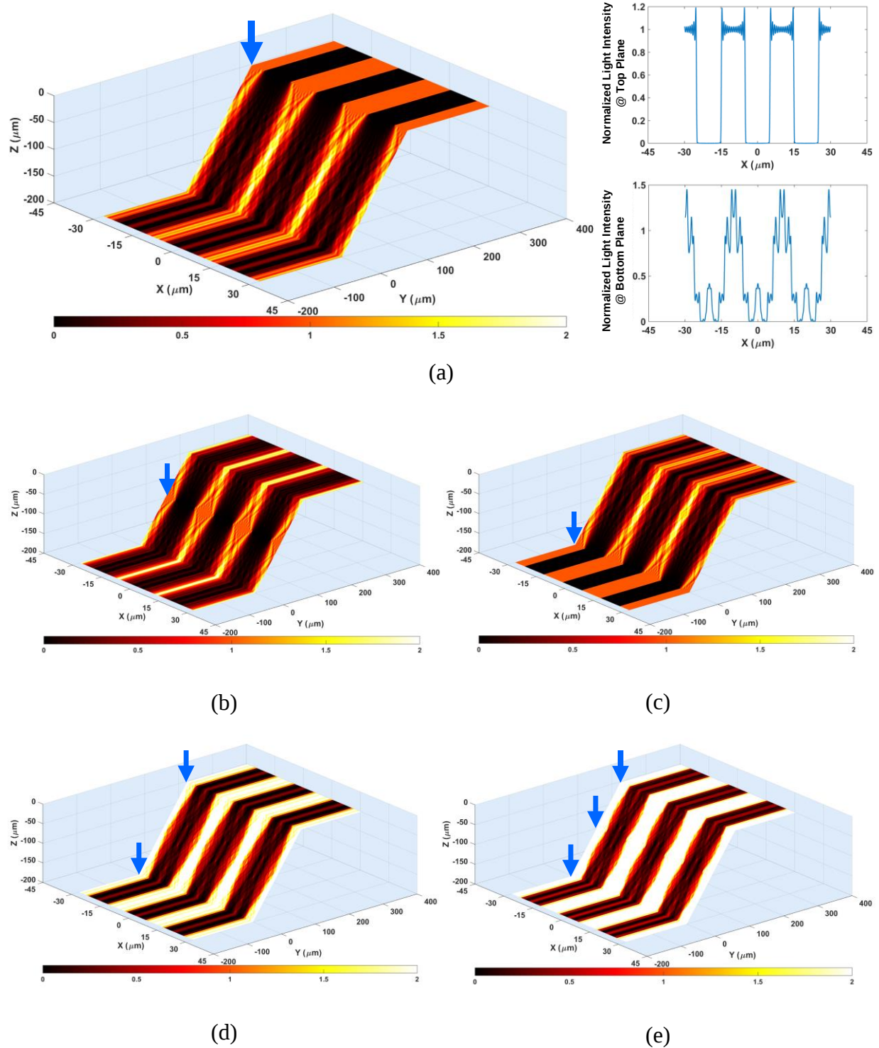
Figure 6-14: Light intensity simulated plots over 200 \mu\text{m} cavity for mask of lines with 10 \mu\text{m} width/20 \mu\text{m} pitch for, (a) one step exposure focusing at top, (b) focusing at mid-level of sidewall, (c) focusing at bottom, (d) double exposure focusing at both top and bottom, and (e) triple exposure focusing at top, bottom and, mid-level of sidewall. The arrows point to the focal plane positions. In multi-exposure parts, light intensity of more than 2 is clipped and saturated. The light intensity amount is scaled to its nominal value (dose to clear).
