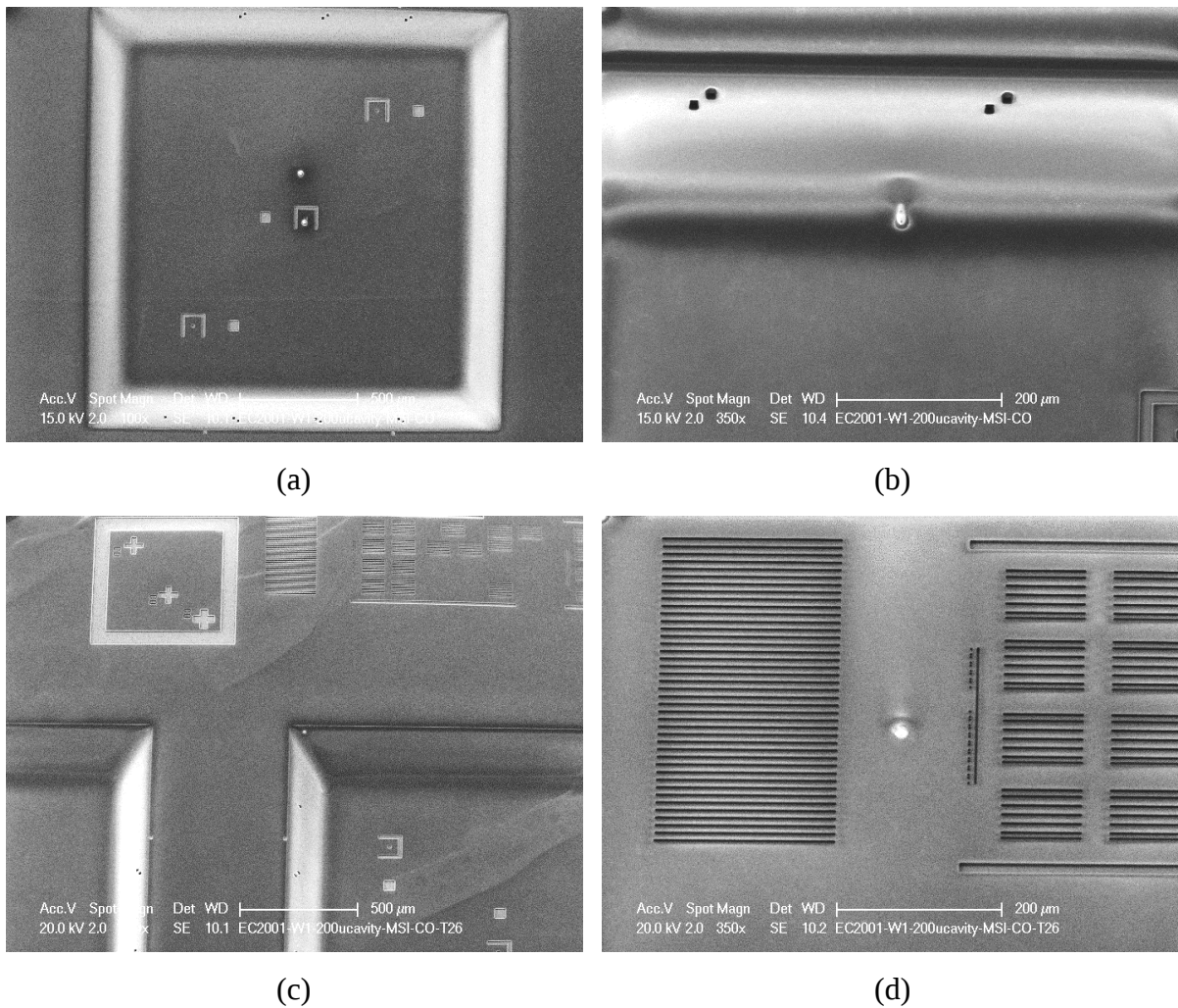
Figure 7-12: SEM images of CO resist patterns formed on top, bottom and sidewalls of 200 \mu\text{m} cavities, from top view: (a) a cavity with open windows on the bottom and sidewalls, (b) magnified image of windows on the cavity sidewall, with 26 degree tilted view: (c) patterns on 3 surfaces, and (d) CO windows with small features on top with good resist adhesion.
