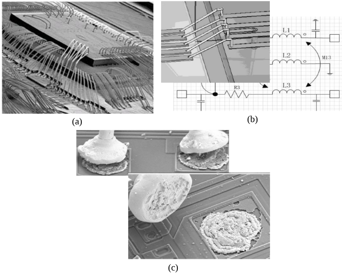
Figure 6-2: Examples of wire bonding interconnect challenges: (a) complexity [12], (b) crosstalk [13], and (c) reliability [14].
