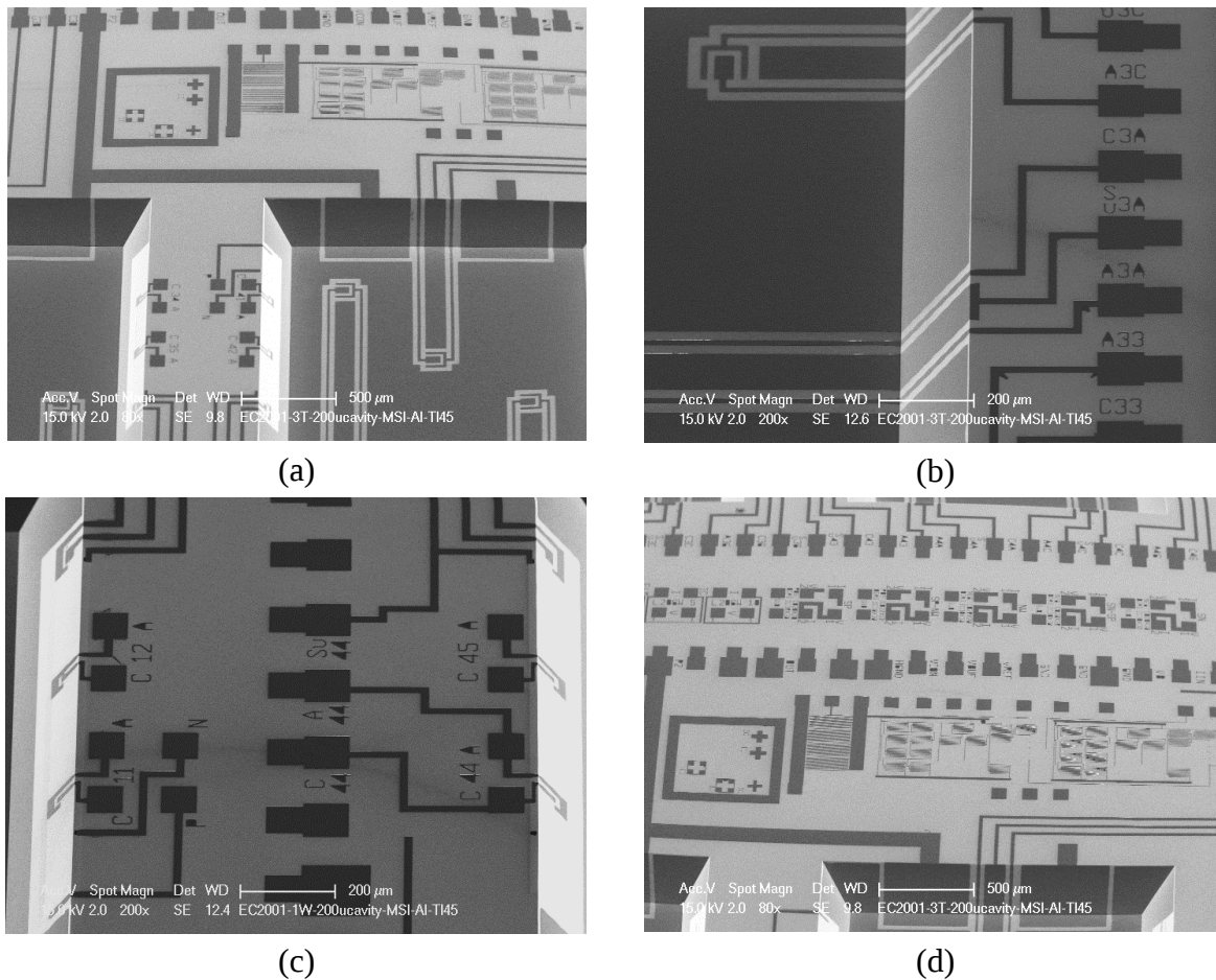
Figure 7-14: SEM images of first aluminum traces formed on top, bottom and sidewall of 200 \mu\text{m} cavities, with 45° tilted view: (a) a cavity with wires to sensors at the bottom and sidewall and LED chip connection wires (b) connections to the bottom temperature sensors, (c) connections to the sidewall light sensors, and (d) control circuits and pads on the top plane.
