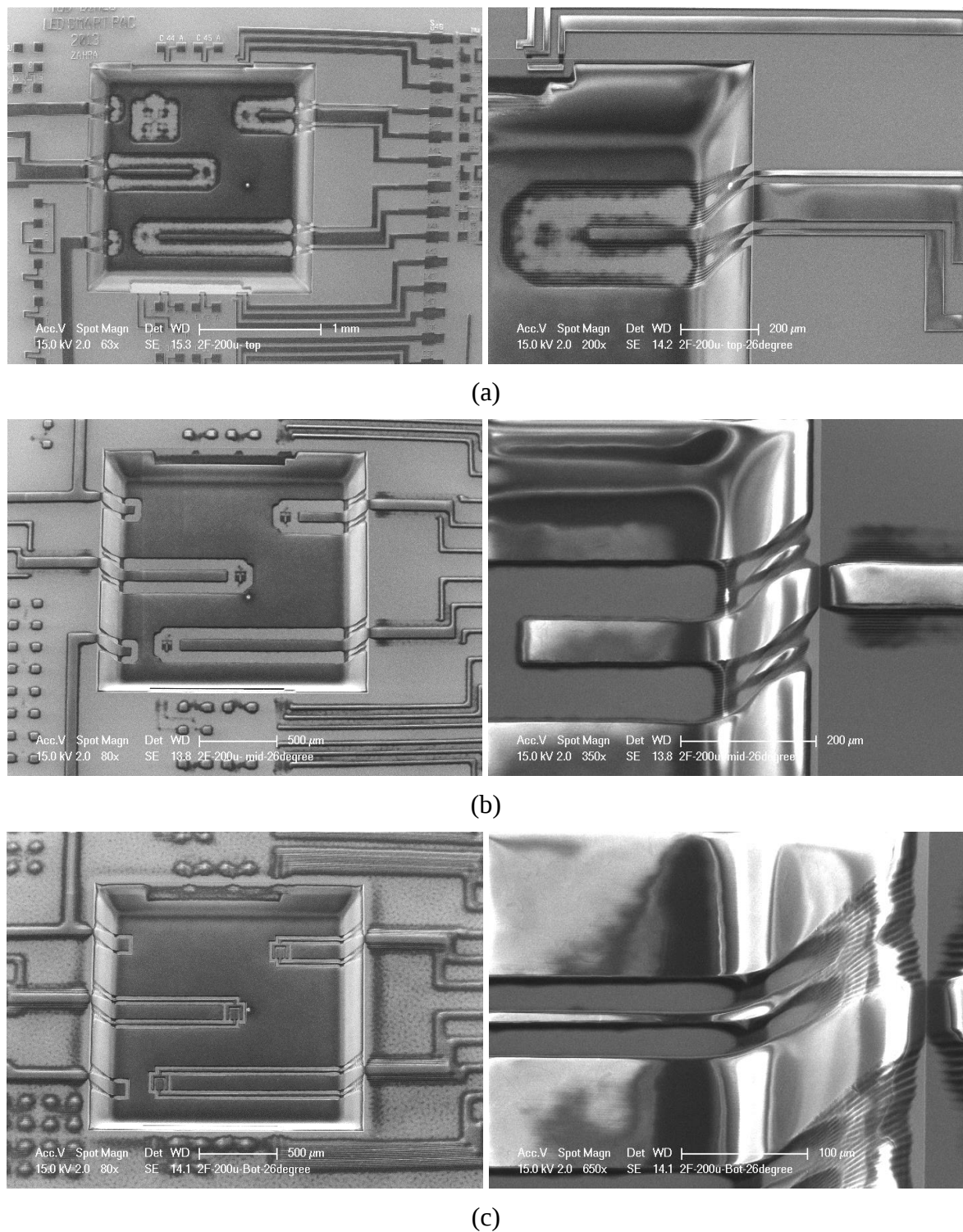
Figure 6-17: The SEM images of MSI experiments with focusing at (a) top plane, (b) mid plane (100 μm), and (c) bottom plane (200 μm).
