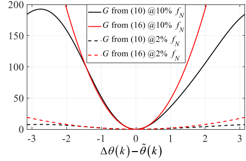
Fig. 4. Waveforms of G(k) with \tilde{\theta}(k) being \pi/2 rad at 1/10 and 1/50 of the rated speed, where f_N is the rated motor rotating frequency.
