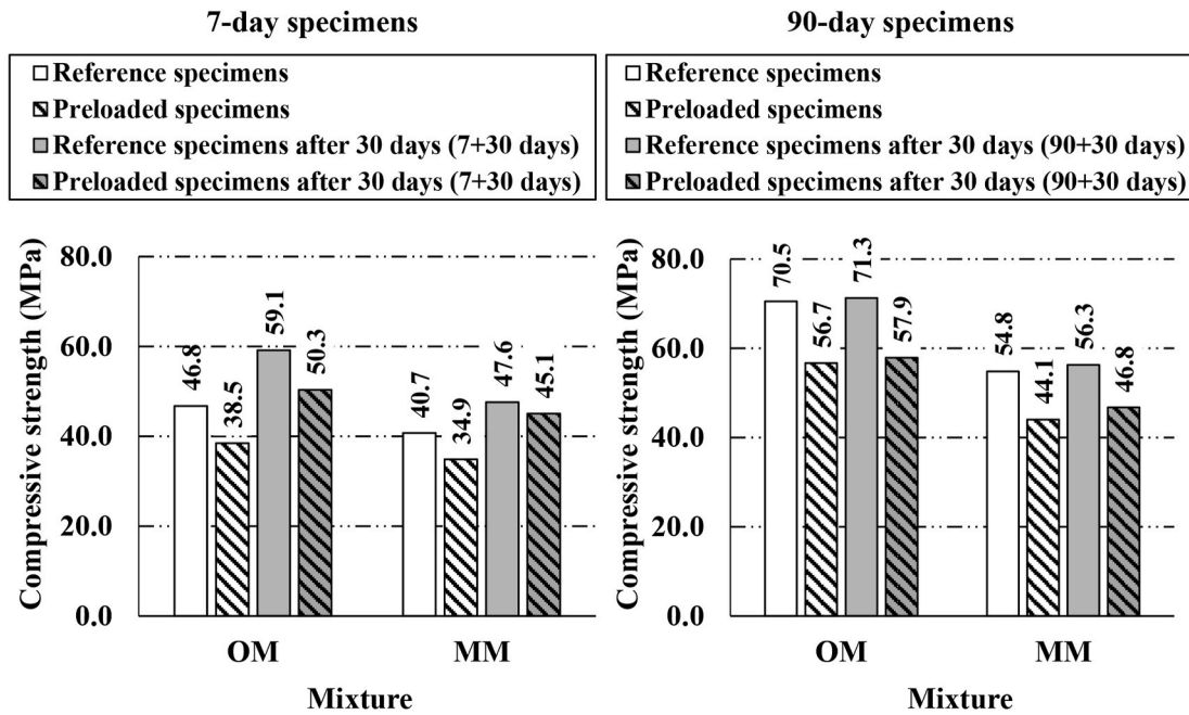
Fig. 14. The compressive strength test results.
