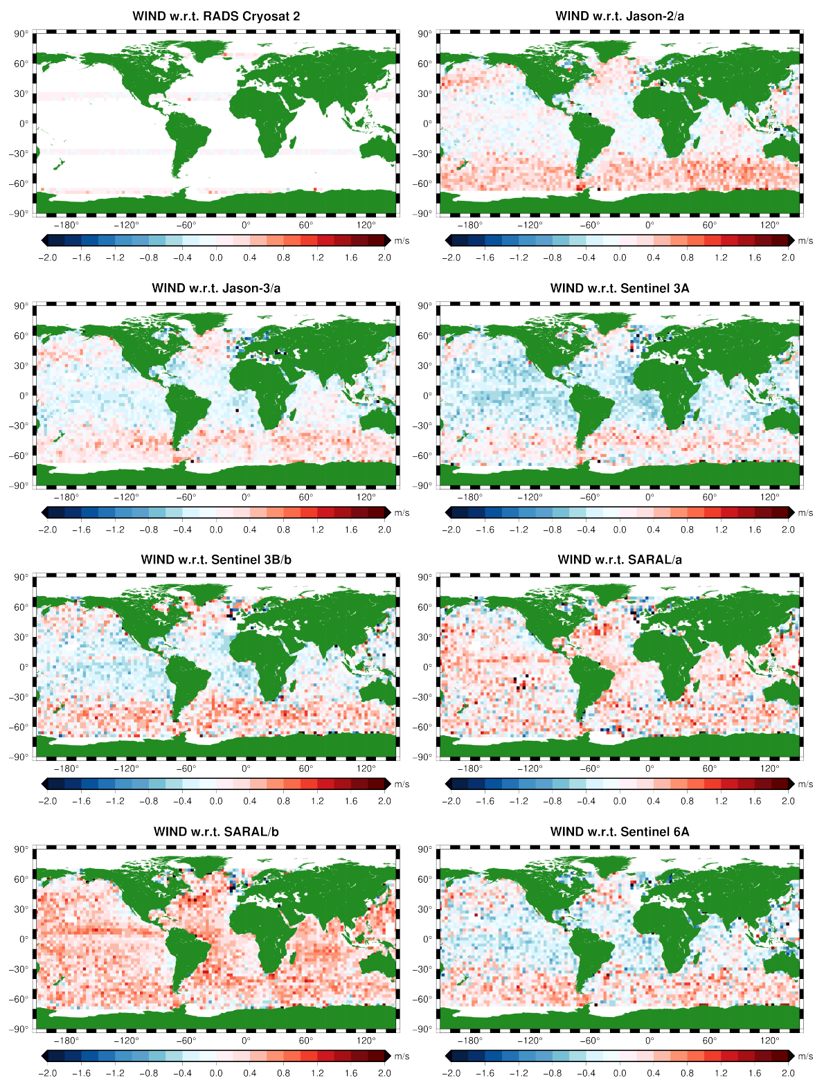
Figure 8. Mean wind speed crossover differences between GOP CryoSat-2 and the concurrent altimetry missions RADS CryoSat-2, Jason-2, Jason-3, Sentinel-3A, Sentinel-3B, SARAL, and Sentinel-6A.
