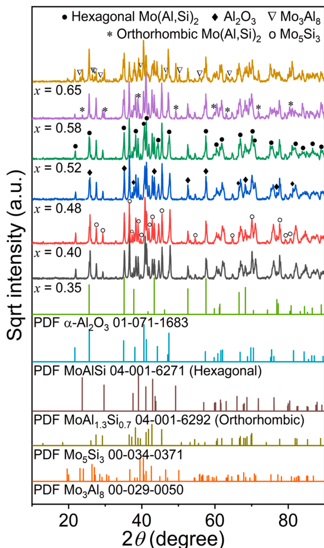
Fig. 7. XRD patterns of \text{Mo}(\text{Al}_x\text{Si}_{1-x})_2 after 16 hours oxidation in low p\text{O}_2 ( 10^{-14} atm.) gaseous ambient at 1373 K recorded with Bragg–Brentano geometry.
