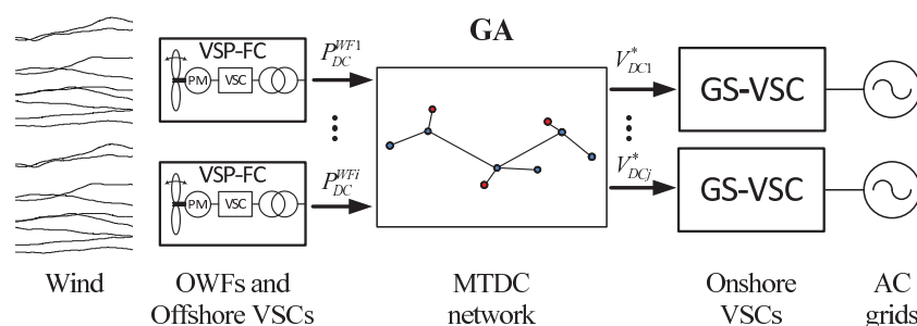
Figure 10. How information flows in the distributed voltage control method.
