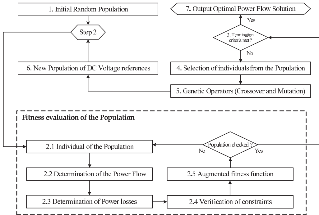
Figure 8. Flowchart of the Genetic Algorithm implemented to solve the load flow of the MTDC grid.
