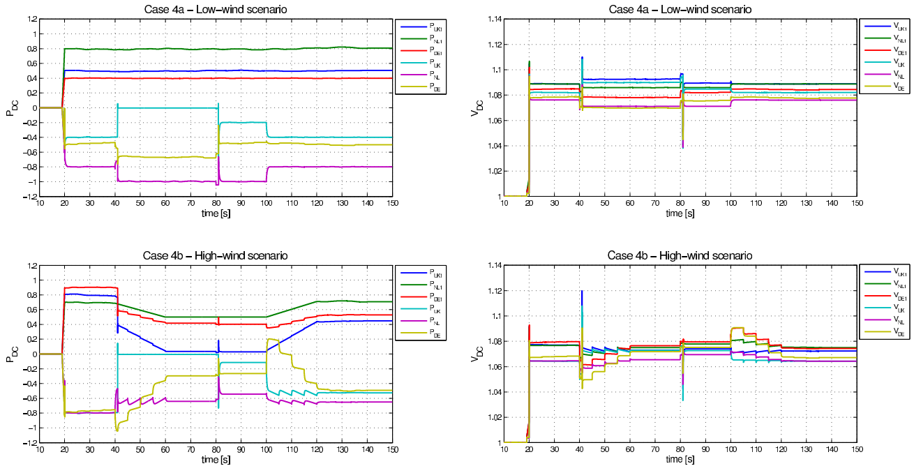
Figure 14. Results from Case Study 4: AC fault in the UK node.
