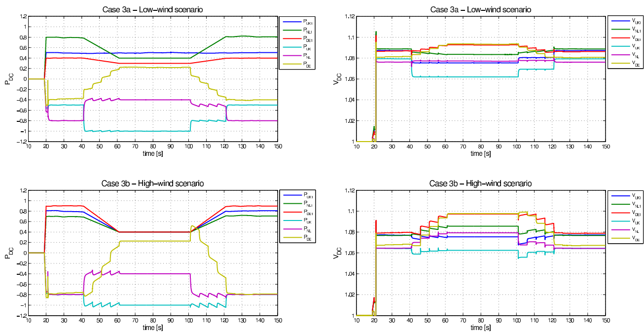
Figure 13. Results from Case Study 3: Wind Curtailment.
