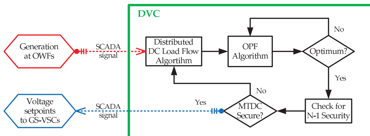
Figure 7. Flow chart of the distributed voltage control method.
