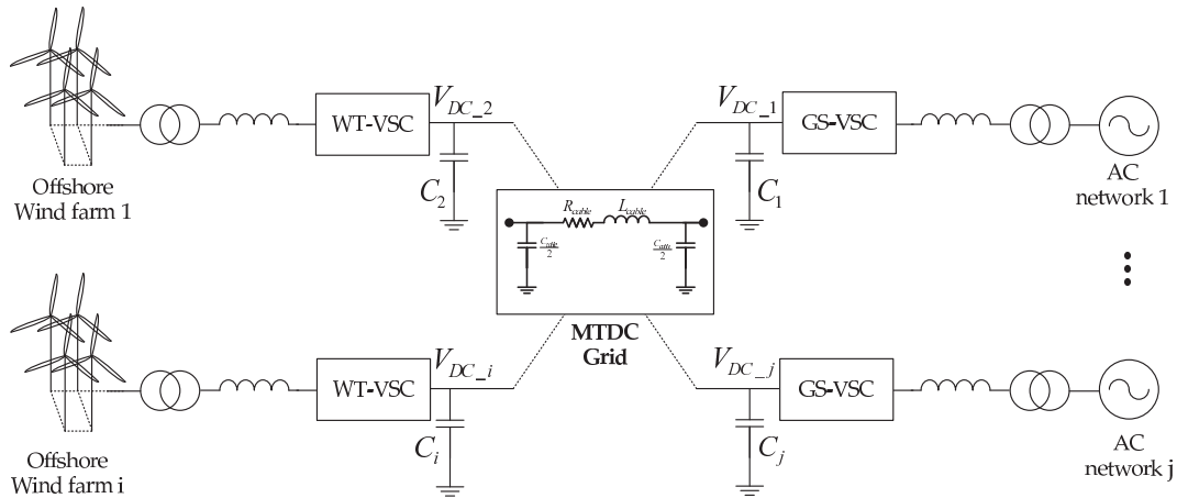
Figure 6. Generic representation of a MTDC grid.
