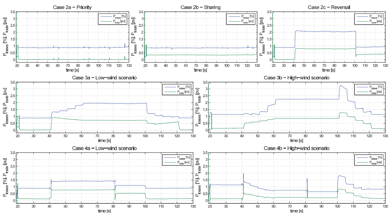
Figure 15. Transmission losses in the MTDC system in percentage of the total generated power and power traded in the MTDC system in per unit of the system power base.
