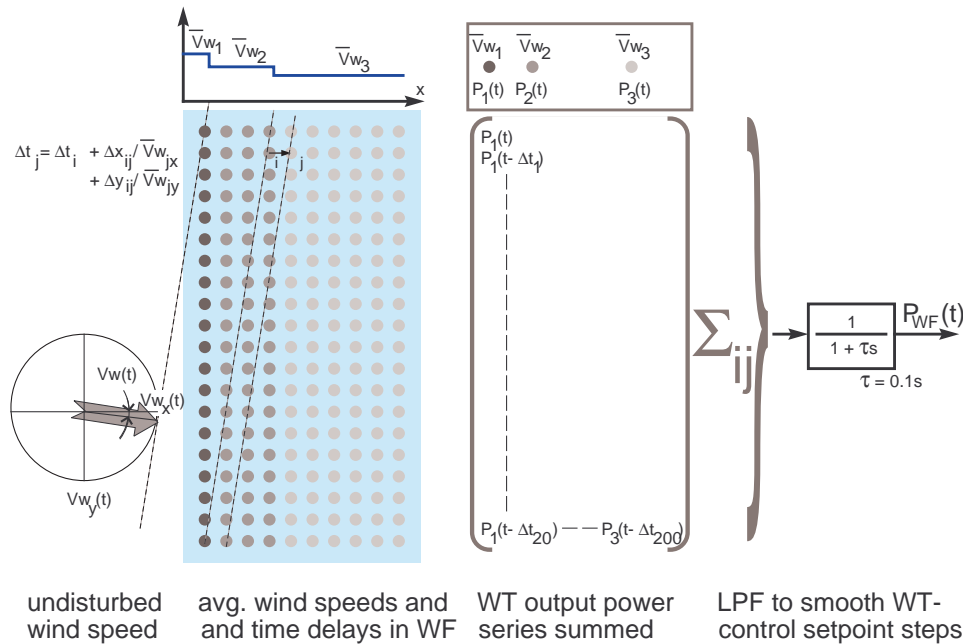
Figure 3. Synthesized wind farm output power.
