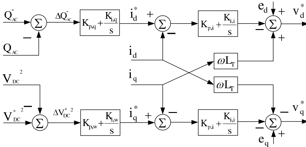
Figure 5. Grid-side VSC-HVDC control diagram with outer controllers.
