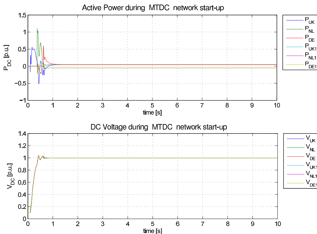
Figure 11. Results from Case Study 1: MTDC Start-up.
