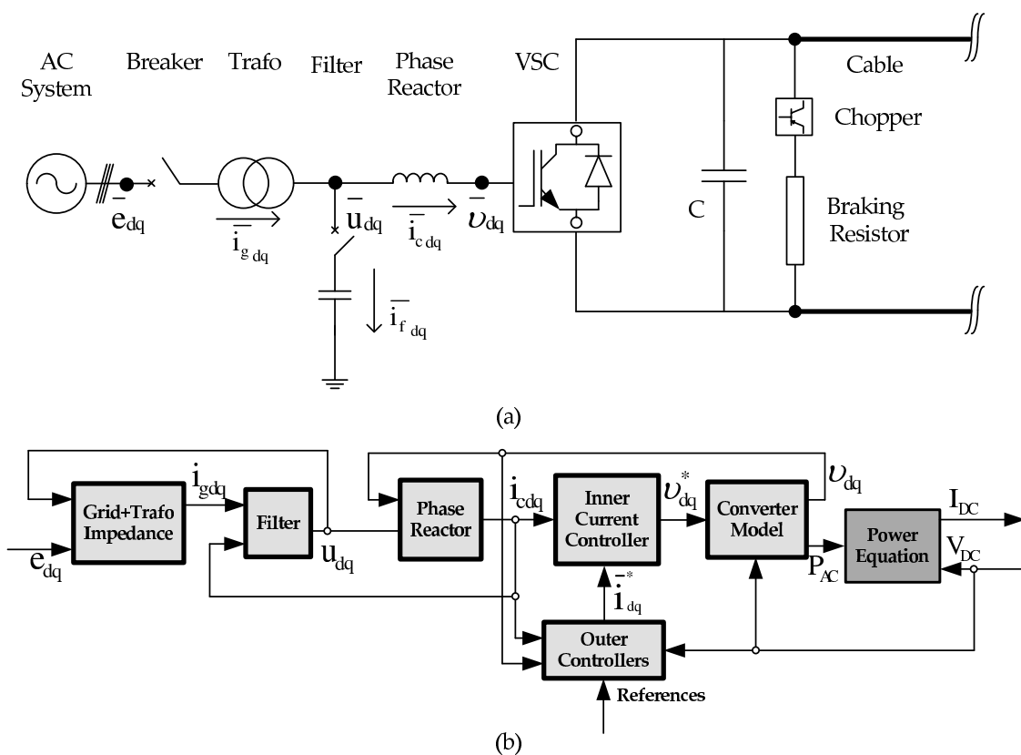
Figure 4. (a) Single-line diagram of the VSC-HVDC model; (b) Signal flow inside the model.
