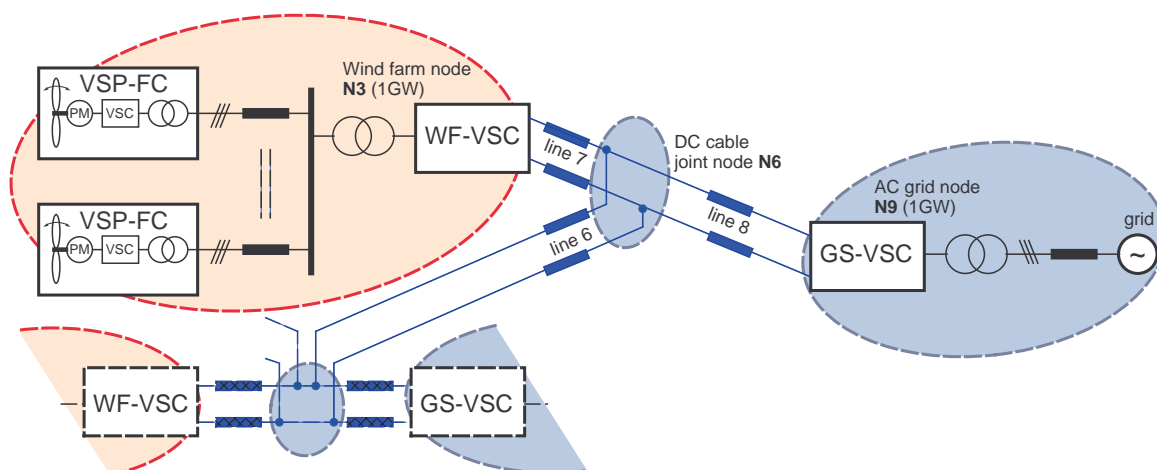
Figure 2. Components of the modeled MTDC grid (DE nodes).
