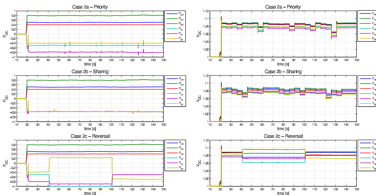
Figure 12. Results from Case Study 2: Normal Operation.
