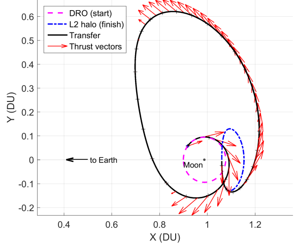
Figure 4. A 1-revolution transfer, using 0.4 N max thrust (for an initial mass of 1500 kg), viewed in the synodic reference frame. The spacecraft begins in the DRO and ends in the L 2 halo orbit. Tick marks appear at \frac{1}{2} day intervals, and thrust vectors appear at \frac{1}{4} day intervals.
