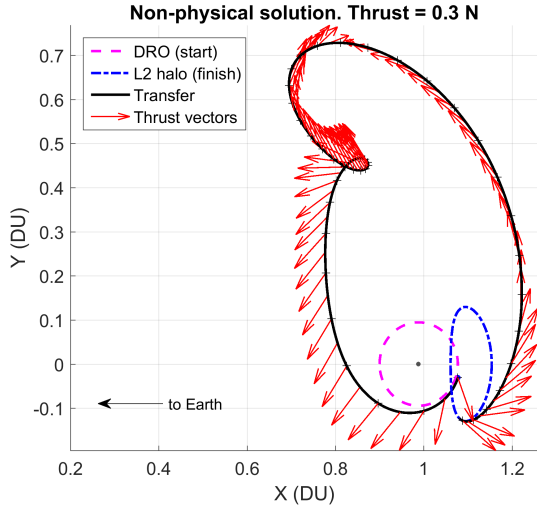
Figure 13. A non-physical solution illustrating a common failure mode for the continuation method described. The loop which appears near x=0.8 , y=0.45 came in for many cases in which the optimizer could not converge.
