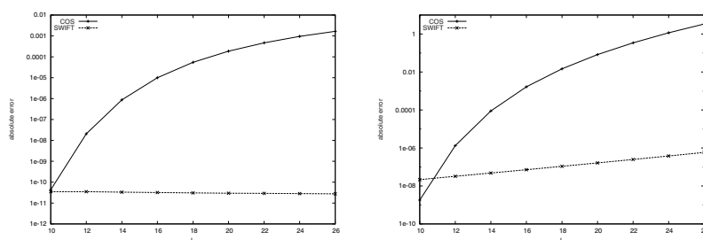
FIG. 5. Absolute errors corresponding to the valuation of a cash-or-nothing call (left) and a European call (right) under the GBM dynamics by means of the SWIFT ( m = 3 ) and COS ( N = 40 ) methods with parameters S_0 = K = 100, r = 0.1, T = 1, \sigma = 0.25 . The reference values have been computed using the Black-Scholes formulae: 0.5504504967481910 (cash-or-nothing) and 14.9757907783113000 (call).
