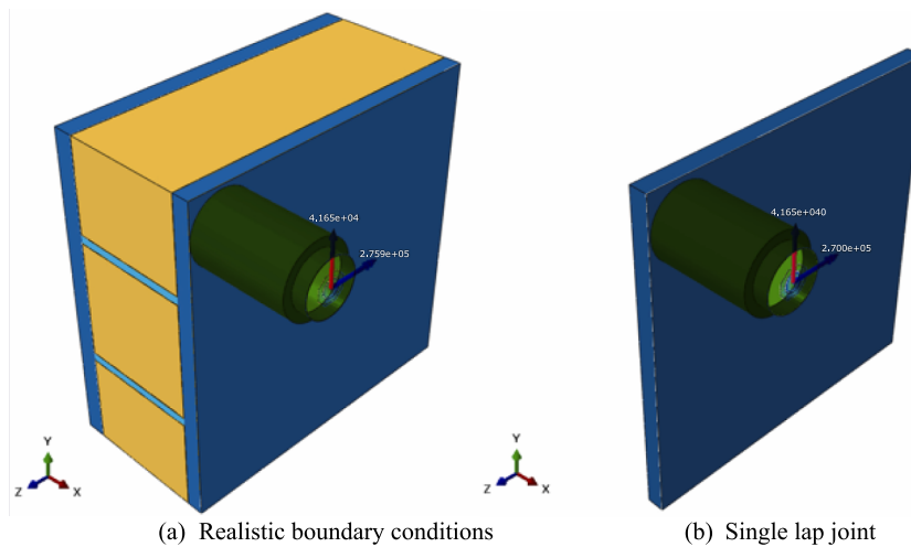
Fig. 25. Influence of boundary conditions on the amount of bending moment at 50 kN, values in N and mm.
