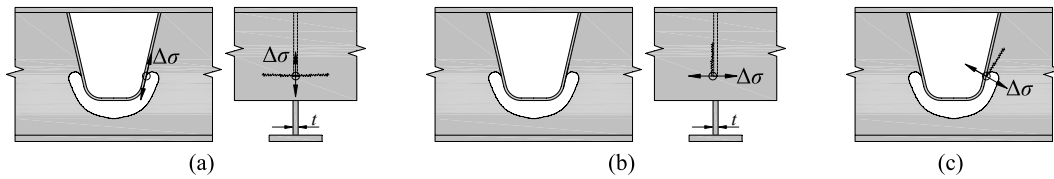
Fig. 22. Fatigue crack at rib-to-crossbeam welded joint: (a) longitudinal crack on U-rib; (b) vertical crack on U-rib; (c) crack on crossbeam.
