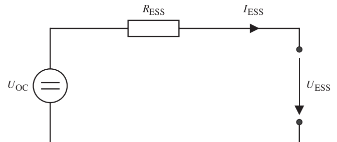
Fig. 3. Equivalent electrical circuit for the Li-ion battery-based energy storage system.
