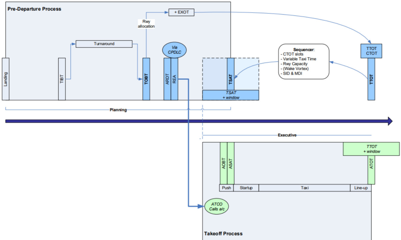
Fig. 1. Schematic diagram of departure manager process overview. The flow contains two distinct phases: the pre-departure phase and the executive phase. (LVNL, 2019)
