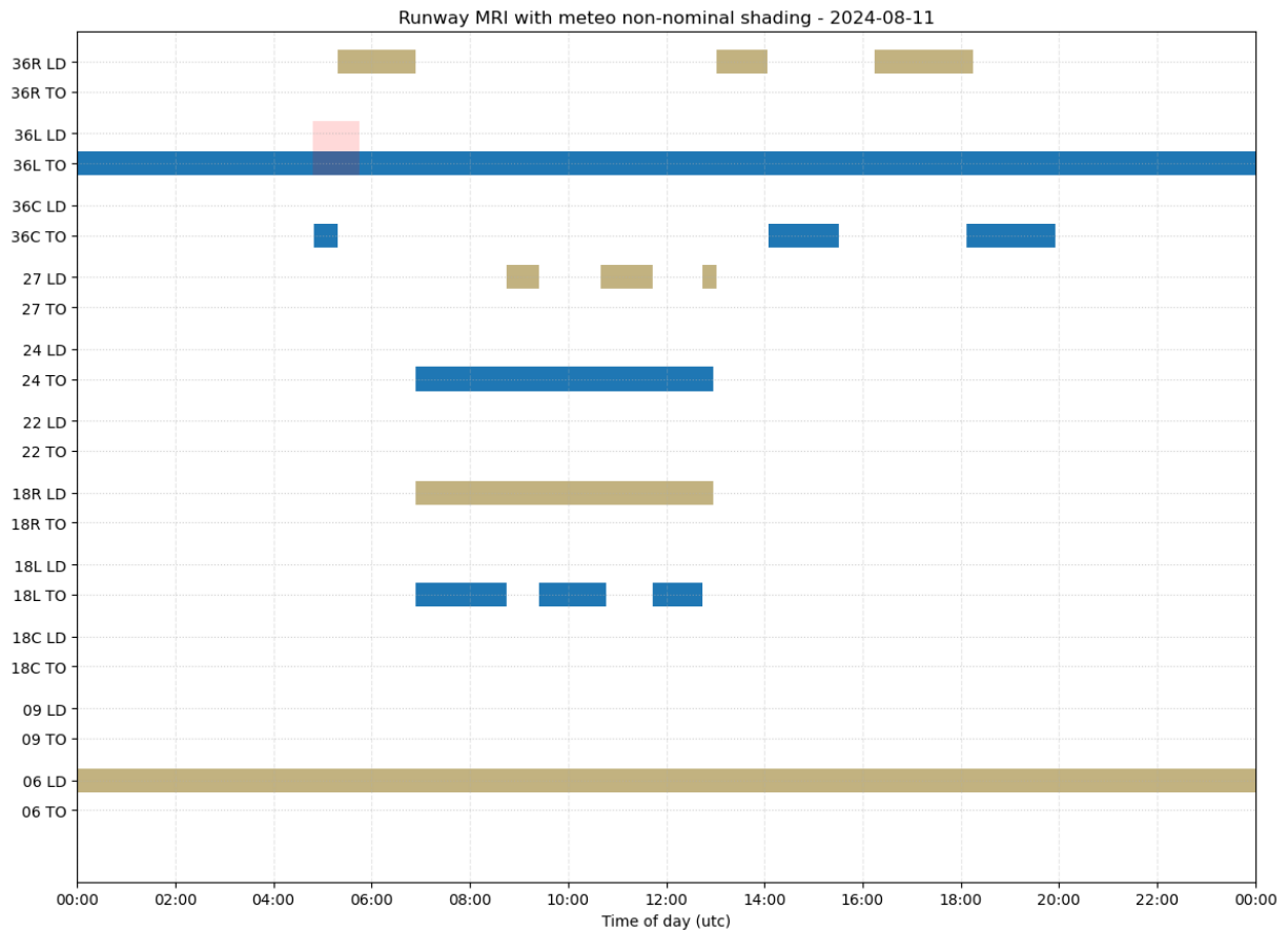
Figure 3.1: Runway operational timeline for August 11, 2024, showing runway opening times per operation type (LD = Landing, TO = Takeoff) with red shading indicating periods exceeding nominal meteorological conditions. Blue bars indicate takeoff operations, sand-colored bars indicate landing operations, and red shading marks the brief morning period when crosswind limits were exceeded.
