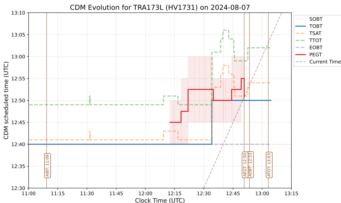
Figure 2.1: Evolution of CDM and PEGT times during the turnaround of TRA173L (HV1731) on 7 August 2024 at Amsterdam Airport Schiphol.
