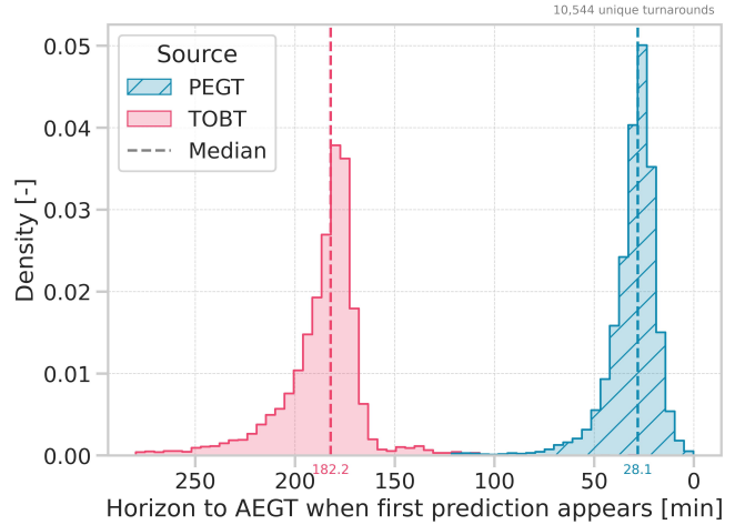
Fig. 3. First availability of TOBT and PEGT relative to AEGT for August 2024 at Amsterdam Airport Schiphol.
