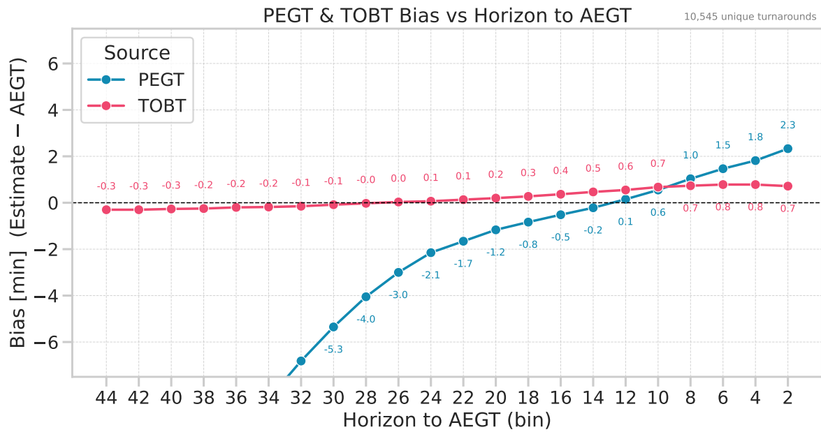
Figure 2.4: Bias in prediction error of PEGT and TOBT relative to AEGT for August 2024 at Amsterdam Airport Schiphol.
