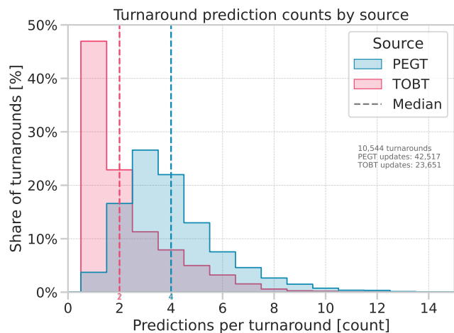
Figure 2.6: Distribution of the number of predictions per turnaround by source (TOBT vs PEGT) for August 2024 at Amsterdam Airport Schiphol.
