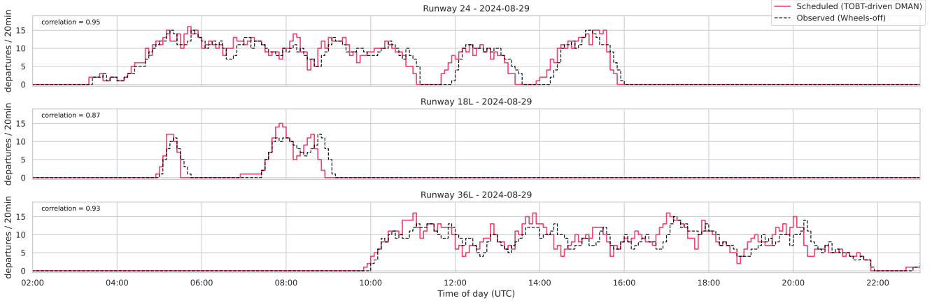
Fig. 6. Comparison of reconstructed DMAN schedule and observed departure throughput per runway on 29 August 2024. Throughput is evaluated using a trailing 20-minute window sampled every 5 minutes. Pearson correlation coefficients per runway are annotated in each subplot.
