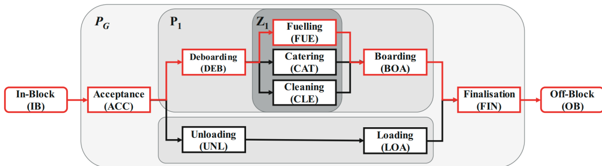
Figure 5.2: Overview of aircraft turnaround processes showing typical sequential and parallel service activities. The critical path (highlighted in red) represents the sequence of time-critical activities that determine the minimum possible turnaround duration. Many parallel processes are omitted for clarity. Adapted from Asadi et al. (2020)
