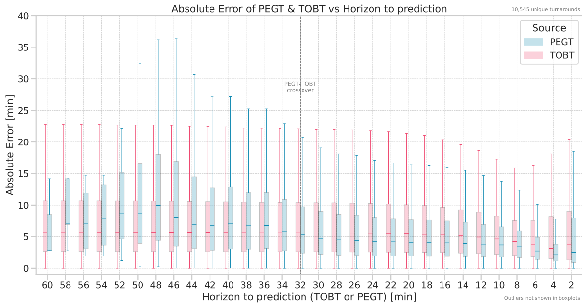
Figure 2.5: Absolute prediction error of PEGT and TOBT relative to their own prediction times for August 2024 at Amsterdam Airport Schiphol.
