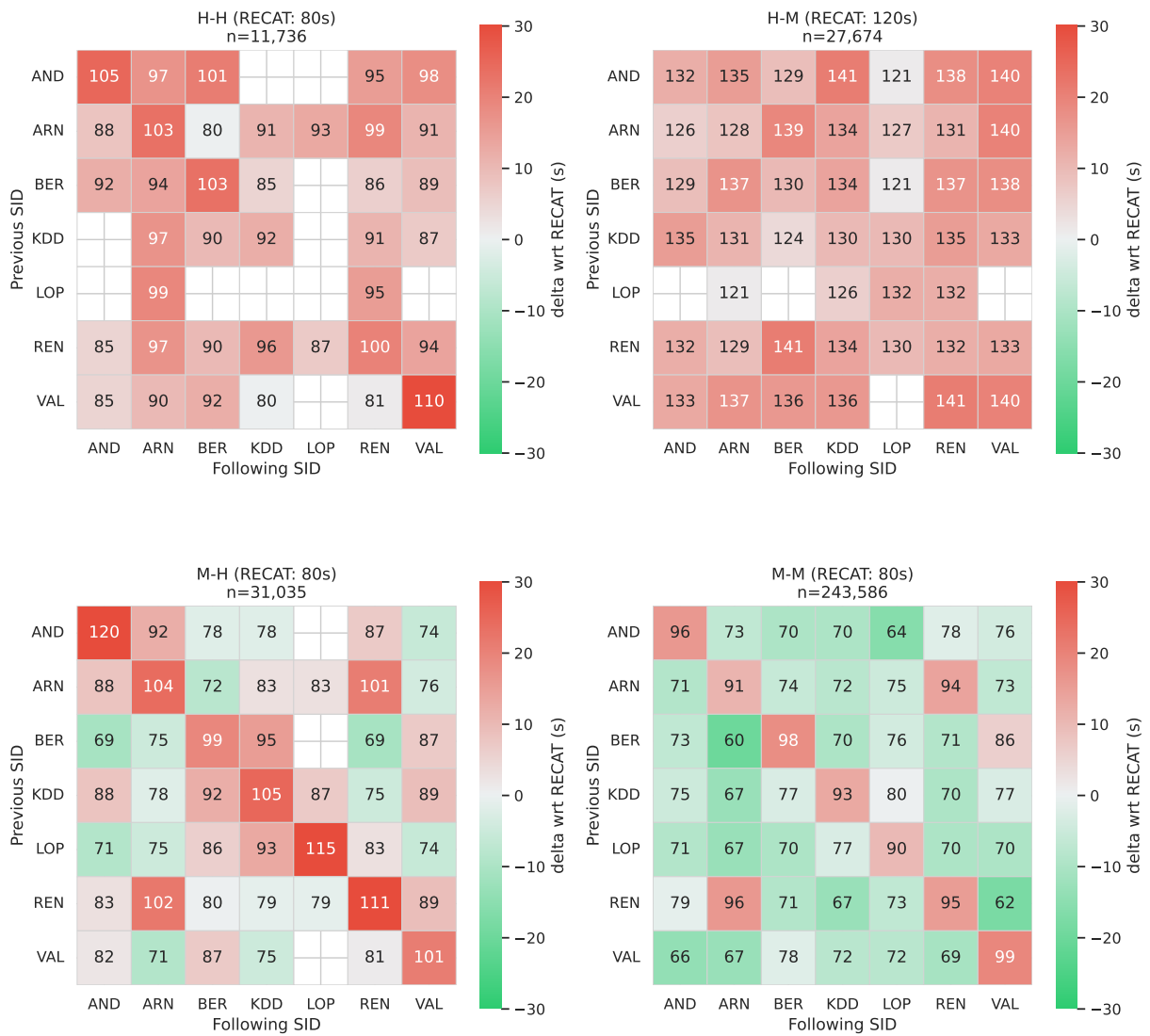
Figure 4.2: Runway 18L: observed SID-pair separation versus RECAT-EU for the most common WTC pairs. Cell values show modal separations (s); colors show \Delta vs RECAT-EU.
