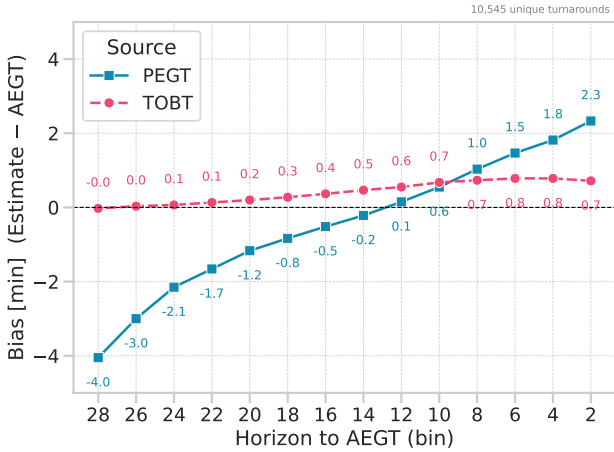
Fig. 5. Bias of TOBT and PEGT relative to AEGT for August 2024 at Amsterdam Airport Schiphol.
