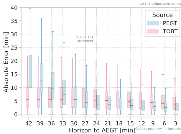
Fig. 2. Absolute prediction error of PEGT and TOBT relative to AEGT for August 2024 at Amsterdam Airport Schiphol.
