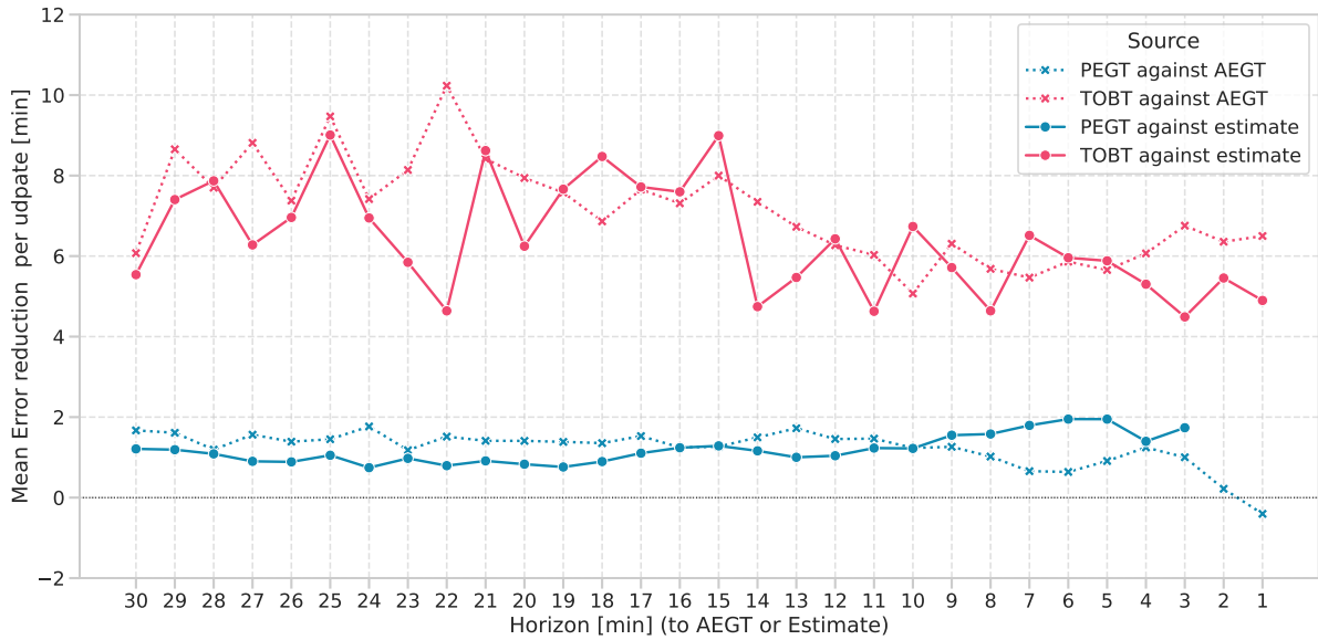
Figure 2.8: Mean reduction in absolute prediction error of PEGT and TOBT updates relative to AEGT and their own prediction times for August 2024 at Amsterdam Airport Schiphol.
