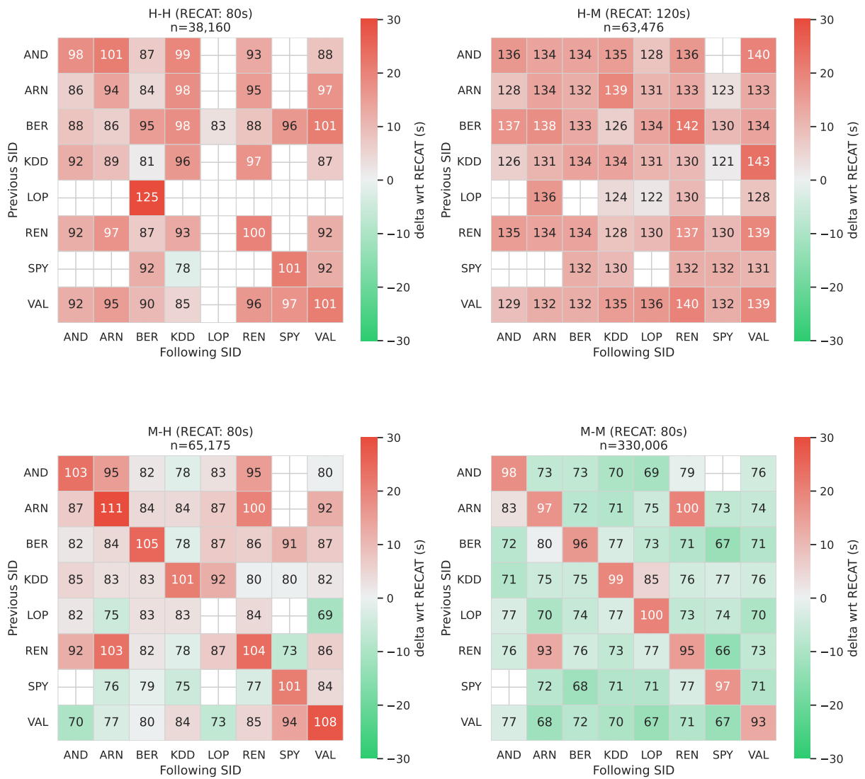
Figure 4.1: Runway 24: observed SID-pair separation versus RECAT-EU for the most common WTC pairs. Cell values show modal separations (s); colors show \Delta vs RECAT-EU.
