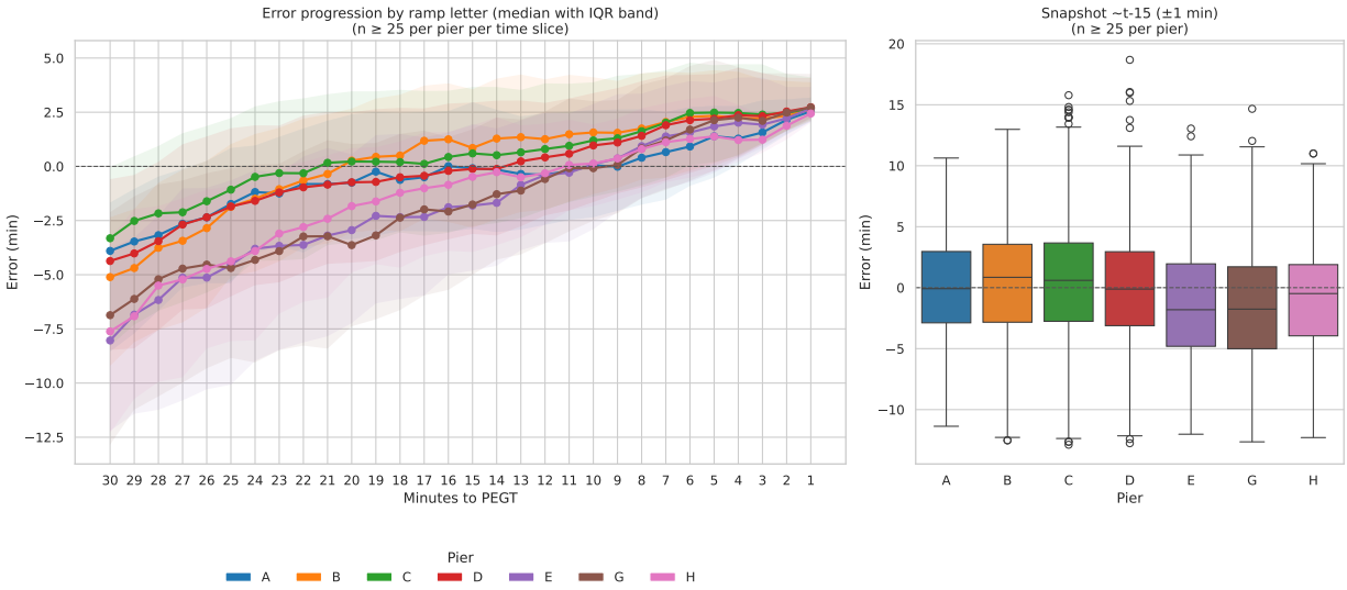
Figure 2.11: Progression of signed PEGT error by pier as a function of time-to-departure. Distinct pier-level patterns are visible, including differences in bias transition timing and dispersion, suggesting that error dynamics depend on operational context.
