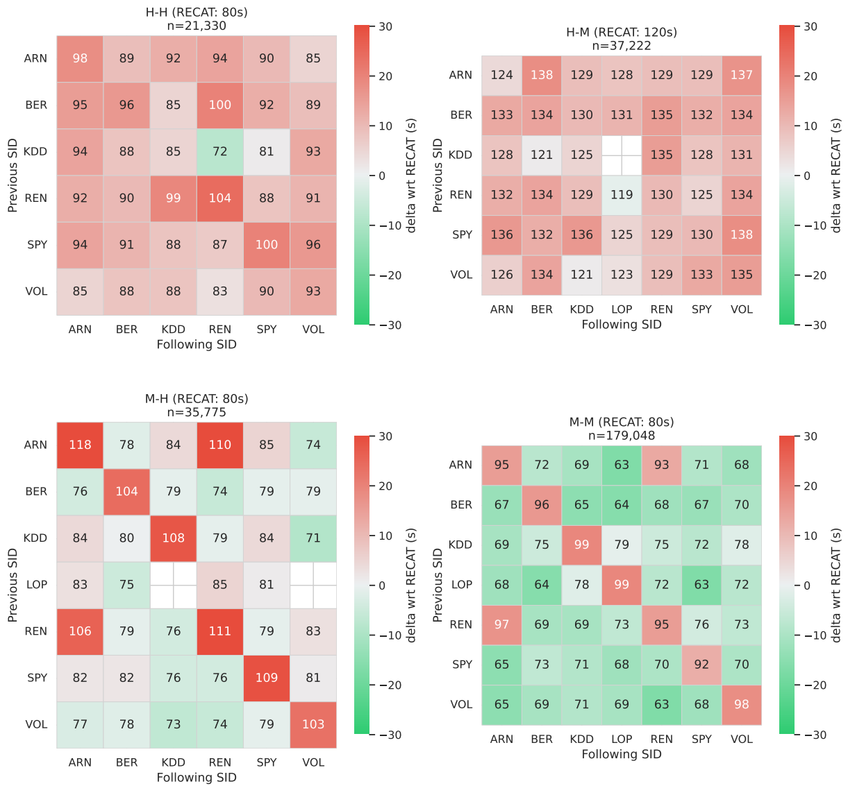
Figure 4.3: Runway 36L: observed SID-pair separation versus RECAT-EU for the most common WTC pairs. Cell values show modal separations (s); colors show \Delta vs RECAT-EU.
