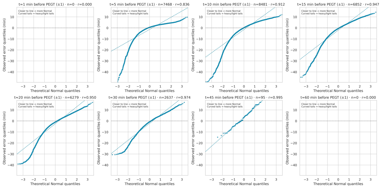
Figure 2.10: Q–Q plots of signed forecast error (PEGT–AEGT) by PEGT-anchored prediction horizon. Short horizons show clear deviations from Normality (skewness and heavy tails), while intermediate horizons exhibit a more linear central region with persistent tail deviations.
