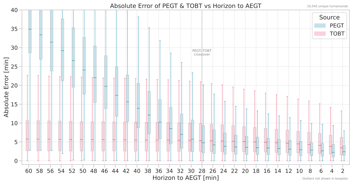
Figure 2.2: Absolute prediction error of PEGT and TOBT relative to AEGT for August 2024 at Amsterdam Airport Schiphol.
