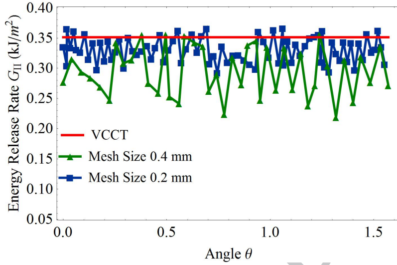
Figure 13: Energy release rate distribution along crack front.
