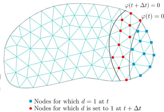
Figure 5: Change of the damage values at the nodes as the front moves.
