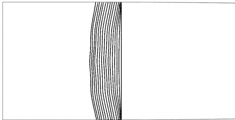
Figure 9: Evolution of crack front under cyclic loading for DCB specimen.
