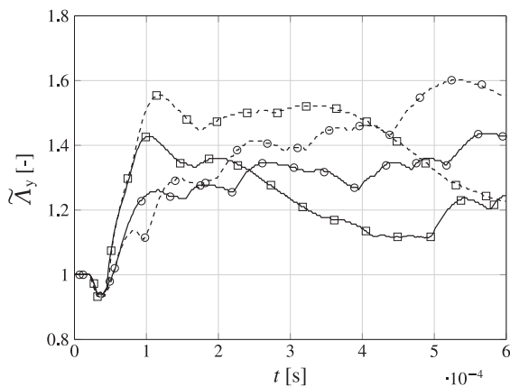
Fig. 16. Comparison of TBD for two- and three-dimensional SBI. —: three-dimensional simulations; .....: two-dimensional simulations; ○: ISBI; □: RSBI.
