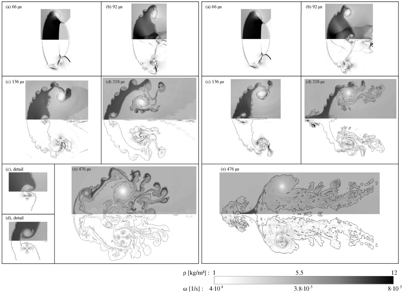
Fig. 15. Bubble evolution of two-dimensional (left) and three-dimensional (right) simulations of ISBI at a shock Mach number of Ma = 2.83 . Isocontours of Y_{Xe} = 0.1 outlines the bubble interface. Density (top) and vorticity magnitude (bottom) show different evolution at five time steps. N_2 -jet is illustrated in the magnified sections in (c), detail and (d), detail.
