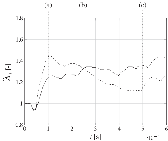
Fig. 12. Normalized transverse bubble diameter for three-dimensional ISBI and RSBI. —: non reacting; .....: reacting.
