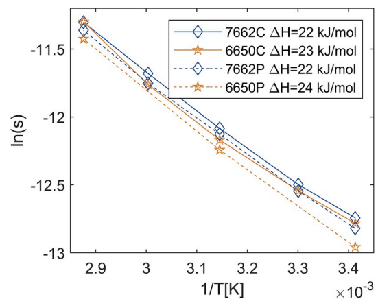
Fig. 11. Evaluation of sorption enthalpy, by using a Van't Hoff plot of the solubility of water vapour at different temperatures; not corrected for phosphor content.
